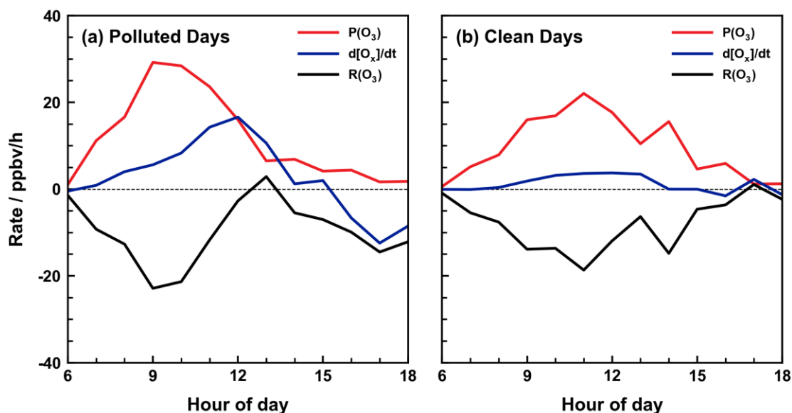
Figure 6. Diurnal variations of daytime P(O_3) , d[Ox]/dt , and R(O_3) during (a) polluted and (b) clean periods. The red line represents the photochemical ozone production rate P(O_3) , the blue line indicates the rate of change of total oxidants d[Ox]/dt , and the black line corresponds to the regional transport rate R(O_3) .
