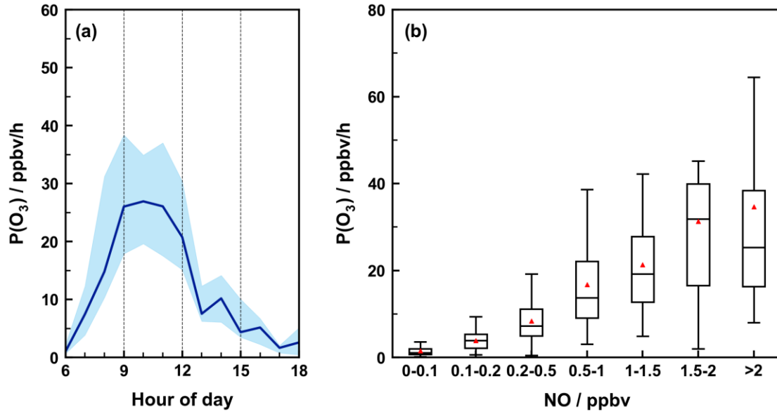
Figure 5. Diurnal variation and NO-dependent distribution of daytime P(O_3) . (a) Average diurnal profile of daytime P(O_3) during the observation period. The dark line denotes the median, and the light blue shading indicates the interquartile range (25th–75th percentile). (b) Box plots of daytime P(O_3) under different NO concentration ranges. The black line inside each box represents the median, and the red triangle marks the mean value within each interval.
