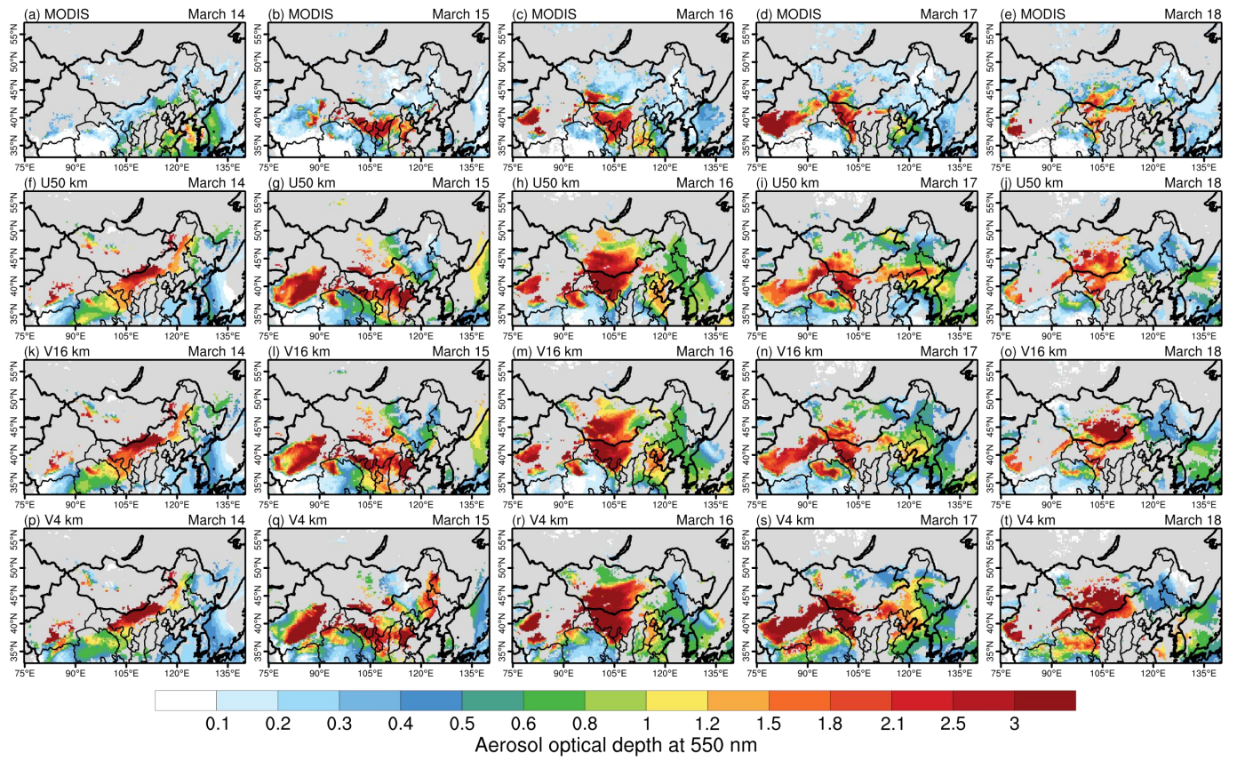
Fig. S6. Daily spatial distributions of MODIS-retrieved and simulated AOD at 550 nm during 14-18 March 2021. For each day, simulated AOD is shown only at grid cells with valid MODIS retrievals to ensure a consistent spatial comparison.
