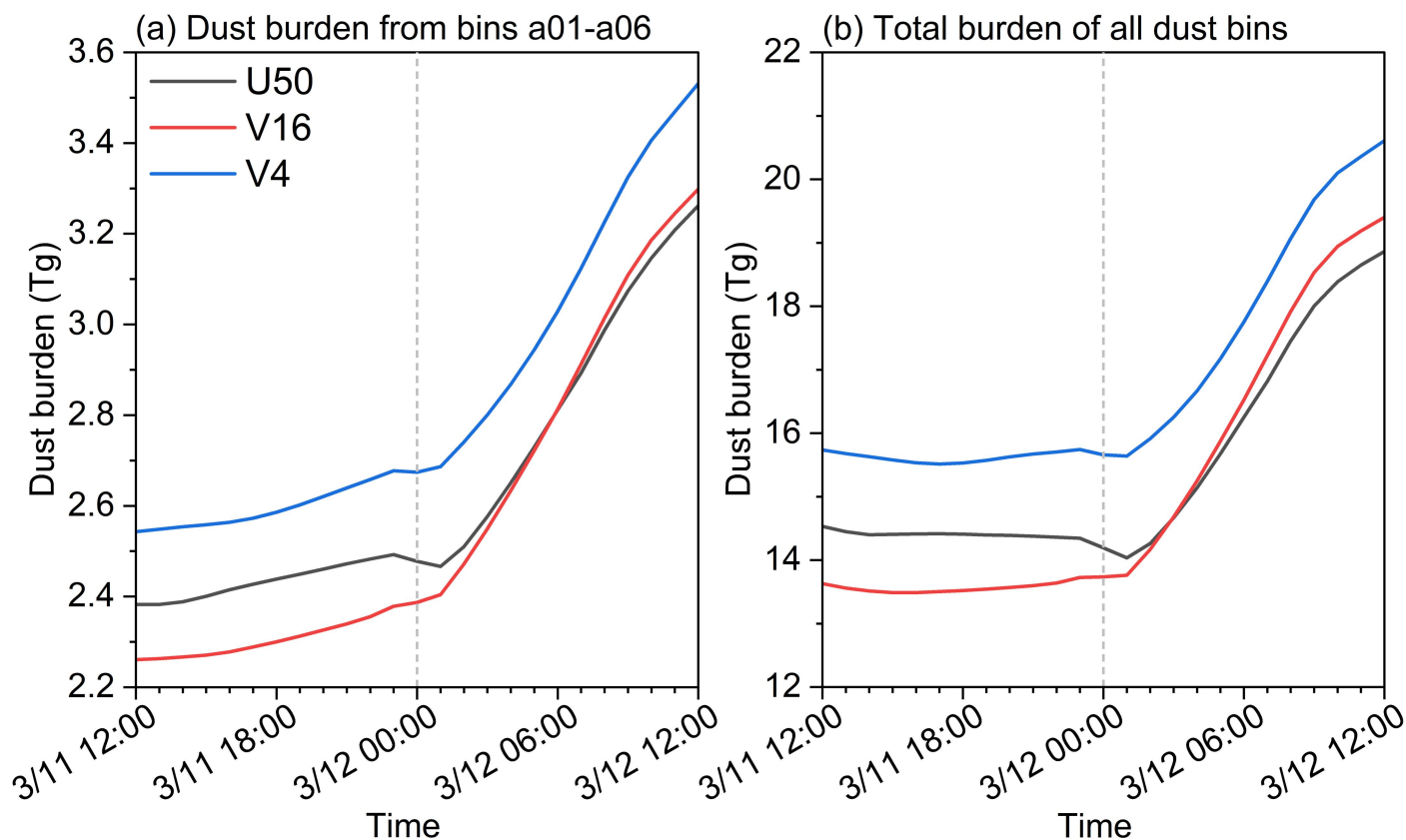
Fig. S1. Temporal evolution of dust burden during the 12 h before and after the meteorological reinitialization at 00:00 on 12 March 2021 for the U50 km, V16 km, and V4 km simulations. (a) Dust burden from bins a01–a06, corresponding to dust size bins 1–6 in Table 1; (b) Total dust burden from all bins a01–a08, corresponding to dust size bins 1–8 in Table 1. The vertical dashed line denotes the meteorological reinitialization time.
