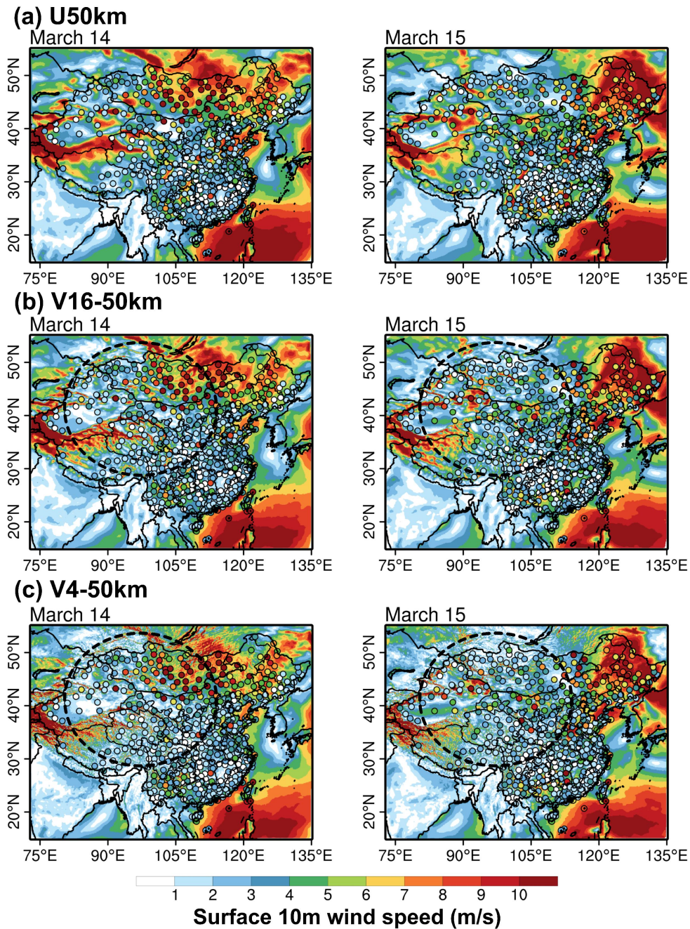
Fig. 4. Spatial distribution of daily mean 10-m wind speed (shading, m s -1 ) from the iAMAS simulations (U50 km, V16 km, and V4 km), with collocated NOAA surface-station observations (453 stations) overlaid as colored markers, during 14-15 March 2021. These two days are selected as representative periods during the development of the dust event. The dashed outline denotes the refinement region.
