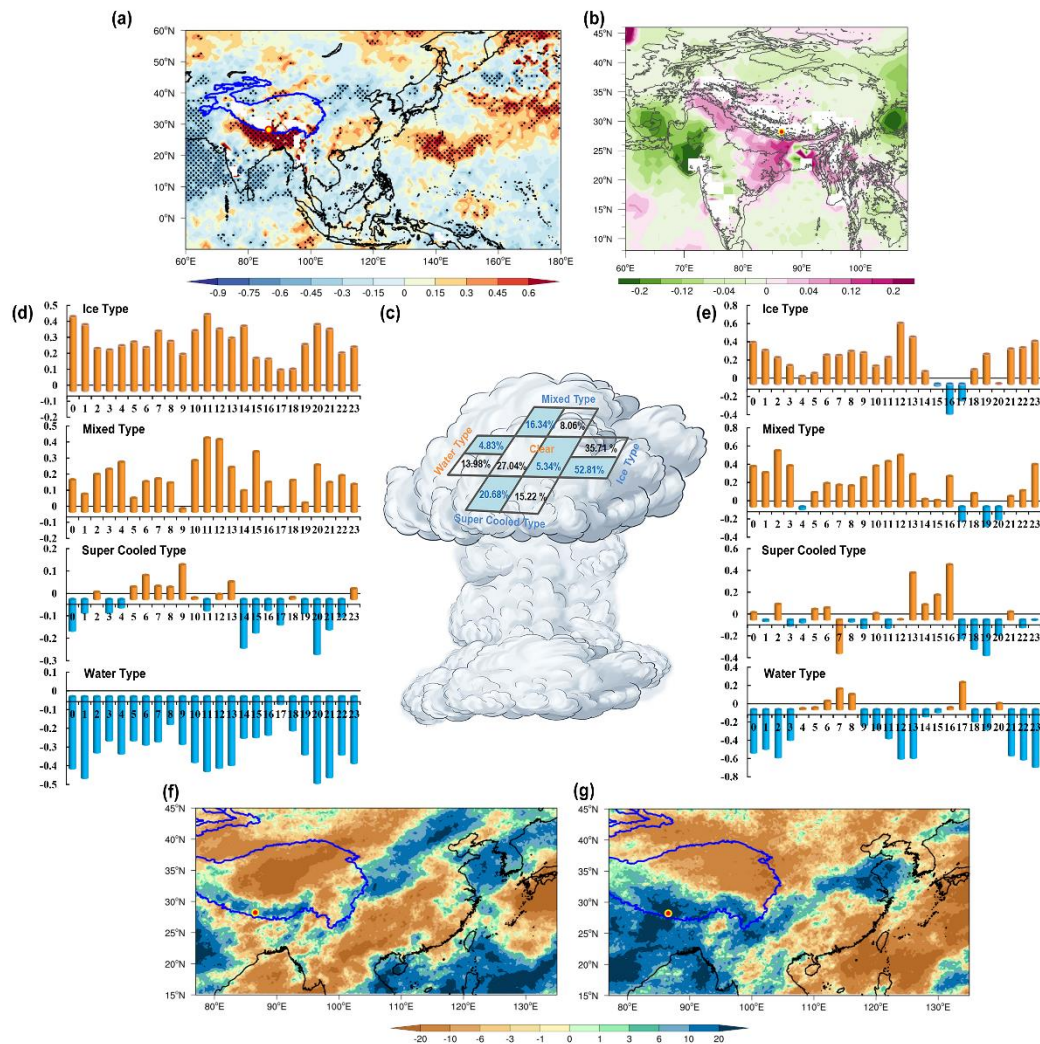
Figure 1. Aerosol distribution and cloud-phase responses over MQ: (a) Spatial correlation between AOD over the MQ region and East Asia during July 2000–2020, dotted regions
