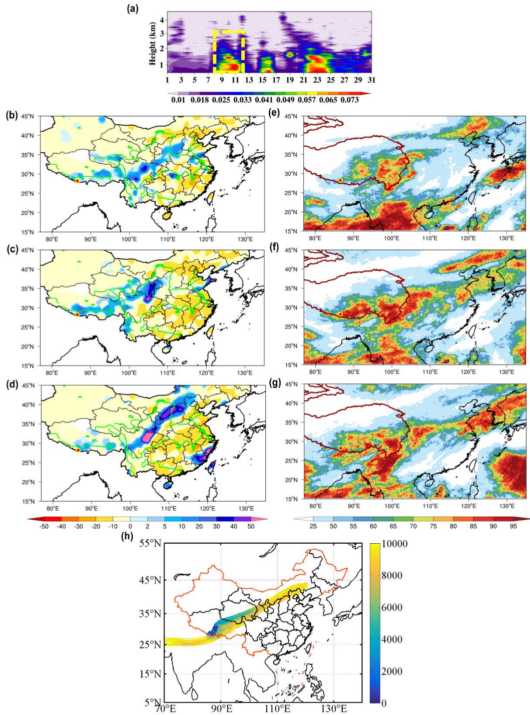
99 Figure S2. (a) Daily variations in the aerosol extinction coefficient over Mount 100 Qomolangma in 2018. The yellow box indicates the selected high-aerosol-loading 101 episode from 9 to 11 July 2018. (b–d) Evolution of precipitation in the upstream and 102 downstream regions on the day of the high-aerosol-loading event and during the 103 following two days. (e–g) Spatial distributions of ice-phase clouds accumulated over 104 the preceding 48 h for each day of the event. Panels (b, e), (c, f), and (d, g) correspond
