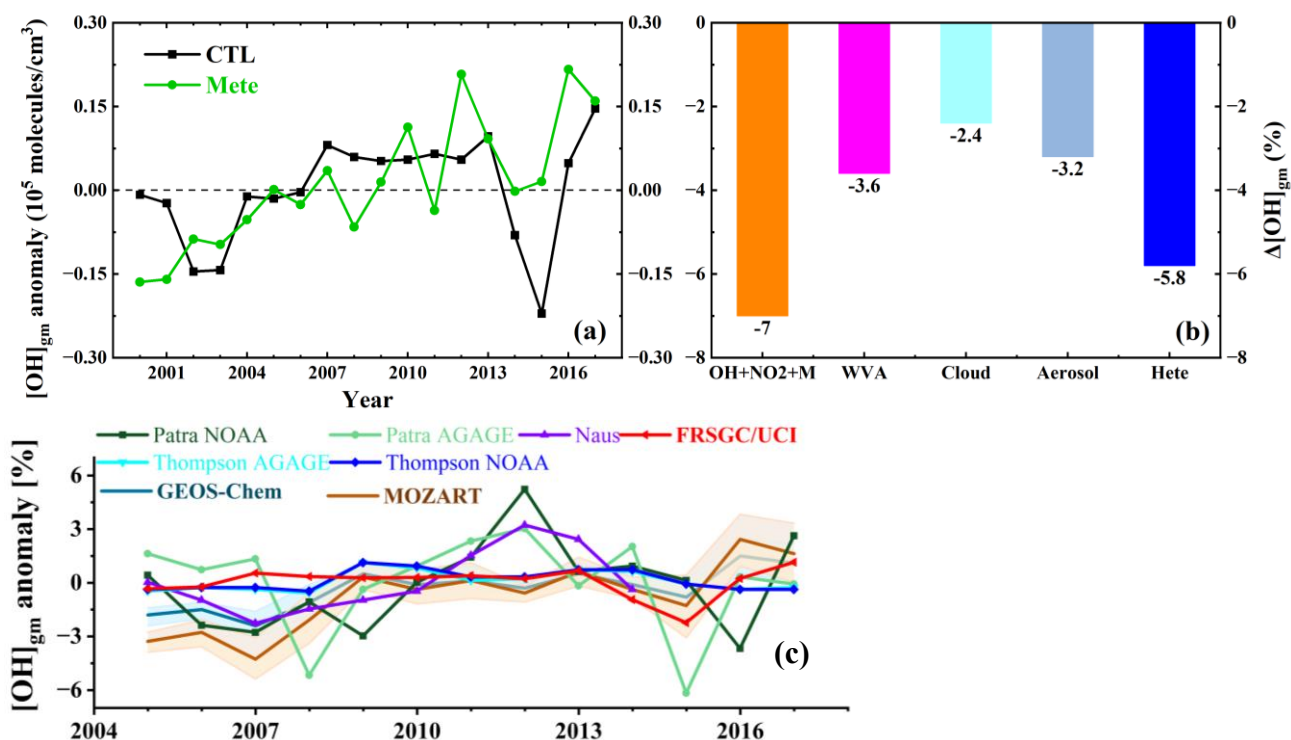
Figure 10. (a) The anomaly of [\text{OH}]_{\text{gm}} ( 10^5 \text{ molecules} \cdot \text{cm}^{-3} ) in the control run (CTL) and fixed emission run (labelled “Mete”), (b) the relative differences in annual mean [\text{OH}]_{\text{gm}} (%) between CTL and the respective sensitivity runs, averaged over 2000–
