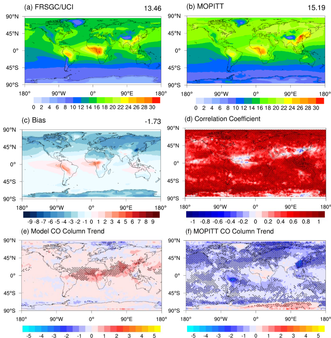
Figure 4. Same as Figure 1, but for total CO column ( 10^{17} molecules·cm -2 ) and annual mean total CO column trends ( 10^{16} molecules·cm -2 ·yr -1 ).
