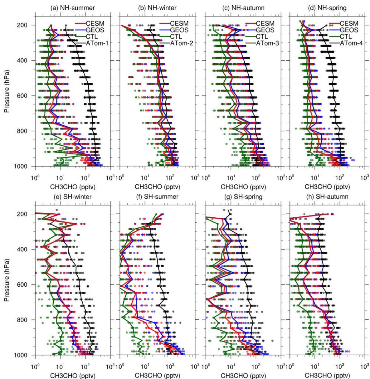
Figure 8. As Figure 5, but for \text{CH}_3\text{CHO} (pptv). The model control run (CTL) is shown in green, with results from model runs using emissions from CESM and GEOS-Chem shown in red and blue respectively.
