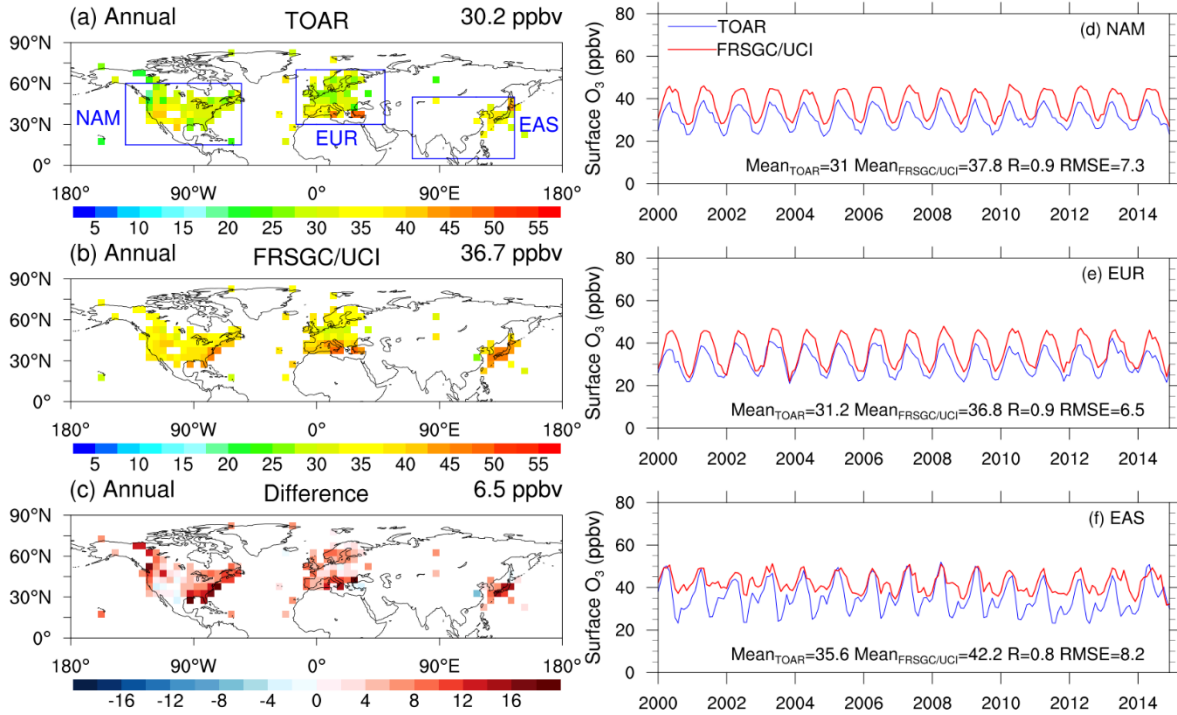
Figure 1. Observed monthly mean surface O 3 (ppbv) from TOAR and corresponding simulated O 3 from the model control run for the period January 2000 to December 2014. Panels (a) and (b) show the distributions of annual mean observed and simulated O 3 , respectively, while panel (c) shows the model–observation difference. Panels (d–f) show the corresponding regional mean time series over North America, Europe, and East Asia, respectively, with line colours indicating observations and model simulations. All modelled means are calculated only for grid squares with available observations. Global mean values are shown in the upper right corner of panels (a–c). The regional mean values, correlation coefficient (R) between observed and simulated regional means, and root mean square error (RMSE) are shown in the lower right corner of panels (d–f).
