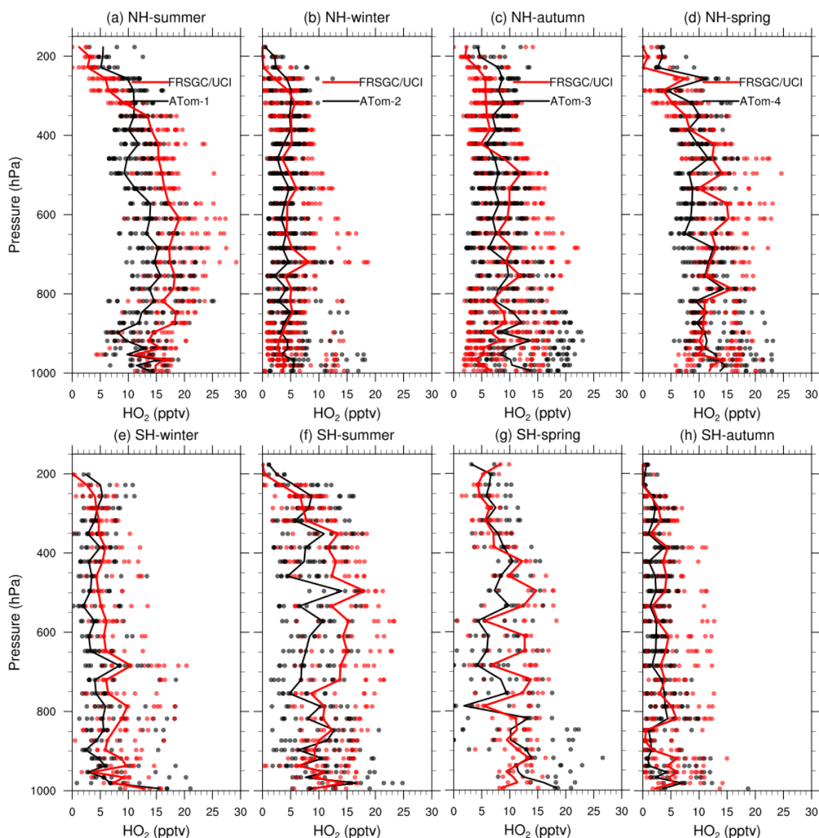
Figure 6. As Figure 5, but for HO 2 (pptv)
