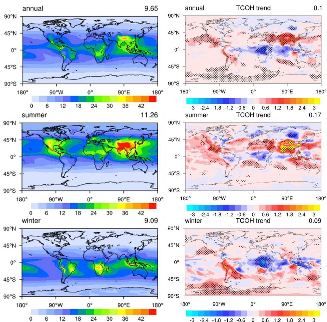
Figure 9. The tropospheric column of OH (TCOH, 10^{12} \text{ molecules} \cdot \text{cm}^{-2} , left panels) and the trend ( 10^{11} \text{ molecules} \cdot \text{cm}^{-2} \cdot \text{yr}^{-1} , right panels) in annual, winter and summer from 2000 to 2017. The troposphere was defined as the region below a climatological tropopause ( p = 300 - 215(\cos(\text{lat}))^2 ) following Lawrence et al. (2001). Trends are calculated as in Figure 2. The value in the right corner is the global average.
