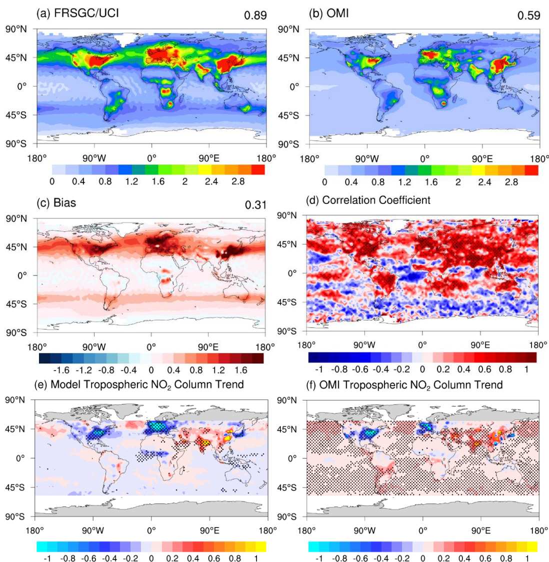
Figure 3. Same as Figure 2, but for tropospheric NO 2 column ( 10^{15} molecules·cm -2 ) and annual mean tropospheric NO 2 column trends ( 10^{14} molecules·cm -2 ·yr -1 ).
