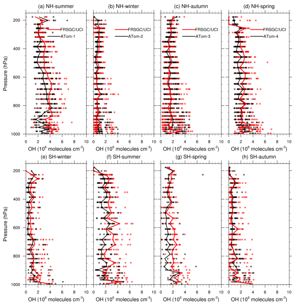
Figure 5. Median OH concentrations ( 10^6 \text{ molecules} \cdot \text{cm}^{-3} ) for the Northern Hemisphere (NH, top row) and Southern Hemisphere (SH, bottom) measured during the ATom aircraft missions (black) along with the corresponding results from the model control run (FRSGC/UCI, red). Dashed lines show the observed 25th–75th percentiles.
