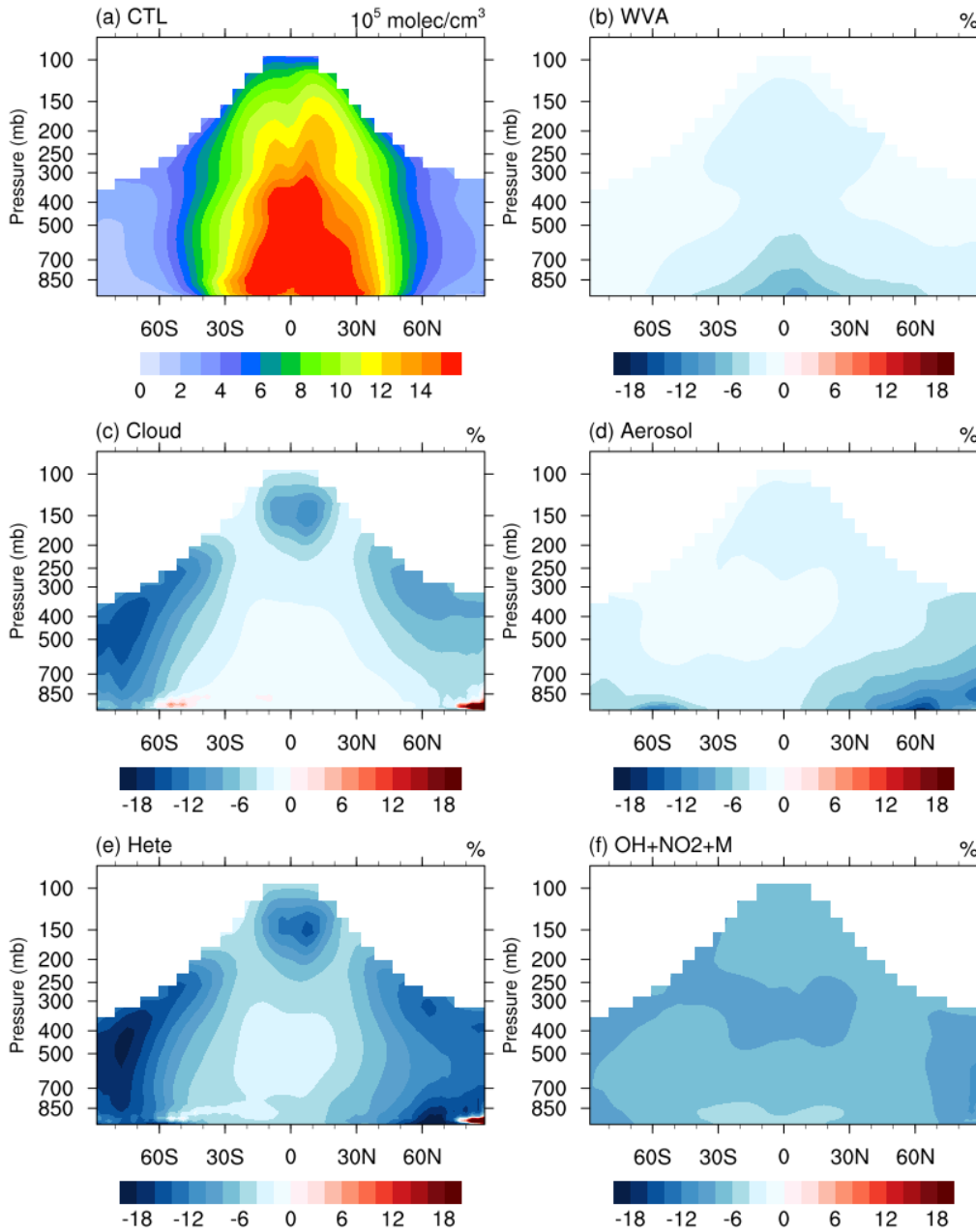
Figure 7. (a) Zonal mean (latitude-pressure) cross sections of annual mean OH concentration ( 10^5 \text{ molec} \cdot \text{cm}^{-3} ) in the CTL run and the effects on tropospheric OH (in %) of (b) water vapor UV absorption (WVA), (c) cloud heterogeneous reactions (Cloud), (d) aerosol heterogeneous reactions (Aerosol), (e) all heterogeneous reactions (Hete), and (f) the updated OH+NO 2 reaction rate. Percentage differences are calculated as (\text{CTL} - \text{experiment})/\text{CTL} \times 100\% . The troposphere was defined as the region below a climatological tropopause ( p = 300 - 215(\cos(\text{lat}))^2 ) following Lawrence et al. (2001).
