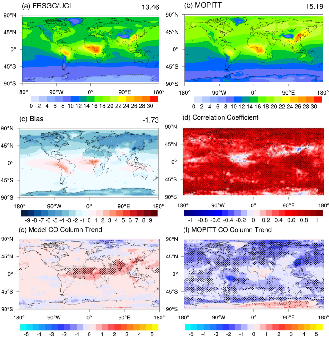
Figure 4. Same as Figure 1, but for total CO column ( 10^{17} molecules·cm -2 ) and annual mean total CO column trends ( 10^{16} molecules·cm -2 ·yr -1 ).
