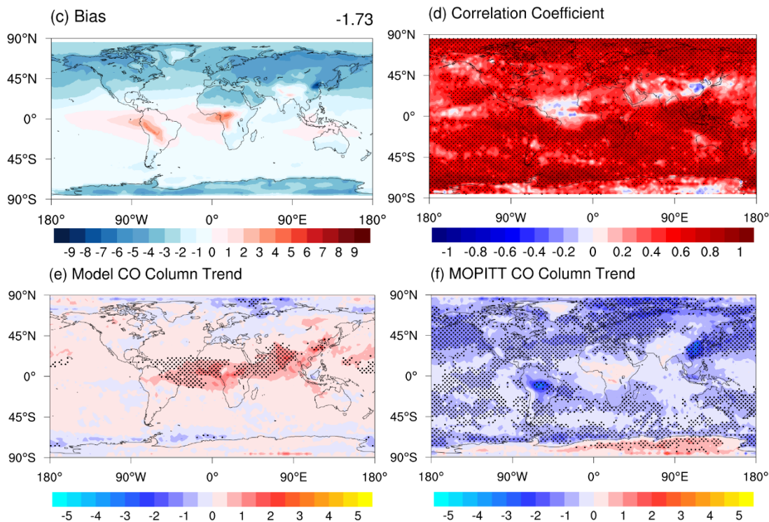
Figure 34. Same as Figure 1, but for total CO column ( 10^{17} molecules·cm ^{-2} ) and annual mean total CO column trends ( 10^{16} molecules·cm ^{-2} ·yr ^{-1} ).
