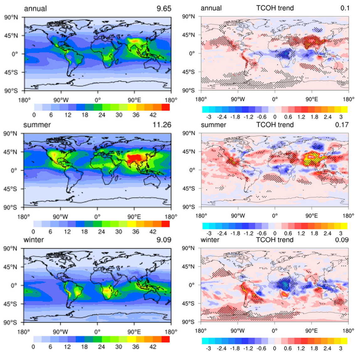
Figure 9. The tropospheric column of OH (TCOH, 10^{12} molecules·cm ^{-2} , left panels) and the trend ( 10^{11} molecules·cm ^{-2} ·yr ^{-1} , right panels) in annual, winter and summer from 2000 to 2017. The troposphere was defined as the region below a climatological tropopause ( p = 300 - 215(\cos(\text{lat}))^2 ) following Lawrence et al. (2001). Trends are calculated as in Figure 12. The value in the right corner is the global average.
