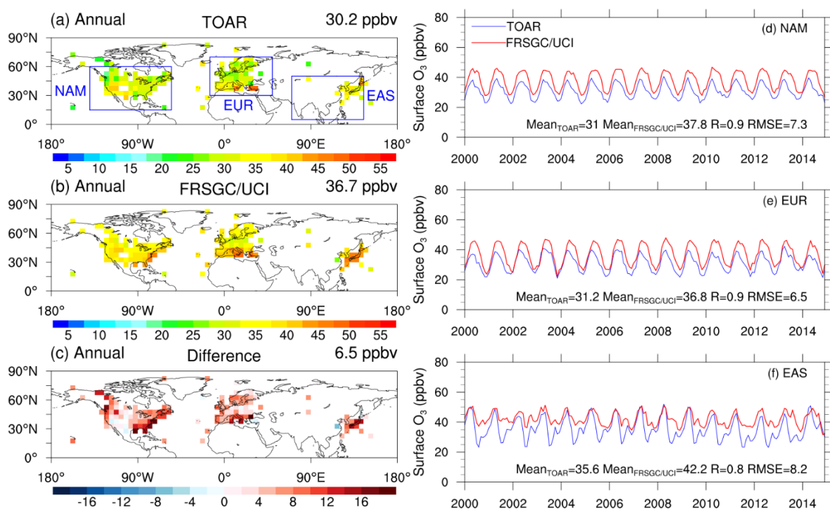
Figure 41. Observed monthly mean surface O_3 (ppbv) from TOAR and corresponding simulated O_3 from the model control run for the period January 2000 to December 2014. Panels (a) and (b) show the distributions of annual mean observed and simulated O_3 , respectively, while panel (c) shows the model–observation difference. Panels (d–f) show the corresponding regional mean time series over North America, Europe, and East Asia, respectively, with line colours indicating observations and model simulations. All modelled means are calculated only for grid squares with available observations. Global mean values are shown in the upper right corner of panels (a–c). The regional mean values, correlation coefficient (R) between
