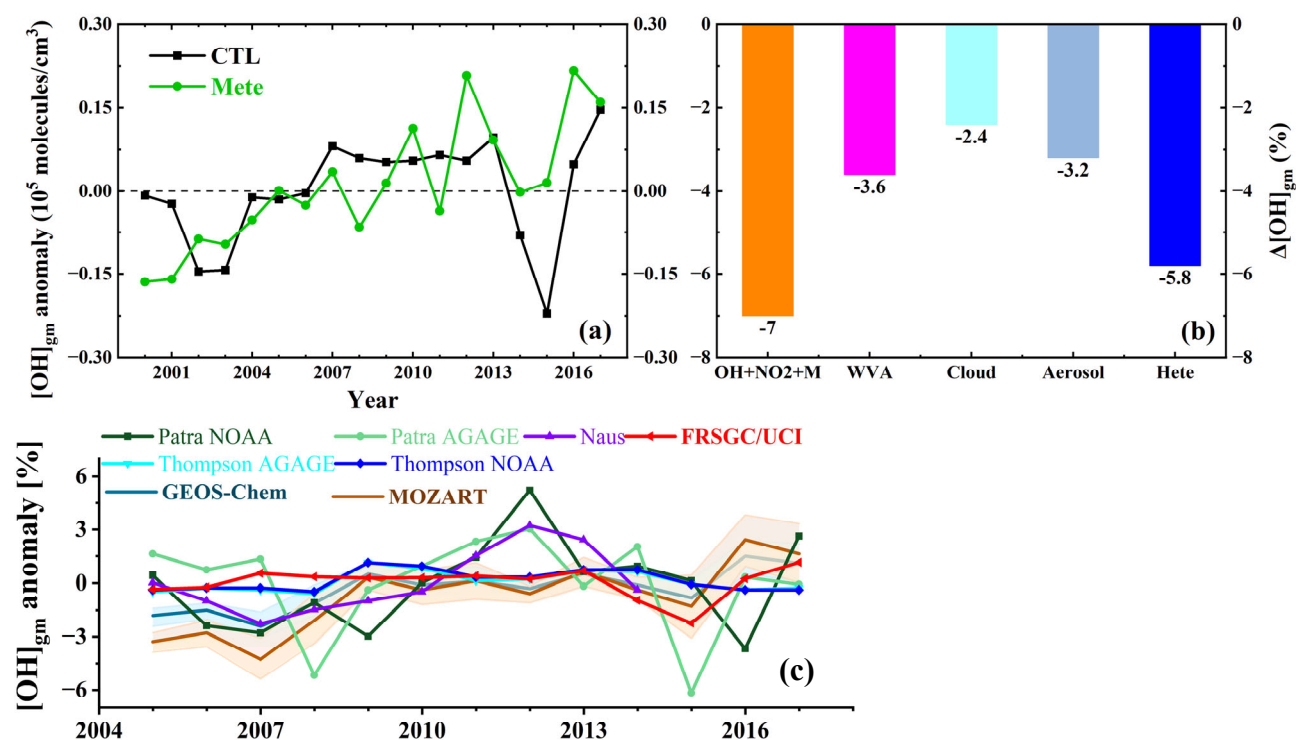
Figure 10. (a) The anomaly of [\text{OH}]_{\text{gm}} ( 10^5 \text{ molecules} \cdot \text{cm}^{-3} ) in the control run (CTL) and fixed emission run (labelled “Mete”), (b) the average relative differences in annual mean [\text{OH}]_{\text{gm}} (%) between CTL and the respective sensitivity runs, averaged over 2000–2017 from the control run (%), and (c) comparison of the relative [\text{OH}]_{\text{gm}} anomalies (%) from this work (FRSGC/UCI) and other studies. The labels in panel (b) match those in Figure 7. Results based on the MOZART and GEOS-Chem chemical mechanisms in panel (c) are from Zhao et al. (2025), the MCF-based inversion estimates are from Patra et al. (2021) and Naus et al. (2019), and the HFC-based inversion estimates are from Thompson et al. (2024).
