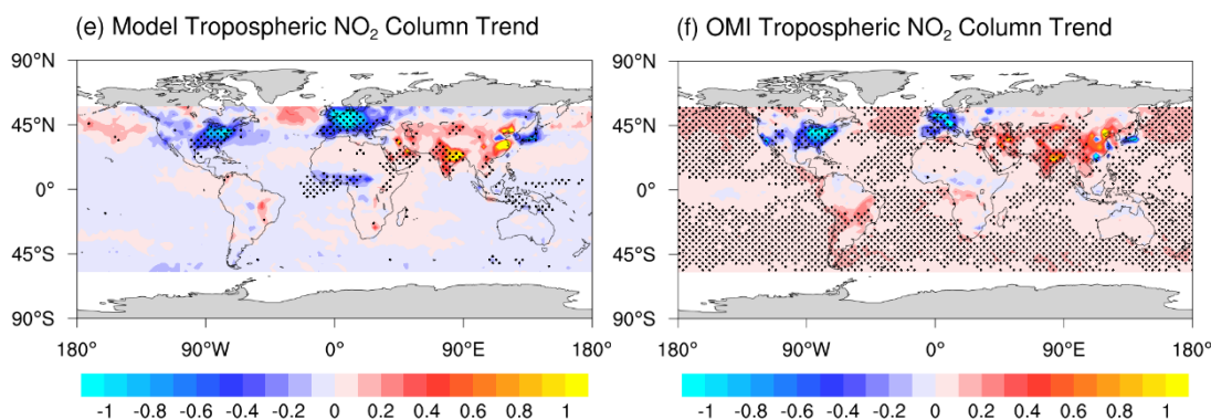
Figure 23. Same as Figure 42, but for tropospheric NO 2 column ( 10^{15} molecules·cm -2 ) and annual mean tropospheric NO 2 column trends ( 10^{14} molecules·cm -2 ·yr -1 ).
