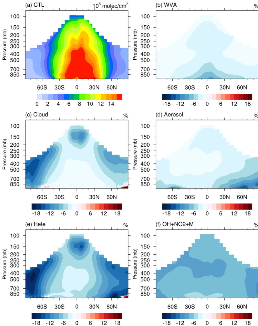
Figure 7. (a) Zonal mean (latitude-pressure) cross sections of annual mean OH concentration ( 10^5 \text{ molec}\cdot\text{cm}^{-3} ) in the CTL run and the effects on tropospheric difference in OH (in %) in the troposphere due to (b) removing water vapor UV absorption (WVA), (c) removing cloud heterogeneous reactions (Cloud), (d) removing aerosol heterogeneous reactions (Aerosol), (e) removing all heterogeneous reactions (Hete), and (f) altering the updated reaction rate for OH+NO 2 reaction rate (JPL). Percentage differences are calculated as (\text{CTL} - \text{experiment})/\text{CTL} \times 100\% . The troposphere was defined as the region below a climatological tropopause ( p = 300 - 215(\cos(\text{lat}))^2 ) following Lawrence et al. (2001).
