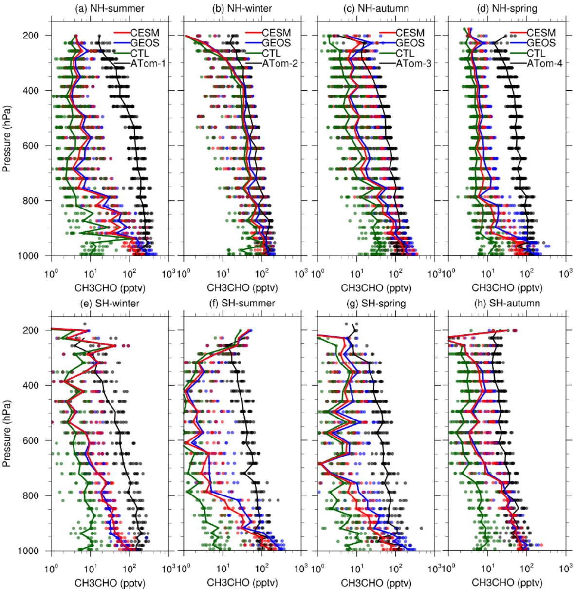
Figure 8. As Figure 5, but for CH 3 CHO (pptv). The model control run (CTL) is shown in green, with results from model runs using emissions from CESM and GEOS-Chem shown in red and blue respectively.
