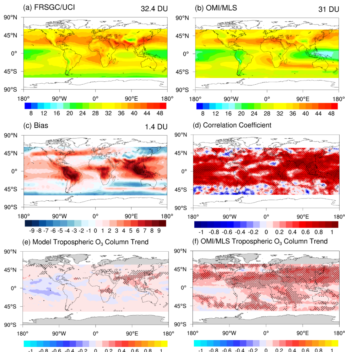
Figure 12. Multiyear average (2005–2017) tropospheric O 3 column (DU) from (a) the model control run and (b) OMI/MLS satellite observations. Panel (c) shows the corresponding mean bias of the tropospheric O 3 column (model minus observation), and (d) shows the correlation coefficient of between annual mean modelled and OMI/MLS tropospheric O 3 column time series at each grid box annual-mean tropospheric O 3 column between model and observations . Annual mean tropospheric O 3 column trends (DU·yr -1 ) are shown in (e) for the model and (f) for satellite observations over the 2005–2017 period. Global mean columns between 60°S–60°N are indicated in the upper right corner of panels (a)–(c). Shaded areas in (d) indicate regions where the correlation is statistically significant at the 95% confidence level (p < 0.05). Trends in panels (e) and (f) were calculated using the Theil–Sen method, and stippling indicates areas with significant trends at the 95% confidence level according to the Mann–Kendall test.
