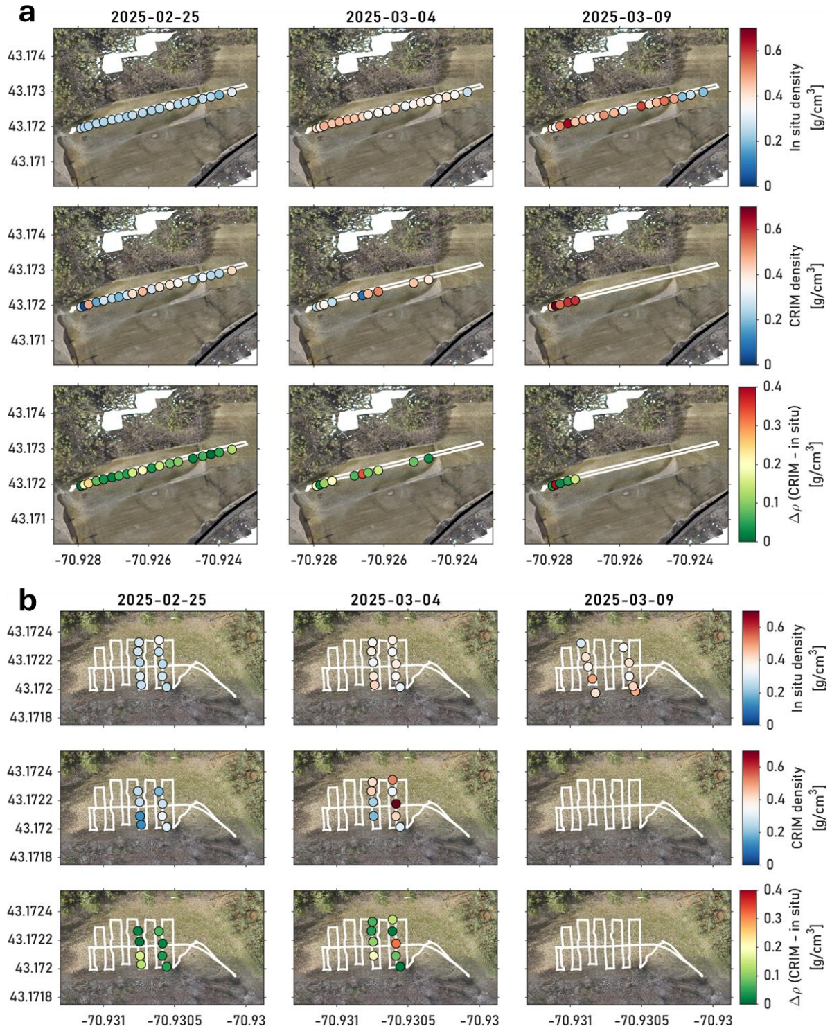
Figure S2: Spatial distribution of the difference between CRIM-derived snow density and in situ measured density along the transects at the open (a) and sheltered forest (b) on three survey dates. Point colors represent the density difference. Points are shown only where both GPR-derived permittivity and in situ measurements were available.
