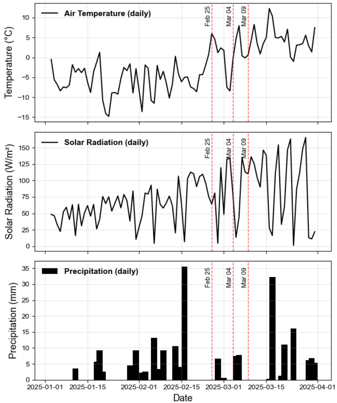
Figure S1: Meteorological and winter conditions at Kingman Farm during the observation period (January – March 2025). Vertical lines indicate the dates of the three UAS-GPR surveys.
