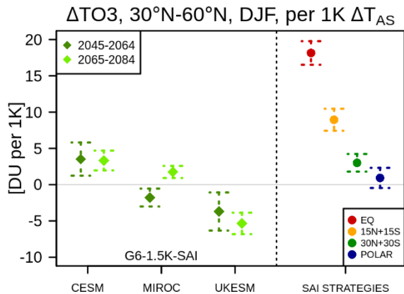
Figure 9. As in Figure 8(f) but for the NH mid-latitude (30°N-60°N) total ozone column in boreal winter, i.e. December-January-February (DJF) mean.
