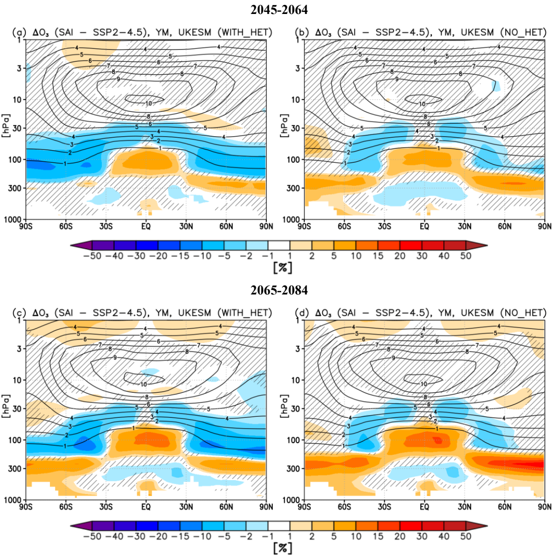
Figure 12. Shading: Annual (top, a-b) 2045-2064 mean and (bottom, c-d) 2065-2084 mean changes in ozone volume mixing ratios between the UKESM G6-1.5K-SAI simulations and the SSP2-4.5 simulations over the same period. Left (a,c) is for the fully coupled simulation discussed in the paper (as in Fig. 4), and right (b,d) is for the sensitivity simulation without heterogeneous chemistry on SAI sulfate aerosols. Contours and shading as in Figure 4.
