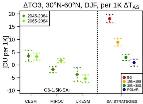
400 Figure 9. As in Figure 8(f) but for the NH mid-latitude (30°N-60°N) total ozone column in boreal winter, i.e. December-January-February (DJF) mean.
