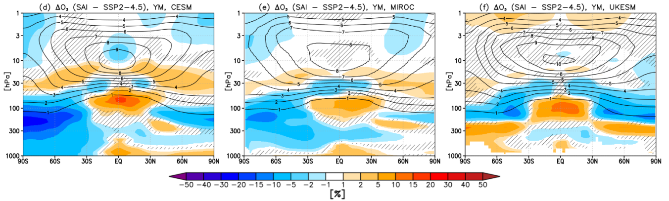
Figure 4. Shading: Annual (top, a-c) 2045-2064 mean and (bottom, d-f) 2065-2084 mean changes in ozone ( O_3 ) volume mixing ratios between the G6-1.5K-SAI simulations and the SSP2-4.5 simulations over the same period for each model (columns). Contours show the corresponding climatological ozone volume mixing ratios (in ppm) in the SSP2-4.5 runs for reference. Hatching marks the region where the response is not statistically significant (defined as in Fig. 1)
