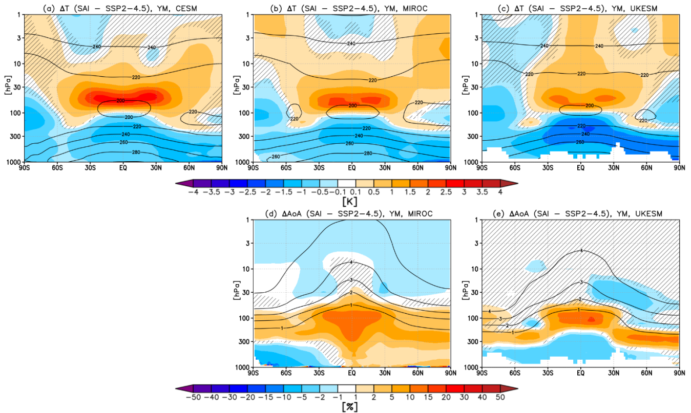
Figure 5. Shading: Annual 2045-2064 mean changes in (top, a-c) temperatures and (bottom, d-e) age-of-air between the G6-1.5K-SAI simulations and the SSP2-4.5 simulations over the same period for each model (columns). Contours show the corresponding climatological values in the SSP2-4.5 runs for reference. Hatching marks the region where the response is not statistically significant (defined as in Fig. 1). Note that an age-of-air diagnostic is not available for CESM.
