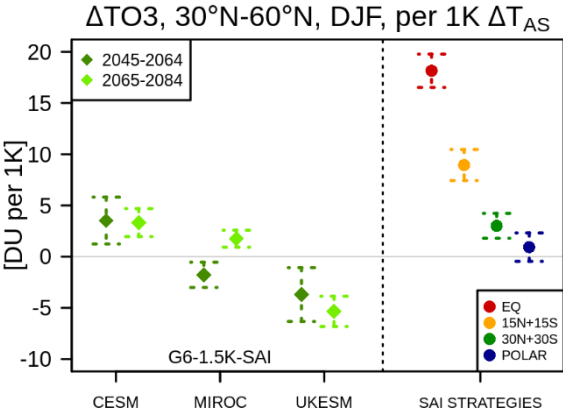
415 Figure 9. As in Figure 8(f) but for the NH mid-latitude (30°N-60°N) total ozone column in boreal winter, i.e. December-January-February (DJF) mean.
