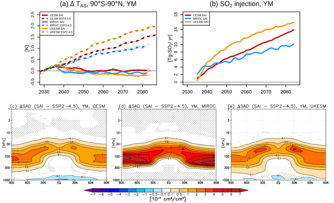
Figure 1. Top: (a) Timeseries of ensemble mean changes in annual mean (‘YM’) global mean near-surface air temperature ( T_{AS} ) in each model (colors) in the G6-1.5K-SAI (solid) or SSP2-4.5 experiments (dashed). Anomalies are calculated relative to each model’s baseline (i.e. 2020-2039 ensemble mean of the SSP2-4.5 simulation). Thin lines denote the ensemble mean changes and thick lines denote their 5-year running means. (b) Timeseries of ensemble mean annual \text{SO}_2 injection rates in each model’s G6-1.5K-SAI experiment (colors). Bottom (c-e): Annual 2045-2064 mean changes in aerosol surface area density (SAD) between G6-1.5K-SAI and SSP2-4.5 over the same period in each model (columns). Hatching marks the region where the response is not statistically significant (taken as smaller than \pm 2 standard errors in the difference in means, calculated using standard deviations of both SAI and no-SAI experiments with 20 annual mean values per ensemble members).
