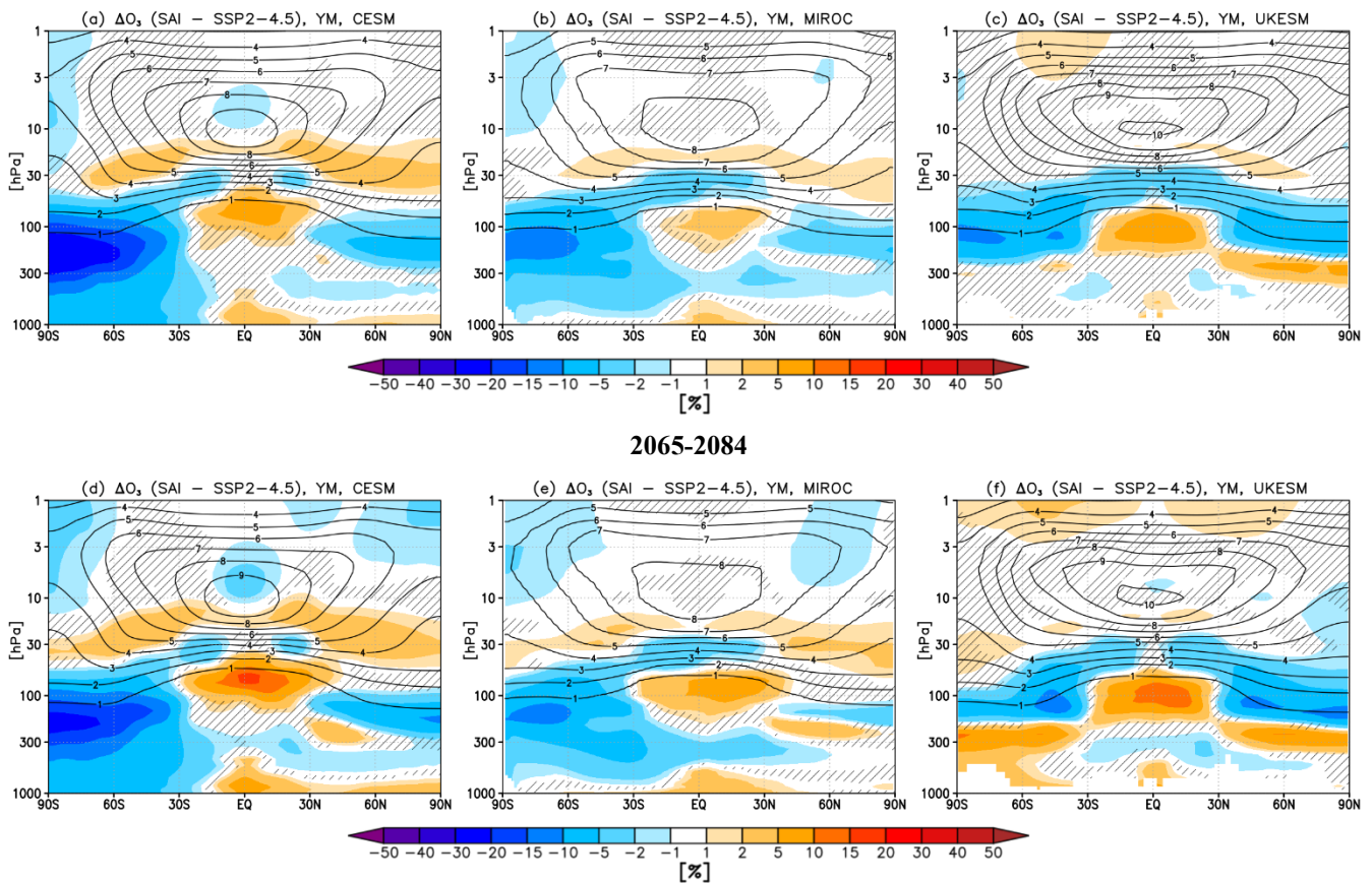
275 Figure 4. Shading: Annual (top, a-c) 2045-2064 mean and (bottom, d-f) 2065-2084 mean changes in ozone ( O_3 ) volume mixing ratios between the G6-1.5K-SAI simulations and the SSP2-4.5 simulations over the same period for each model (columns). Contours show the corresponding climatological ozone volume mixing ratios (in ppm) in the SSP2-4.5 runs for reference. Hatching marks the region where the response is not statistically significant (defined as in Fig. 1)
