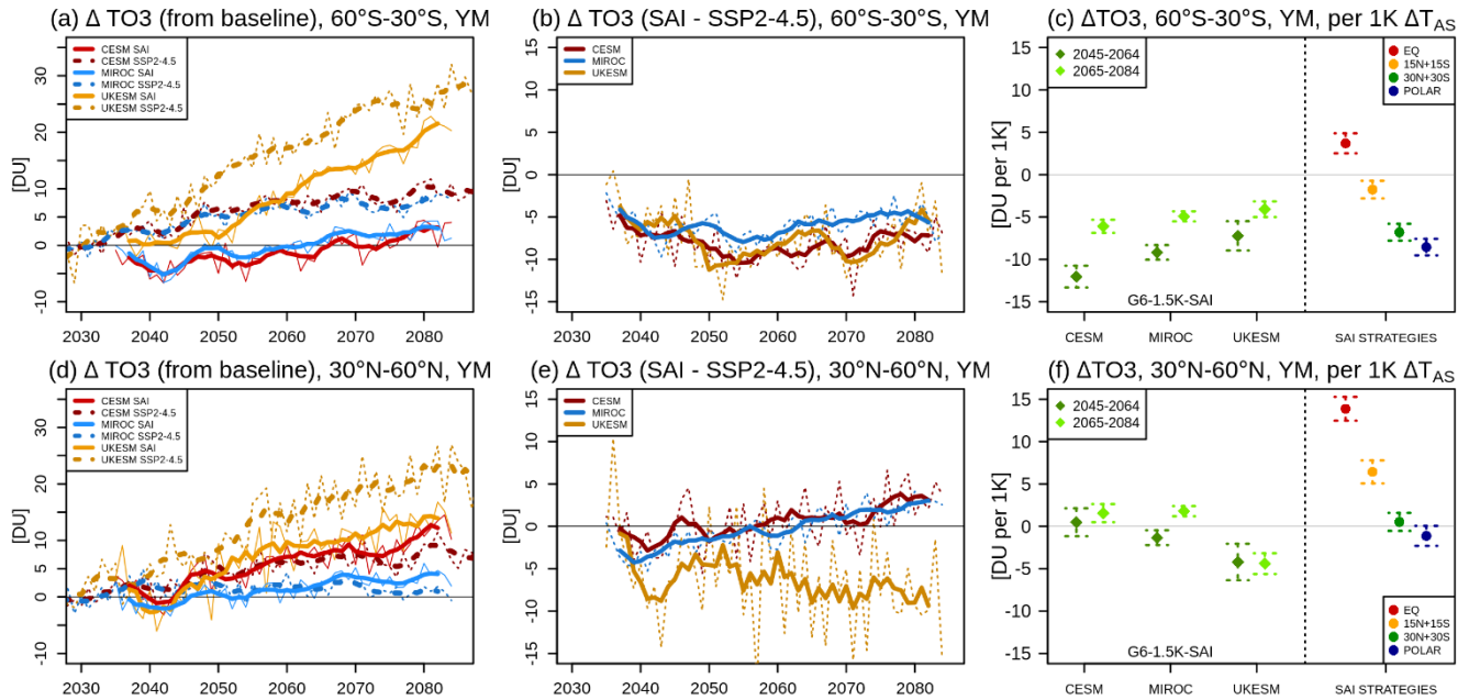
Figure 8. Annual mean (top, a-c) SH mid-latitude (60°S-30°S) and (bottom, d-f) NH mid-latitude (30°N-60°N) total column ozone changes for each of the models. (a,d) Timeseries of differences from the baseline period (2020-2039 mean of SSP2-4.5) in the control SSP2-4.5 simulations (dashed) and the corresponding G6-1.5K-SAI simulations (solid). Thin lines in (a-b) denote the ensemble mean changes for each model and thick lines denote their 5-year running means. (c,f): Normalized total column ozone changes between the G6-1.5K-SAI and SSP2-4.5 simulations averaged over either 2045-2064 or 2065-2084 periods and scaled with the corresponding global mean near-surface air temperature change. Shown also are the corresponding changes (2050-2069) in the different SAI strategies discussed in Bednarz et al. (2023a; see text for more details). The error bars represent \pm 2 standard errors in the difference in means, calculated from the annual mean values (20 per ensemble member).
