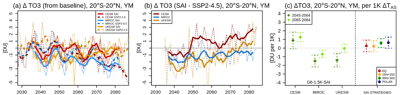
Figure 3. Annual mean tropical (20°S-20°N) total column ozone changes for each of the models. (a) Timeseries of differences from the baseline period (2020-2039 mean of SSP2-4.5) in the control SSP2-4.5 simulations (dashed) and the corresponding G6-1.5K-SAI simulations (solid). (b) Timeseries of differences between the G6-1.5K-SAI and SSP2-4.5 simulations. Thin lines in (a-b) denote the ensemble mean changes for each model and thick lines denote their 5-year running means. (c): Normalized total column ozone changes between the G6-1.5K-SAI and SSP2-4.5 simulations averaged over either 2045-2064 or 2065-2084 periods and scaled with the corresponding global mean near-surface air temperature change. Shown also are the corresponding changes (2050-2069) in the different SAI strategies discussed in Bednarz et al. (2023a; see text for more details). The error bars represent +/- 2 standard errors in the difference in means, calculated from the annual mean values (20 per ensemble member).
