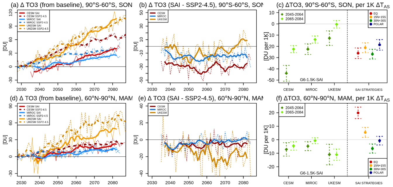
Figure 10. Springtime (top, a-c) SH high-latitude (90°S-60°S, September-October-November, SON) and (bottom, d-f) NH high-latitude (60°N-90°N, March-April-May, MAM) total column ozone changes for each of the models. (a,d) Timeseries of differences from the baseline period (2020-2039 mean of SSP2-4.5) in the control SSP2-4.5 simulations (dashed) and the corresponding G6-1.5K-SAI simulations (solid). (b,e) Timeseries of differences between the G6-1.5K-SAI and SSP2-4.5 simulations. Thin lines in (a-b) denote the ensemble mean changes for each model and thick lines denote their 5-year running means. (c,f): Normalized total column ozone changes between the G6-1.5K-SAI and SSP2-4.5 simulations averaged over either 2045-2064 or 2065-2084 periods and scaled with the corresponding global mean near-surface air temperature change. Shown also are the corresponding changes (2050-2069) in the different SAI strategies discussed in Bednarz et al. (2023a; see text for more details). The error bars represent +/- 2 standard errors in the difference in means, calculated from the annual mean values (20 per ensemble member).
