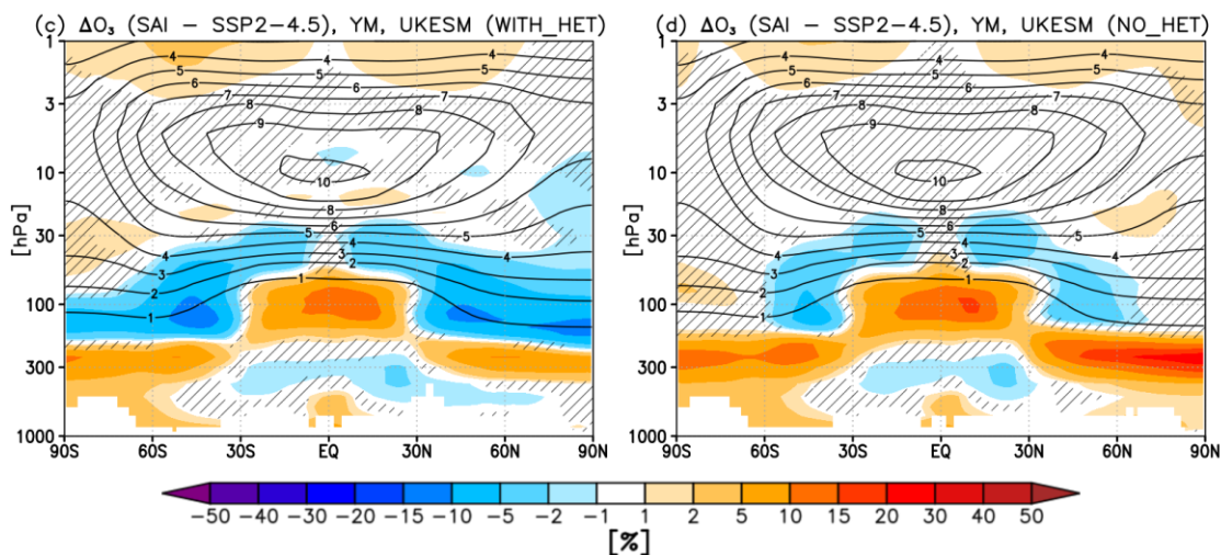
Figure 12. Shading: Annual (top, a-b) 2045-2064 mean and (bottom, c-d) 2065-2084 mean changes in ozone volume mixing ratios between the UKESM G6-1.5K-SAI simulations and the SSP2-4.5 simulations over the same period. Left (a,c) is for the fully coupled simulation discussed in the paper (as in Fig. 4), and right (b,d) is for the sensitivity simulation without heterogeneous chemistry on SAI sulfate aerosols. Contours and shading as in Figure 4.
