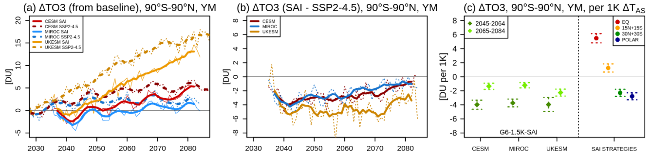
Figure 2. Annual and global mean total column ozone (TO3) changes for each of the models. (a) Timeseries of differences from the baseline period (2020-2039 mean of SSP2-4.5) in the control SSP2-4.5 simulations (dashed) and the corresponding G6-1.5K-SAI simulations (solid). (b) Timeseries of differences between the G6-1.5K-SAI and SSP2-4.5 simulations. Thin lines in (a-b) denote the ensemble mean changes for each model and thick lines denote their 5-year running means. (c): Normalized total column ozone changes between the G6-1.5K-SAI and SSP2-4.5 simulations averaged over either 2045-2064 or 2065-2084 periods and scaled with the corresponding global mean near-surface air temperature change. Shown also are the corresponding changes (2050-2069) in the different SAI strategies with CESM2(WACCM6-MA) - EQ, 15N+15S, 30N+30S, POLAR - discussed in Bednarz et al. (2023a), see text for more detail. The error bars represent \pm 2 standard errors in the difference in means, calculated from the annual mean values (20 per ensemble member).
