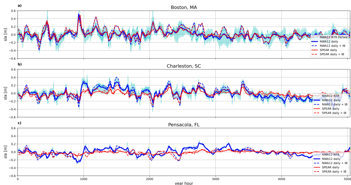
Figure 3. SPEAR (red) and NWA12 (blue) coastal sea level at Boston, MA (a), Charleston, SC (b), and Pensacola, FL (c) tide gauge stations for the 2015-12-01 – 2016-06-30 period. Tides and a twenty-year mean season cycle have been removed. Hourly non-tidal residuals are in light blue. Solid and dashed lines are daily averages without and with the diagnosed IB contribution.
