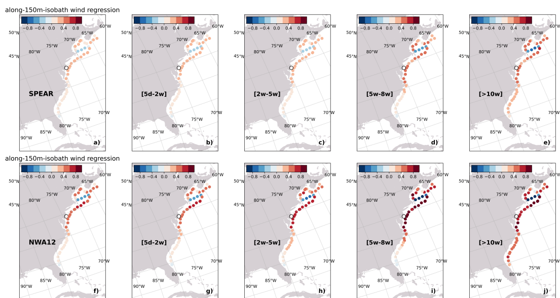
Figure 7. Regression of along-150 m isobath winds with SPEAR total SSH at Atlantic City, NJ (open-circle) (a) and as a function of frequency band (b-e). f-j) Same as a-e but for NWA12.
