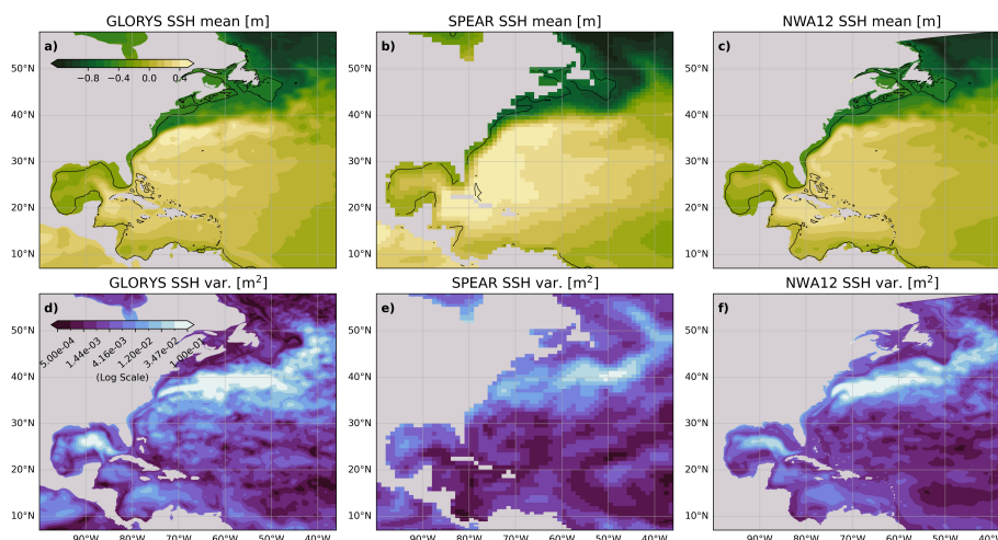
Figure 1. a-c) GLORYS, SPEAR, and NWA12 annual mean sea surface height (SSH) (for GLORYS we show dynamic sea level, such that the zero value corresponds to the global mean. This is used to initialize NWA12 SSH referenced to the model ellipsoid). The 150 m isobath is contoured in black. d-f) GLORYS, SPEAR, and NWA12 annual mean sea surface height variance (note log colorscale).
