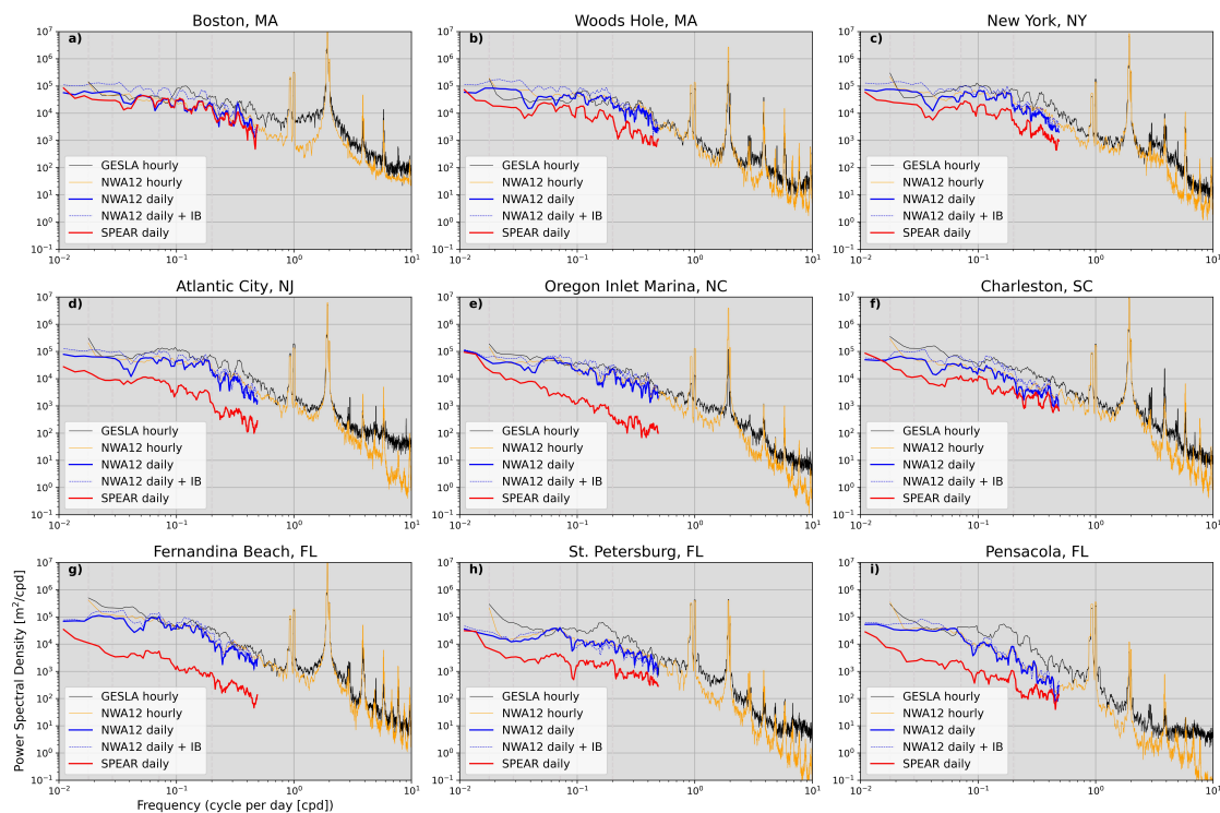
Figure 4. Power spectral density at nine tide gauge stations. Black denotes observed and yellow NWA12 hourly spectra for the 2018-12-01 simulation start time. Solid red (SPEAR) and blue (NWA12) are daily spectra with the blue dashed line adding the IB contribution. Moving left to right, light gray vertical dashed lines correspond to 2-month, 1-month, 2-week, and 5-day periods.
