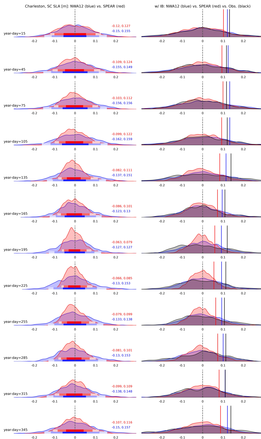
Figure 11. left) Distributions of daily SPEAR (red) and NWA12 (blue) sea level anomalies (SLA) at the Charleston, SC tide gauge station as a function of lead month. Horizontal bands denote 5,10,25,75,90,95 percentiles. Red and blue text are 5th and 95th percentile values for SPEAR and NWA12. right) Distributions of daily SPEAR (red), NWA12 (blue), and observations (black) with the IB effect included. Solid vertical lines denote corresponding standard deviations.
