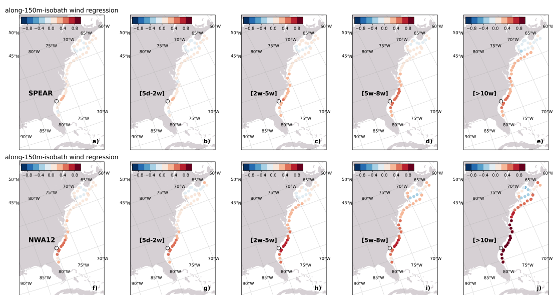
Figure 8. Regression of along-150 m isobath winds with SPEAR total SSH at Charleston, SC (open-circle) (a) and as a function of frequency band (b-e). f-j) Same as a-e but for NWA12.
