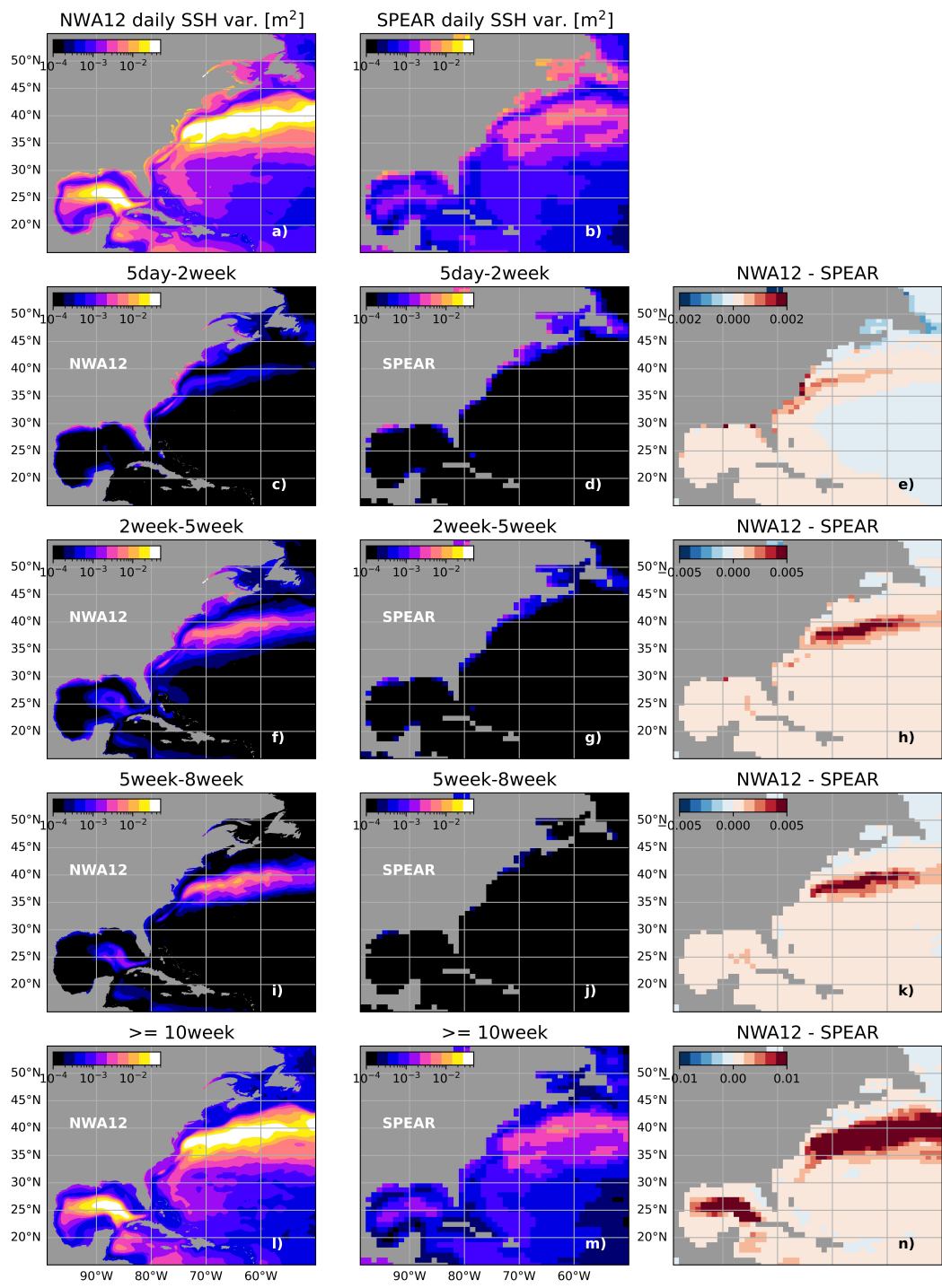
Figure 6. a-b) Deseasonalized total SPEAR and NWA12 sea surface height variance. Variance is partitioned into four frequency bands [5 day - 2 week (c,d), 2 week - 5 week (f,g), 5 week - 8 week (i,j), and greater than 10 weeks. e,h,k,n) Differences in variance (NWA12 - SPEAR) at SPEAR horizontal resolution.]
