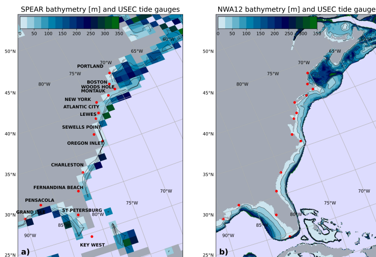
Figure 2. a) SPEAR and b) NWA12 continental shelf and slope bathymetry [0 - 350 m] colored at respective ocean model grid resolution. Black contours correspond to 25, 50, 100, and 150 m isobaths. Red dots locate the 15 tide gauge stations whose data are used in this analysis.
