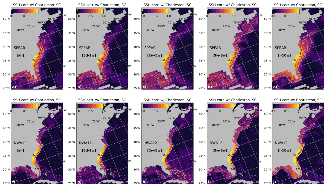
Figure 9. SPEAR (a-e) and NWA12 (f-j) SSH correlation with SSH at the Charleston, SC tide gauge station. Black contour is the 150 m isobath.
