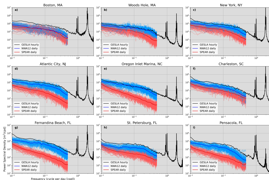
Figure 5. SPEAR (red) and NWA12 (blue) daily-mean power spectral density curves at nine tide gauge stations. Averages across twenty initialization years and ensemble members are added as thicker red and blue curves. Twenty-year mean spectra computed from hourly observations is added in black.
