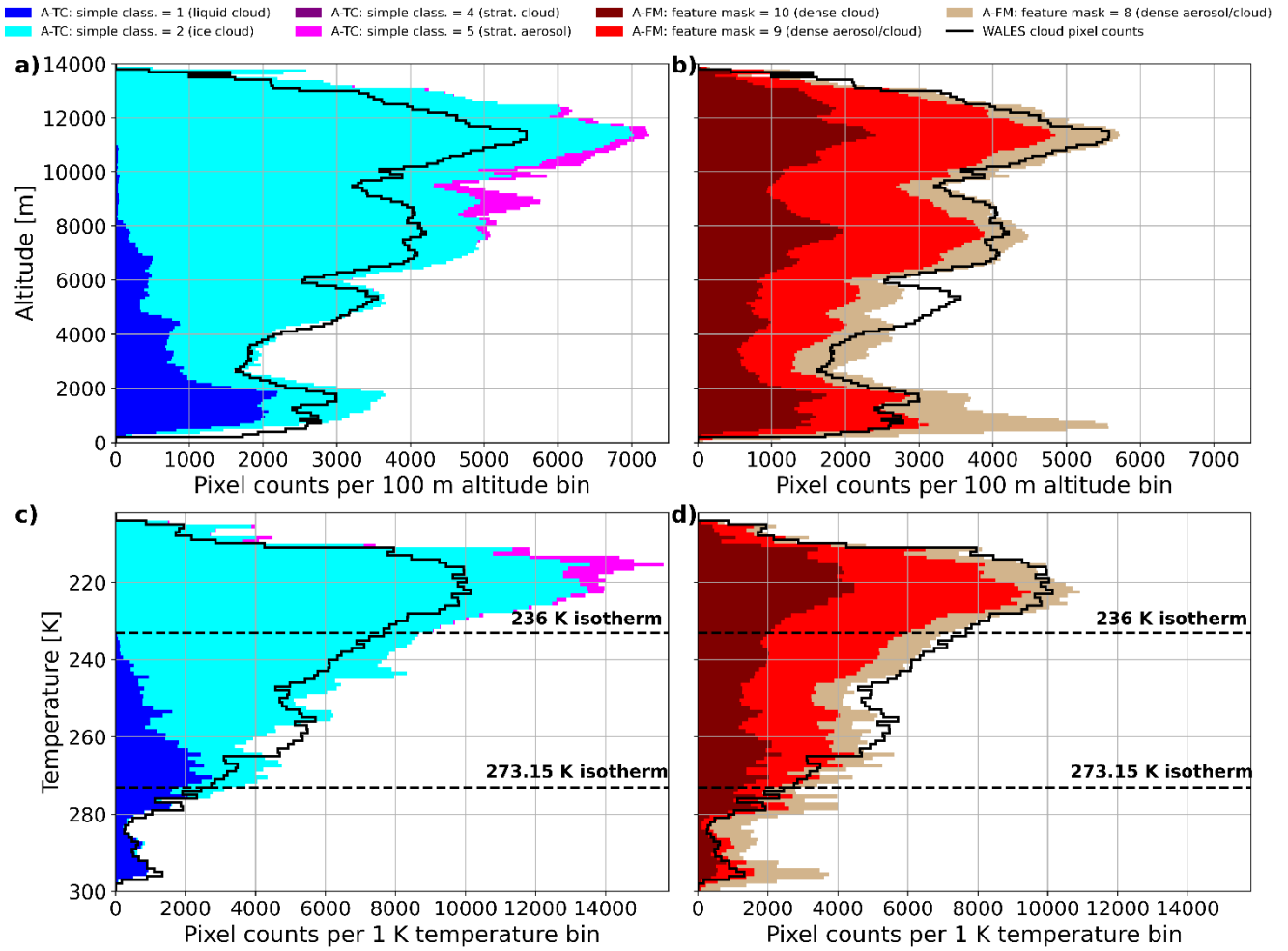
Figure 6: Vertical distributions of cloud pixels determined from WALES (black step histogram) for the 40 full EarthCARE underflight segments. Histograms are shown for 100 m altitude bins in (a, b) and for 1 K temperature bins in (c, d). The stacked colouring in (a) and (c) represent the pixel counts from the A-TC simple classification, whereas in (b) and (d) the colouring shows the distribution of atmospheric features classified by the A-FM product (see legend).
