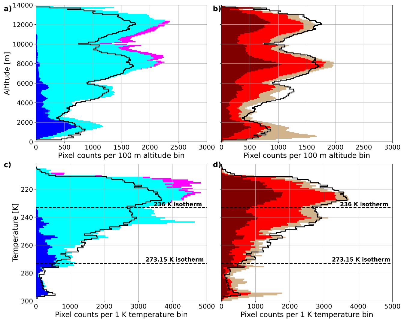
Figure D1: Same as Figure 6 c,d, but focus on observations within \pm 138 km / 10 min, with the same coloring of the different flags of A-FM and A-TC. The similarity of the distributions compared to Fig. 6 underlines the strong consistency between cloud pixels of the full dataset and the segments close to the underpass (i.e., of higher expected representativeness).
