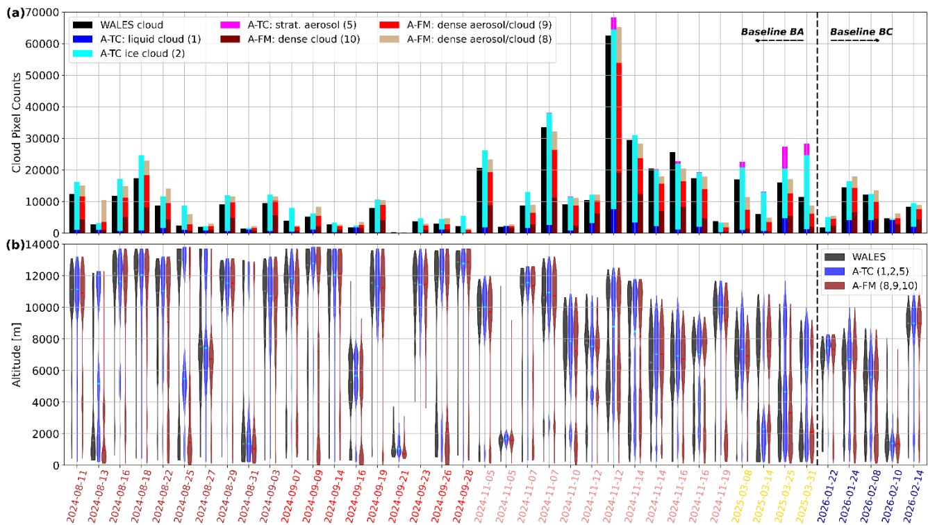
Figure 5: (a) Number of cloud pixel counts per research flight given as bar plots for WALEs, A-TC's simple classification (flag 1,2,5), and the A-FM's feature mask (flag 8-10) with the same colouring as in Fig. 3. (b) illustrates the vertical distribution of cloud pixels as violin boxplots for WALEs (black), A-TC (blue) and A-FM (red). The horizontal bars inside the violins represent the median. The colouring of the x-axis labels corresponds to the different field campaign with the same color-coding as in Fig. 1.
