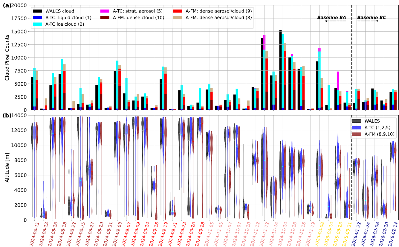
880 Figure C1: Same as Fig. 5, for data within \pm 10 min; 138 km centred around the EarthCARE underpass).
