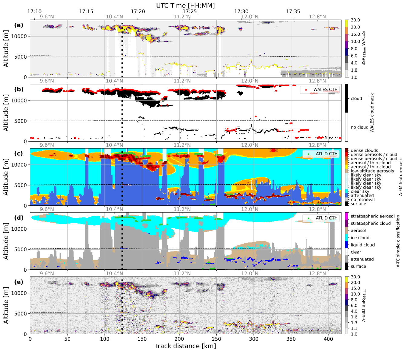
340 Figure 3: Time-altitude cross sections for the research flight on the 7 September 2024 from Barbados (PERCUSSION-WEST) of (a) the BSR measured from WALES, (b) the cloud mask (black contours) and the top altitude of the uppermost cloud (red dots) as determined from WALES BSR, (c) the feature mask of the A-FM product, (d) the simple classification of the A-TC product, and (e)
