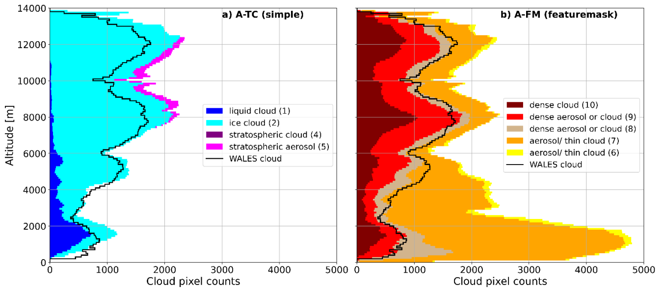
Figure B1: Same as Figure 6 a, b but inclusion of thin features in A-FM (values 6,7). Shown are data within \pm 10 min; 138 km centred around the EarthCARE underpass. Note that the x-axis are changed compared to Fig.6.
