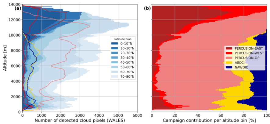
Figure 2: (a) Histogram of the cloud pixels (in 100 m altitude bins) determined from WALES for the full 40 EarthCARE underflights coloured with blueish contours by 10° bins of latitude, and number of cloud pixels observed per campaign (coloured lines), and (b) percentage contribution of each campaign per altitude bin.
