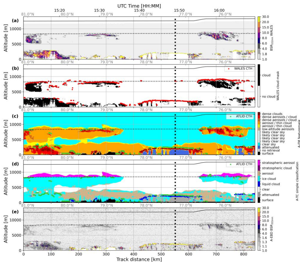
Figure 4: Time-altitude cross sections with the same parameters as for Fig. 3, but for the research flight on the 31 March 2025 from Kiruna (ASCCI). The horizontal black dashed line in (c)-(e) represents the tropopause altitude provided from A-EBD. All AT-LID Level 2 products shown represent baseline BA.
