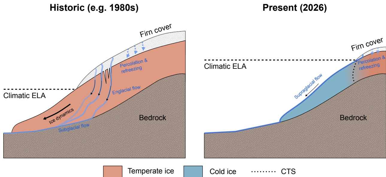
Figure 9. Conceptual illustration of the thermal consequences of firn cover loss under glacier recession, comparing the 1980s with present-day (2026) conditions.
