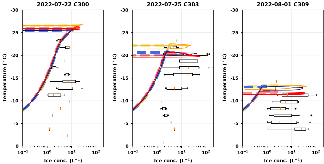
Figure 5. Observed and simulated ice particle concentrations as a function of temperature for the three selected cases. In each panel, the boxplots show the observed ice concentrations based primarily on CPI data, and the coloured lines show the parcel model simulations under different entrainment scenarios. Blue, orange, and red lines represent the HOM+EA, INHOM+EA+RA, and ADIA simulations, respectively. Solid lines represent simulations with all SIP mechanisms activated, while dashed lines indicate simulations with SIP processes disabled.
