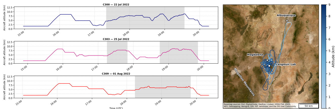
Figure 1. The left panel shows the time series of aircraft altitude for the three selected DCMEX cases, with shaded periods indicating cloud penetration. The right panel shows the corresponding flight track for the case on 22 July 2022 (C300).
