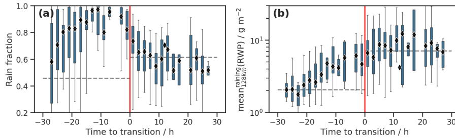
Figure 13. Same as Decomposition of RWP in Fig. 11–12(b–f), but for in (a) rain fraction, and (b) mean RWP below cloud, (c) where the mean rain-water content at cloud base and is taken only over raining profiles (d) 95th percentile instead of rain-water content at cloud base, from ACM-CAP over all cloudy profiles ).
