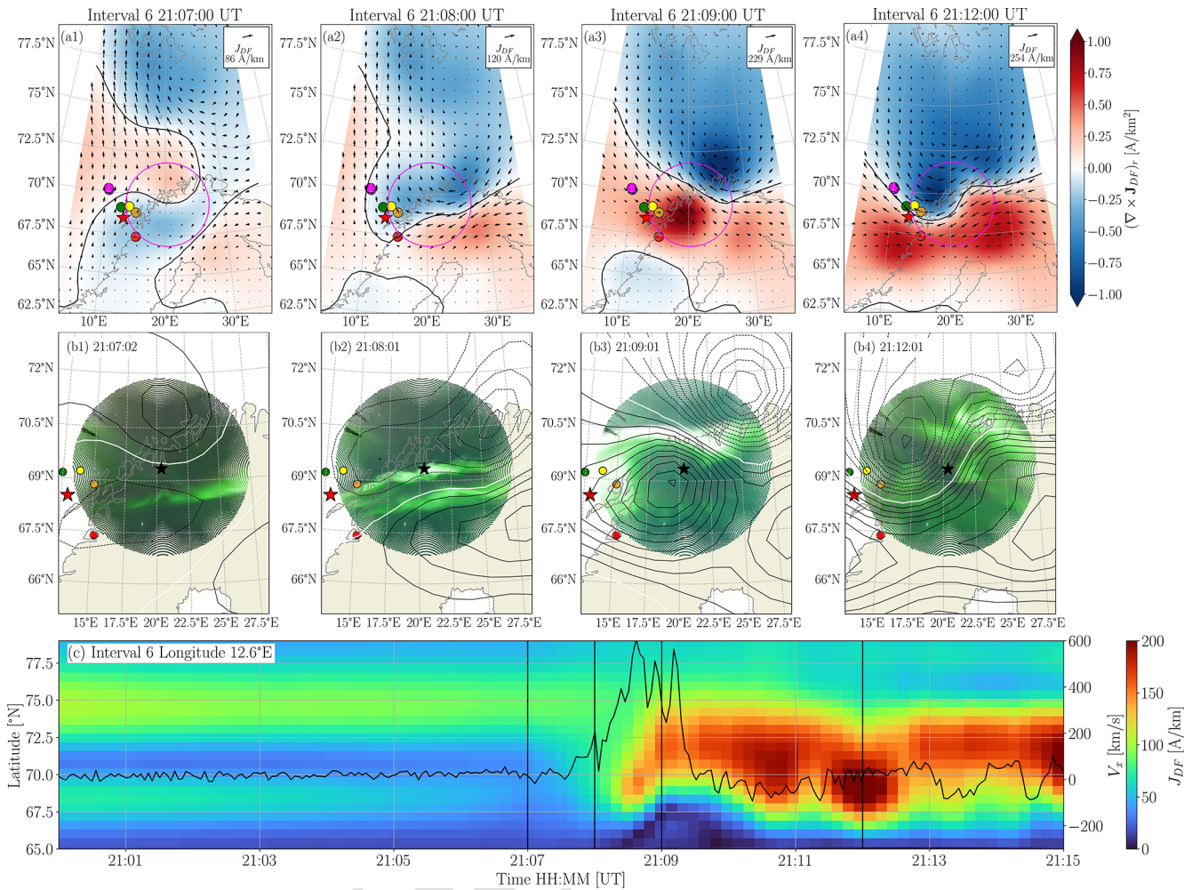
Figure 8. The same as Fig. 5 except for the Interval 6 on 7 December 2023 between 21:00 and 21:15 UT.
