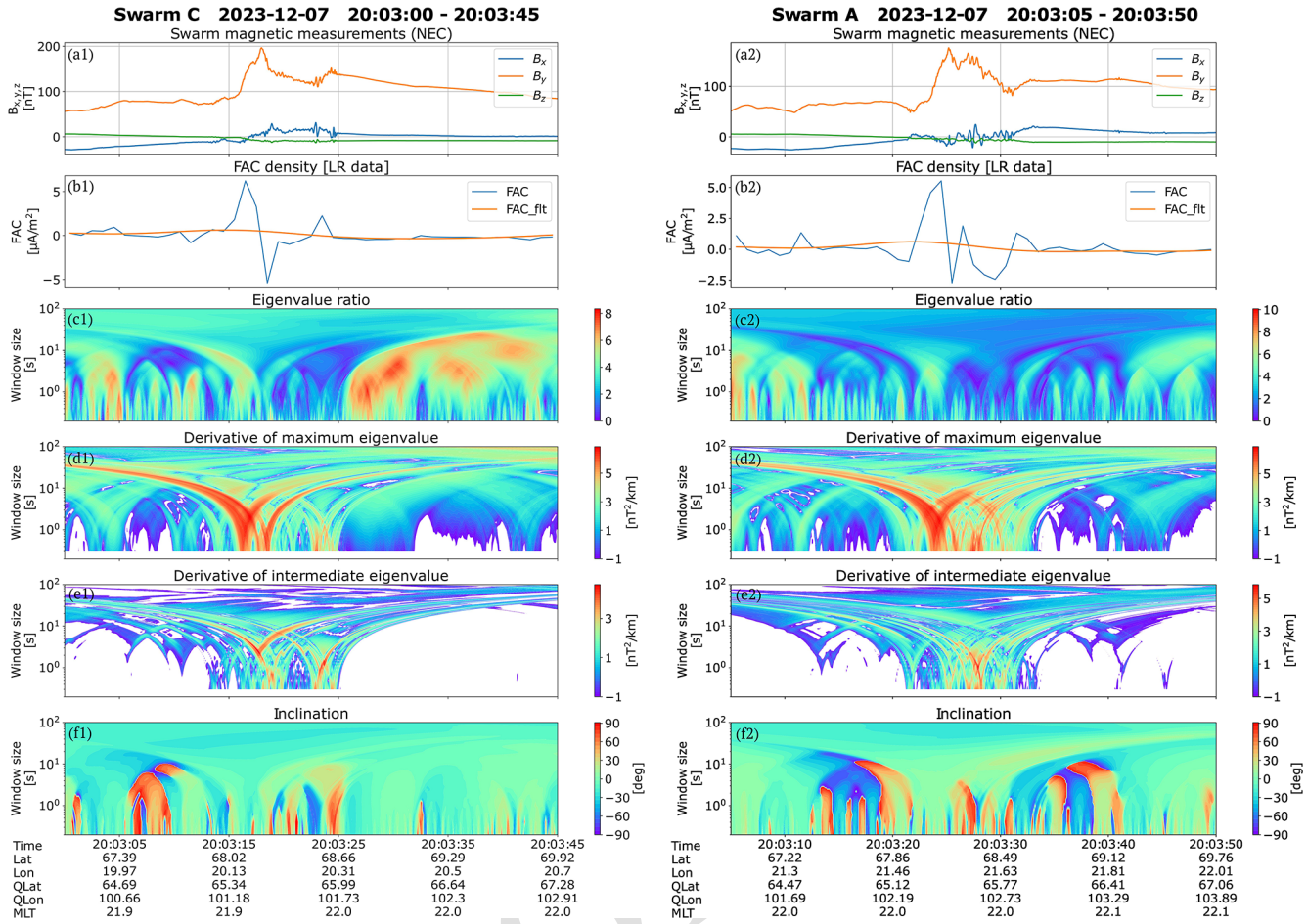
Figure 10. Multi-scale minimum variance analysis of Swarm C (left) and Swarm A (right) FAC data on 7 December 2023 20:03:00–20:03:50 UT. (a) Magnetic field perturbation, (b) single spacecraft current density, (c) eigenvalue ratio, (d, e) derivative of the maximum/intermediate eigenvalue with respect to the width of the sliding window, and (f) inclination with respect to east–west direction.
