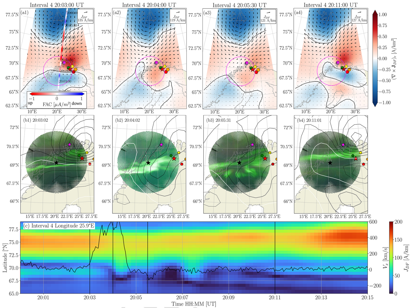
Figure 6. The same as Fig. 5 except for the Interval 4 on 7 December 2023 between 20:00 and 20:15 UT. Panel (a) at 20:03:00 UT includes the Swarm dual spacecraft FACs projected at 110 km altitude. The BBF footpoint centroid and the ASC are displayed as a red and a black star respectively. The BBF footpoint centroid computed from the Tsyganenko models are shown in dots: T89 (red), T96 (orange), T01 (green), and T04 (yellow), TA15n (purple), and TA15b (magenta).
