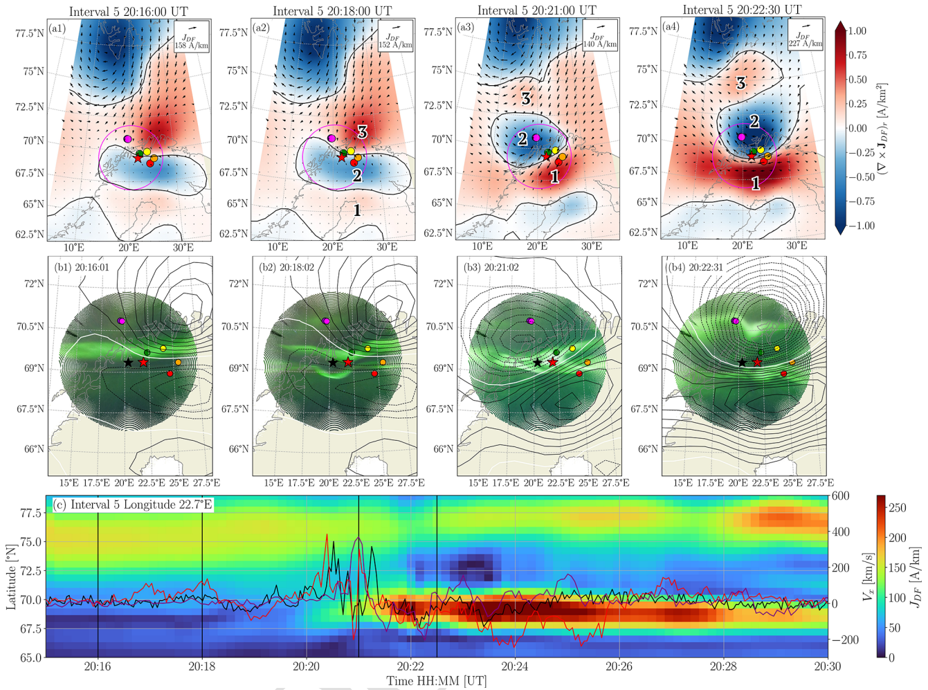
Figure 7. The same as Fig. 5 except for the Interval 5 on 7 December 2023 between 20:15 and 20:30 UT. Panel (c) shows measurements done by THEMIS-A (black), THEMIS-D (red), and THEMIS-E (purple).
