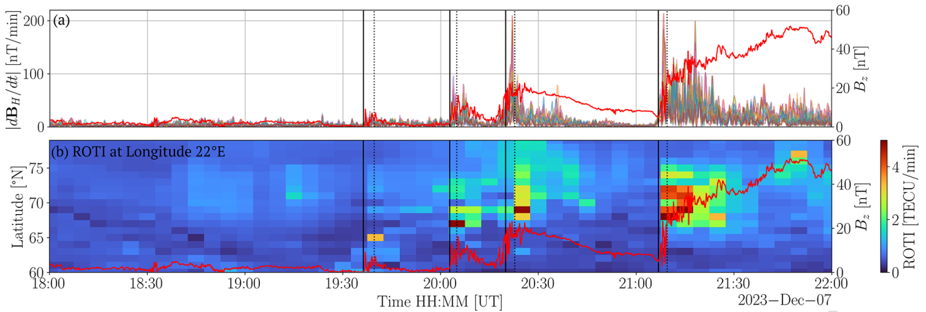
Figure 12. Space weather response to the dipolarization. (a) Ground magnetic field perturbation |dB_H/dt| for each station shown in Fig. 4b, together with the B_z observations by THEMIS-D. (b) Keogram of the ROTI, together with the B_z observations by THEMIS-D. The vertical lines indicate the beginning (solid) and end (dashed) times of the four BBFs intervals listed in Table 1.
