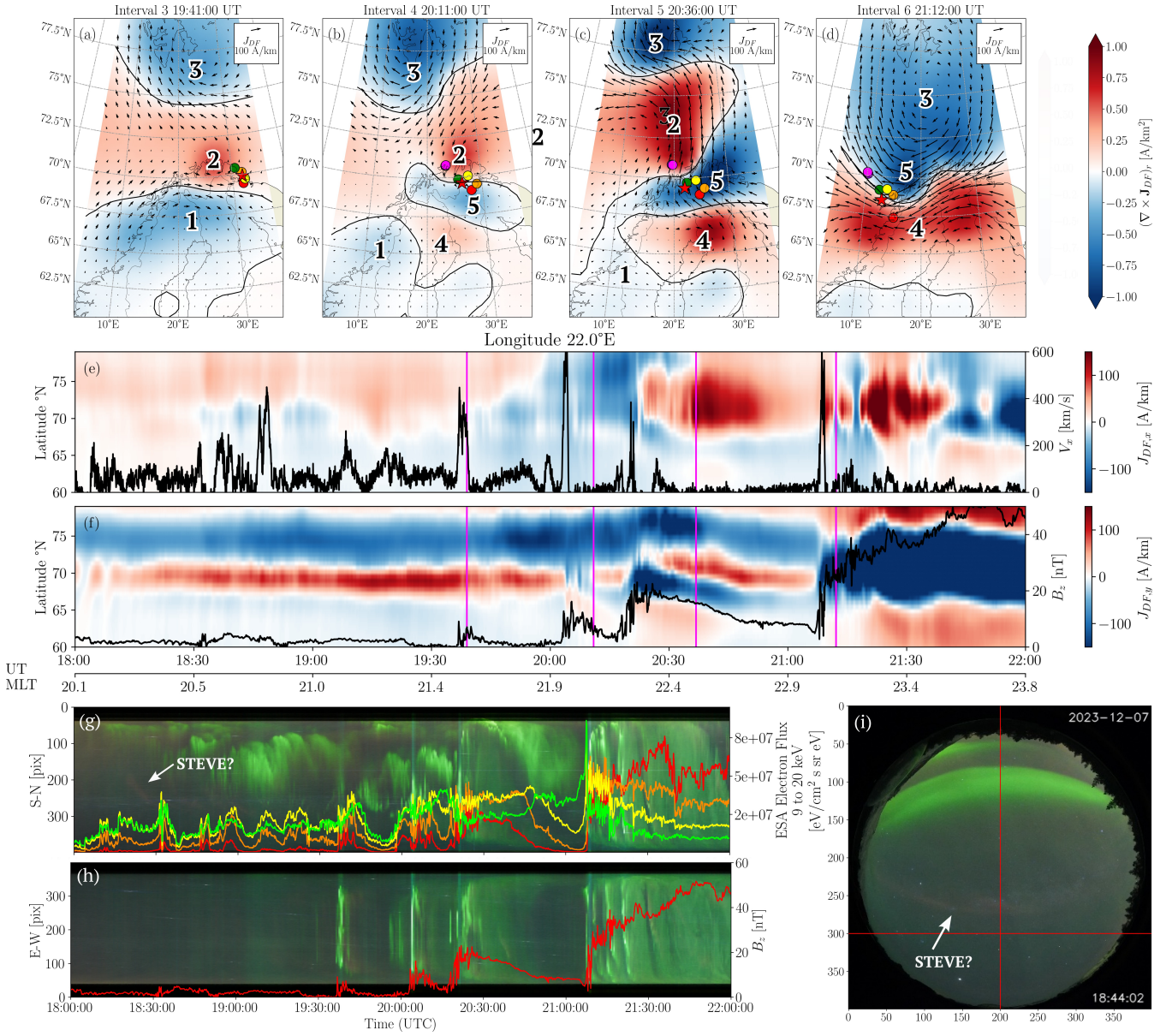
Figure 11. Overview of the interval on 7 December 2023 between 18:00 and 22:00 UT, during which six BBFs were detected by THEMIS-D; the last four were accompanied by clear dipolarization signatures. (a-d) Horizontal ionospheric equivalent current density ( \mathbf{J}_{DF} ) magnitude and direction (arrows), its vorticity ( \nabla \times \mathbf{J}_{DF} ) r (shaded), with counterclockwise (red) and clockwise values (blue). The red star marks the BBF footpoint centroid computed from the Tsyganenko models, shown in dots: T89 (red), T96 (orange), T01 (green), and T04 (yellow), TA15n (purple), and TA15b (magenta). (e) Keogram of the north–south current component J_{DF,x} , together with THEMIS-D V_x used for BBF identification. (f) Keogram of the east–west component J_{DF,y} , shown with THEMIS-D B_z to indicate dipolarization. (g) Keogram of the Skibotn auroral images along the central longitude (pix 200), together with THEMIS-D observations of electron flux. (h) Keogram along the latitude cut southward from the Skibotn location (pix 300), together with THEMIS-D B_z . (i) ASC image showing the longitudinal and latitudinal cuts used in panels (g) and (h).
