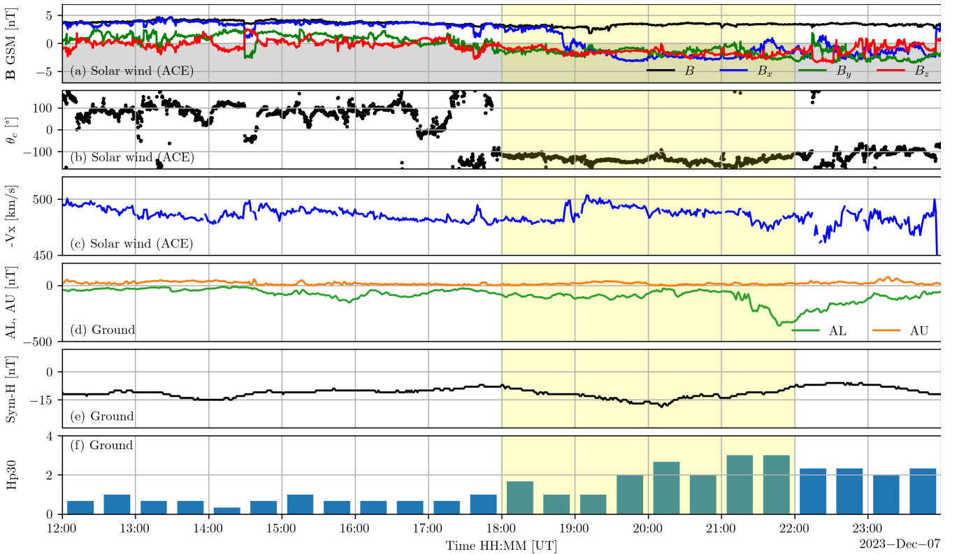
Figure 2. Overview of the 7 December 2023 event between 12:00 and 23:59 UT. (a-c) Solar wind observations from ACE spacecraft (no time-shift): (a) interplanetary magnetic field components in GSM coordinates, (b) IMF clock angle, and (c) solar wind speed. (d-e) Ground geomagnetic response: auroral electrojet index AL (green) and AU (orange), and Sym-H index (black). (f) Hp30 geomagnetic index. The yellow shaded interval marks the period during which several earthward BBFs were detected in the magnetotail.
