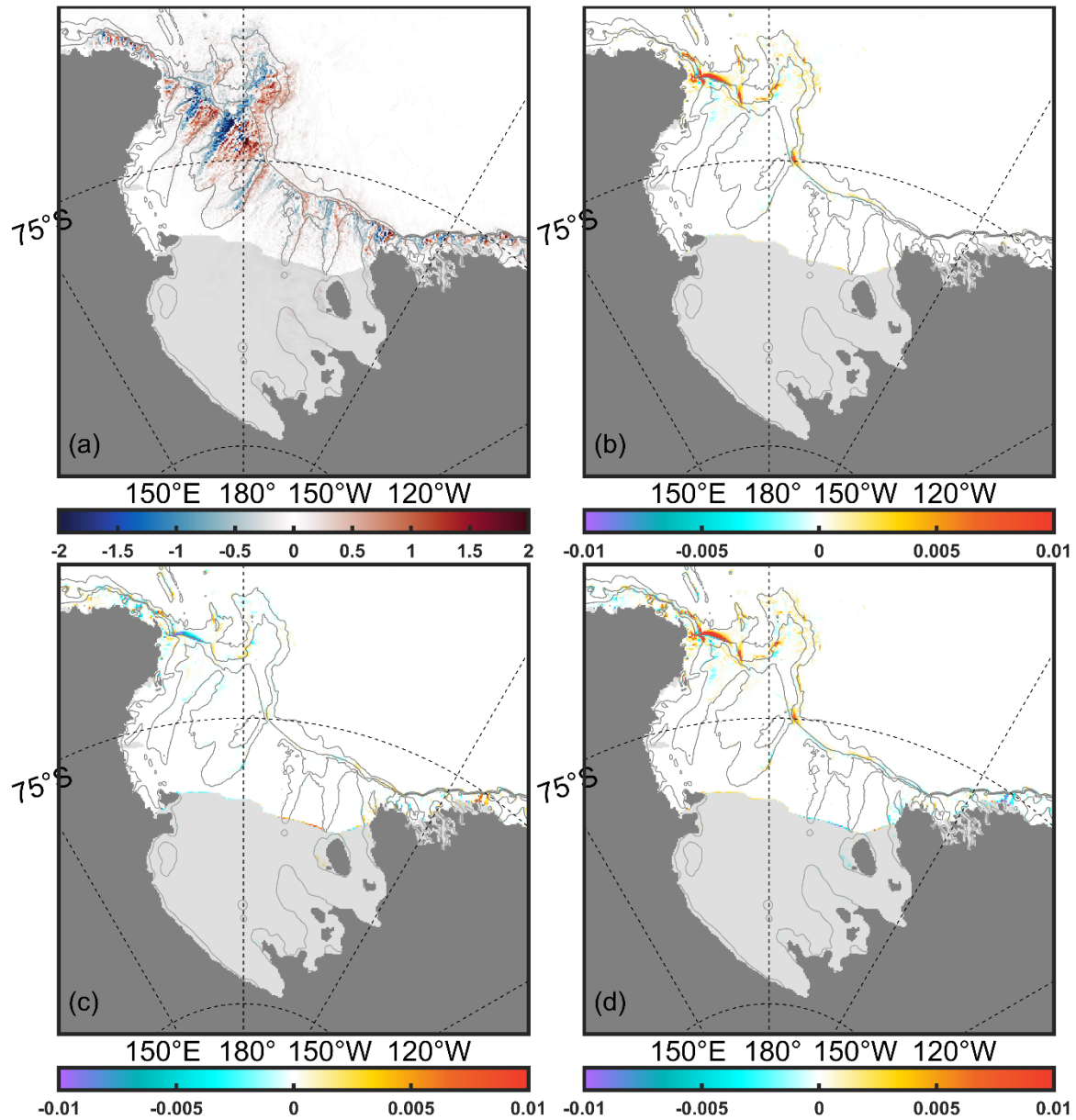
Figure 11. The rate of energy conversion ( \text{W/m}^2 ) from (a) Surface mode to Topographic mode, (b) Barotropic (Surface + Topographic modes) tides to baroclinic tides, (c) Topographic mode to baroclinic tides, and (d) Surface mode to baroclinic tides. Bathymetry contours are spaced at 500, 1000, and 2000 m.
