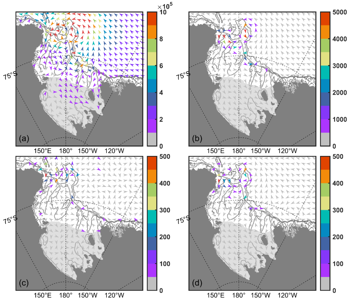
Figure 13. Depth-integrated energy flux (W/m) components (snapshots at high tide): (a) barotropic pressure work, (b) barotropic advective work, (c) baroclinic pressure work, and (d) baroclinic advective work.
