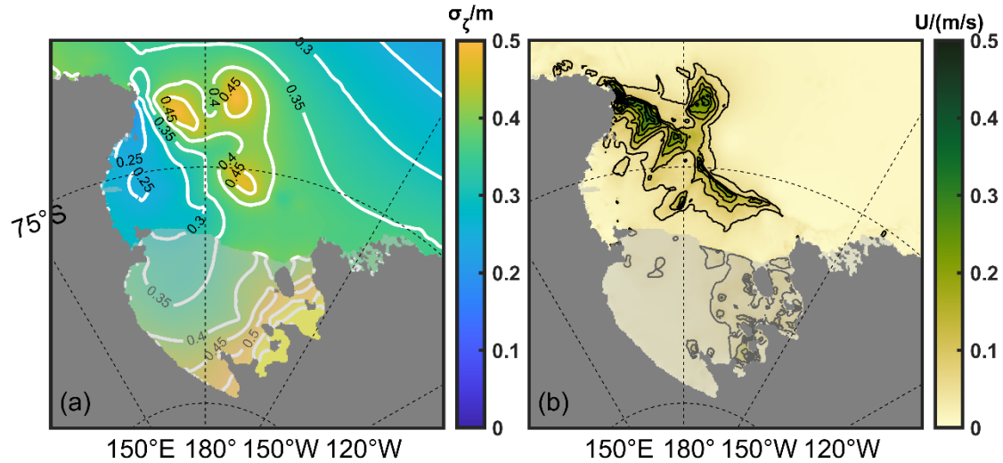
145 Figure 2. Spatial patterns of tidal characteristics calculated by definitions from Padman et al. (2002, 2003): (a) Root-sum-square of tidal harmonic amplitude \sigma_{\zeta} = \sqrt{\sum a_i^2} (m), where a_i is the amplitude of the i -th tidal harmonic and (b) Time-averaged tidal flow speed (m/s).
