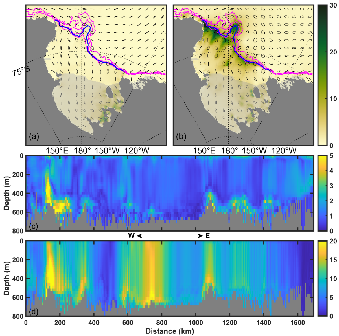
Figure 65. (a, b) Tidal ellipses for M_2 and K_1 . Ellipse major axes are normalized; color shading shows actual speed (cm/s). The 500, 1000, and 2000-m isobaths (magenta) and the 700-m isobath (blue) are shown along the continental slope. (c, d) Vertical section of the mean amplitude of cross-slope tidal flow speed (cm/s) for the semidiurnal and diurnal constituents along the 700 m isobath.
