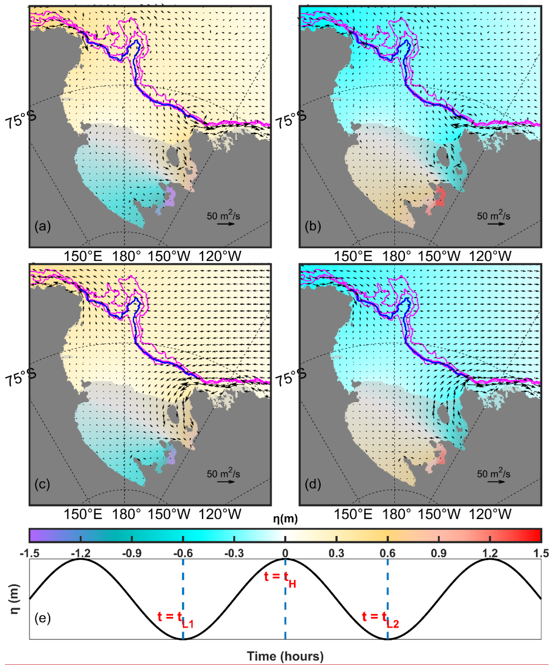
355 Figure 87. Same as Fig. 76, but for semi-diurnal tides.
