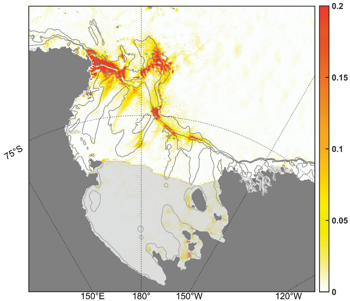
Figure 1413. Map of the depth-integrated, period-averaged tidal dissipation rate ( \text{W/m}^2 ). Bathymetry contours are spaced at 500, 1000, and 2000 m.
