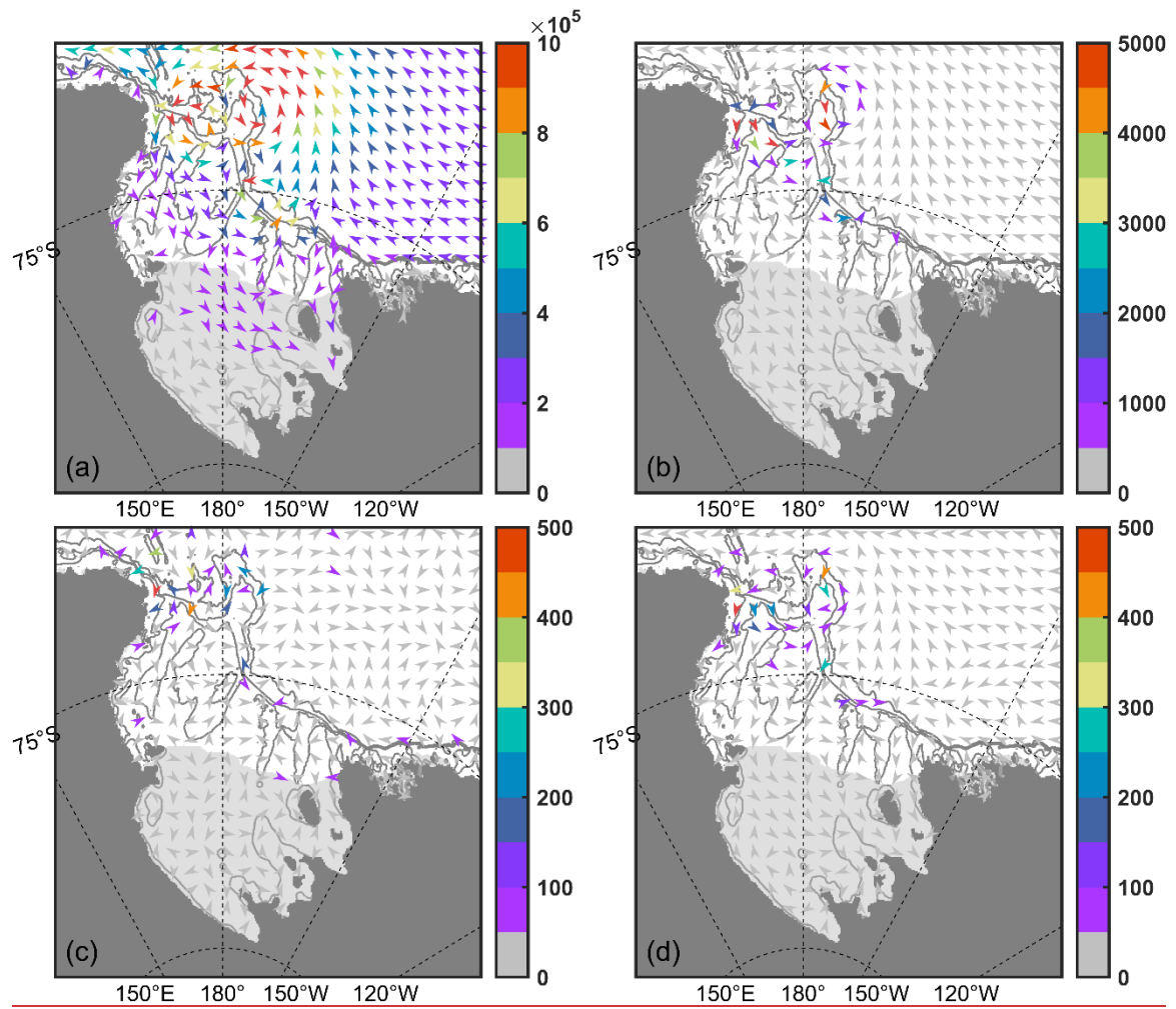
515 Figure 1342. Depth-integrated energy flux (W/m) components (snapshots at high tide): (a) barotropic pressure work, (b) barotropic advective work, (c) baroclinic pressure work, and (d) baroclinic advective work.
