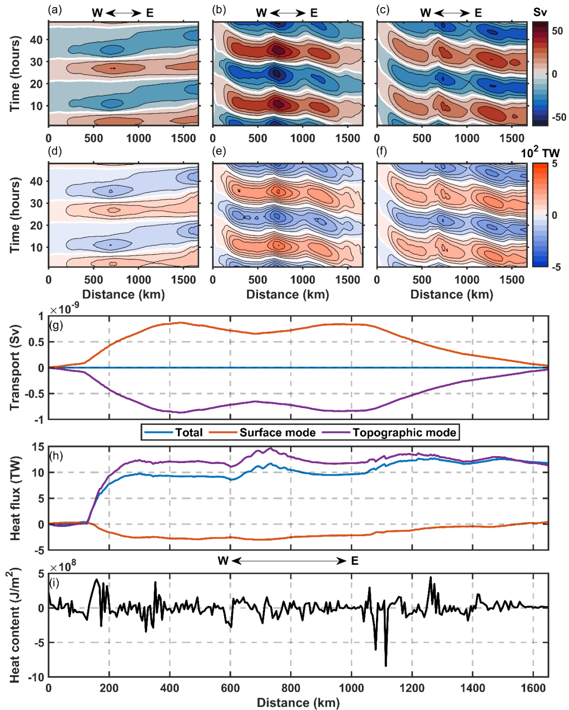
Figure 98. (a-c) Cross-slope volume transport integrated along the 700-m isobath as a function of time for (a) the surface mode, (b) the topographic mode, and (c) their sum. (d-f) The corresponding heat transport. (g, h) The temporal averages of the volume and heat transport, respectively. Positive (negative) values indicate onshore (offshore) transport. (i) Flood-minus-ebb heat content difference.
