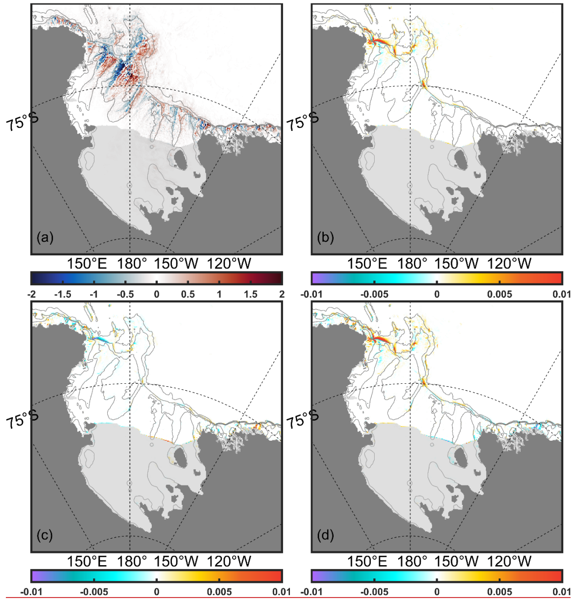
Figure 1140. The rate of energy conversion ( \text{W/m}^2 ) from (a) Surface mode to Topographic mode, (b) Barotropic (Surface + Topographic modes) tides to baroclinic tides, (c) Topographic mode to baroclinic tides, and (d) Surface mode to baroclinic tides. Bathymetry contours are spaced at 500, 1000, and 2000 m.
