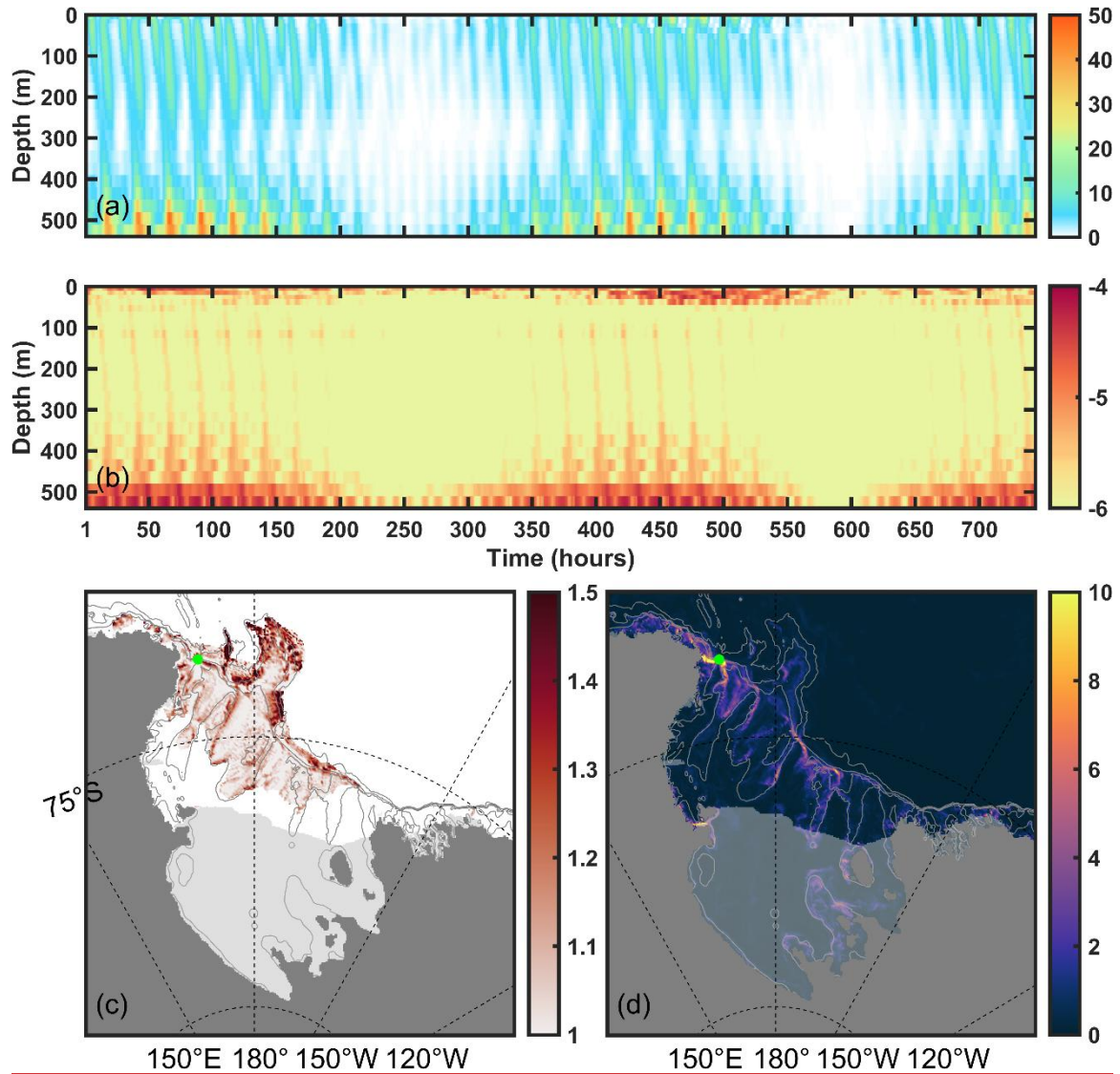
Figure 910. Time-depth plot of the (a) baroclinic kinetic energy density ( \text{J/m}^3 ) and (b) common logarithm of square of the vertical shear of tidal velocity \log_{10} \left( \left( \frac{\partial u}{\partial z} \right)^2 + \left( \frac{\partial v}{\partial z} \right)^2 \right) ( \text{s}^{-2} ) at the point marked by green dots in panels (c, d) (close to mooring cc1) from the model simulation. (c) Map of the ratio of the near-bottom-averaged kinetic energy to the column-averaged kinetic energy ( R_{KE} ). (d) Map of the maximum vertical displacement (m) of time-averaged density at the bottom of each water column. Bathymetry contours are spaced at 500, 1000, and 2000 m.
