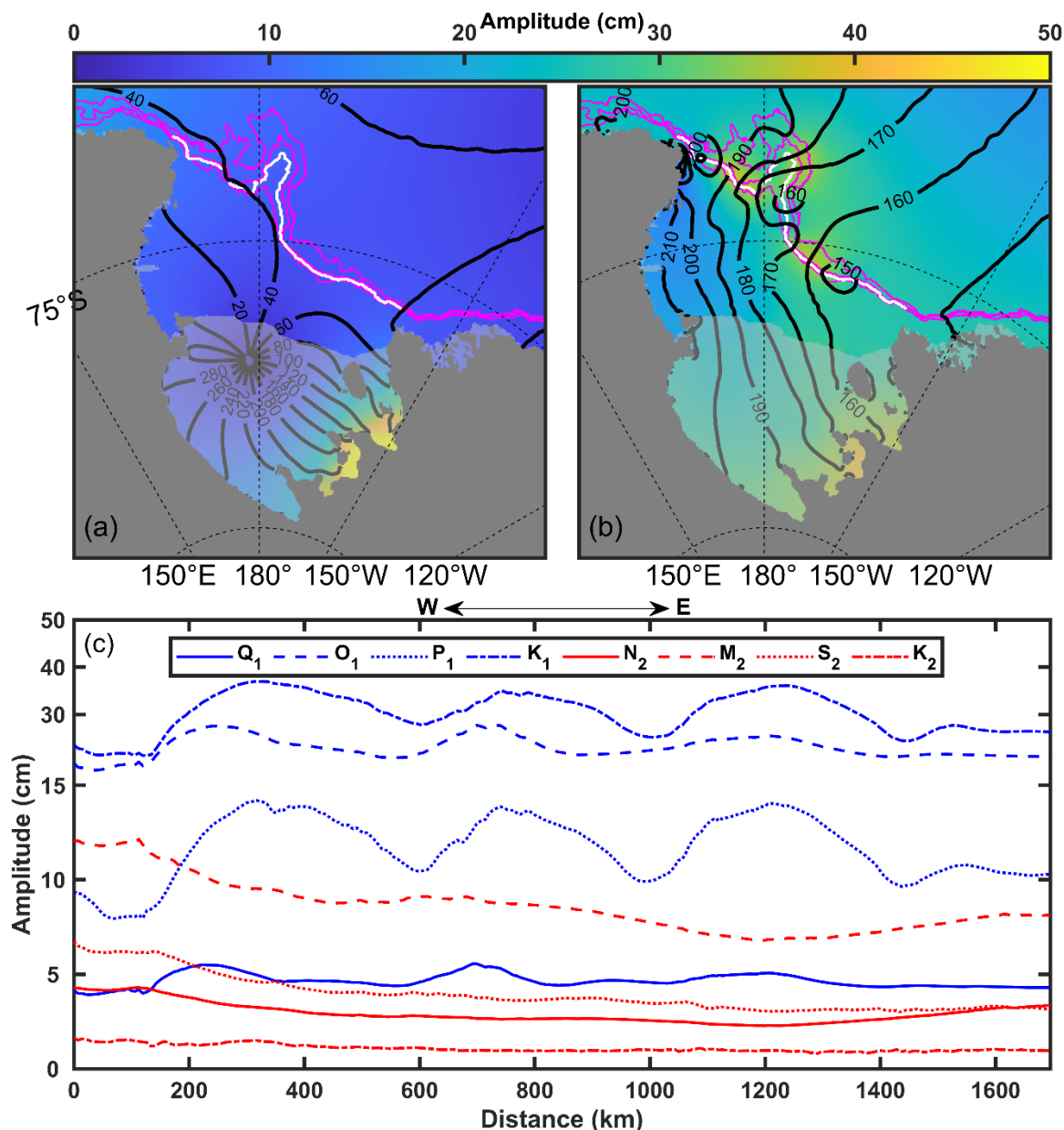
Figure 54. The cotidal charts of (a) M_2 and (b) K_1 tidal constituents from the model simulation. The co-phase lines are shown as black lines. The 500, 1000, and 2000-m isobaths (magenta) and the 700-m isobath (white) are shown along the continental slope. (c) The amplitude of individual constituents along the 700-m isobath.
