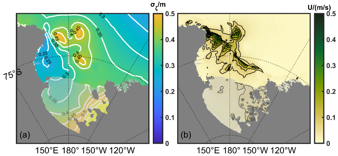
Figure 2. Spatial patterns of tidal characteristics calculated by definitions from Padman et al. (2002, 2003): (a) Root-sum-square of tidal harmonic amplitude \sigma_\zeta = \sqrt{\sum a_i^2} (m), where a_i is the amplitude of the i -th tidal harmonic and (b) Time-averaged tidal flow speed \langle |u| \rangle (m/s), where angle brackets denote time averaging.
