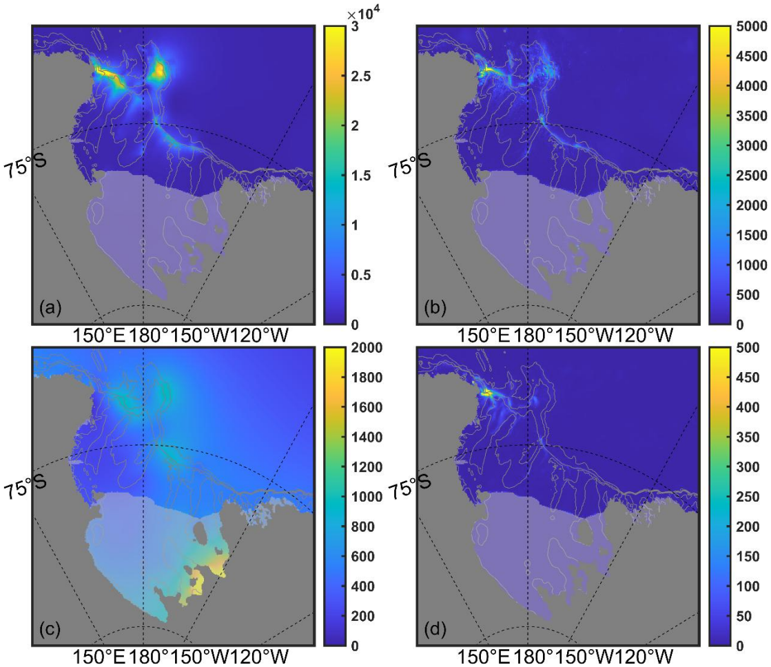
Figure 1244. Spatial distribution of depth-integrated, period-averaged (a) barotropic kinetic energy density ( \text{J/m}^2 ), (b) baroclinic kinetic energy density ( \text{J/m}^2 ), (c) barotropic potential energy density ( \text{J/m}^2 ), and (d) available potential energy density ( \text{J/m}^2 ). Bathymetry contours are spaced at 500, 1000, and 2000 m.
