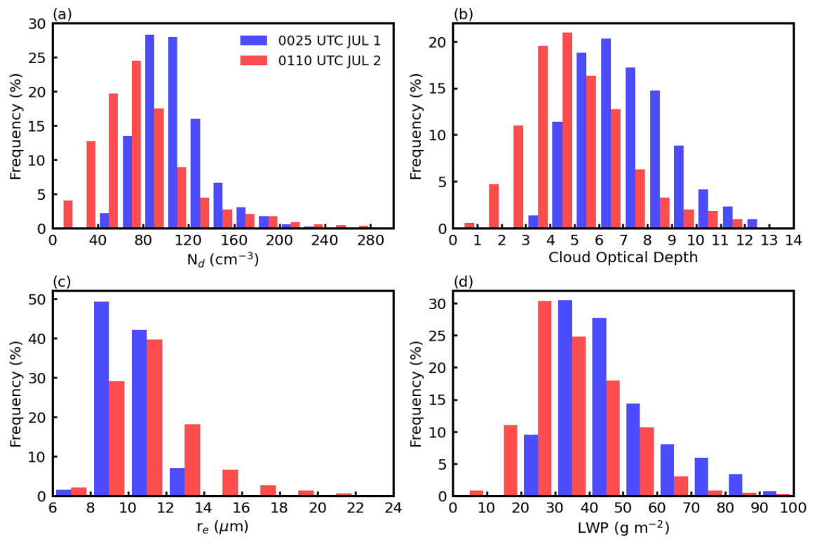
2 3 Figure S1. Frequency distributions (%) of fog properties retrieved from MODIS within the boxed regions 4 shown in Figs. 3a and 3c at 00:25 UTC on July 1 and in Figs. 3b and 3d at 01:10 UTC on July 2: (a) fog 5 droplet number concentration ( \text{cm}^{-3} ), (b) cloud optical depth, (c) effective radius ( \mu\text{m} ), and (d) liquid water 6 path ( \text{g m}^{-2} ). Blue bars indicate July 1, and red bars indicate July 2.
