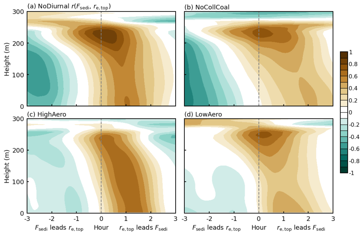
Figure S3. As in Fig. 9 but for the: (a) NoDiurnal, (b) NoCollCoal, (c) HighAero, and (d) LowAero experiments.
