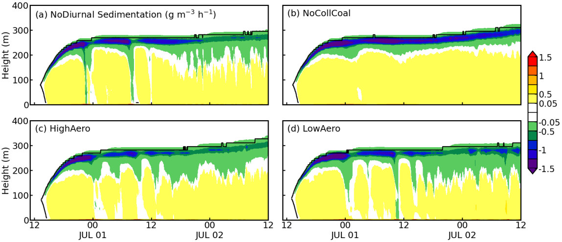
Figure S2. As in Fig. 10d but for the: (a) NoDiurnal, (b) NoCollCoal, (c) HighAero, and (d) LowAero experiments.
