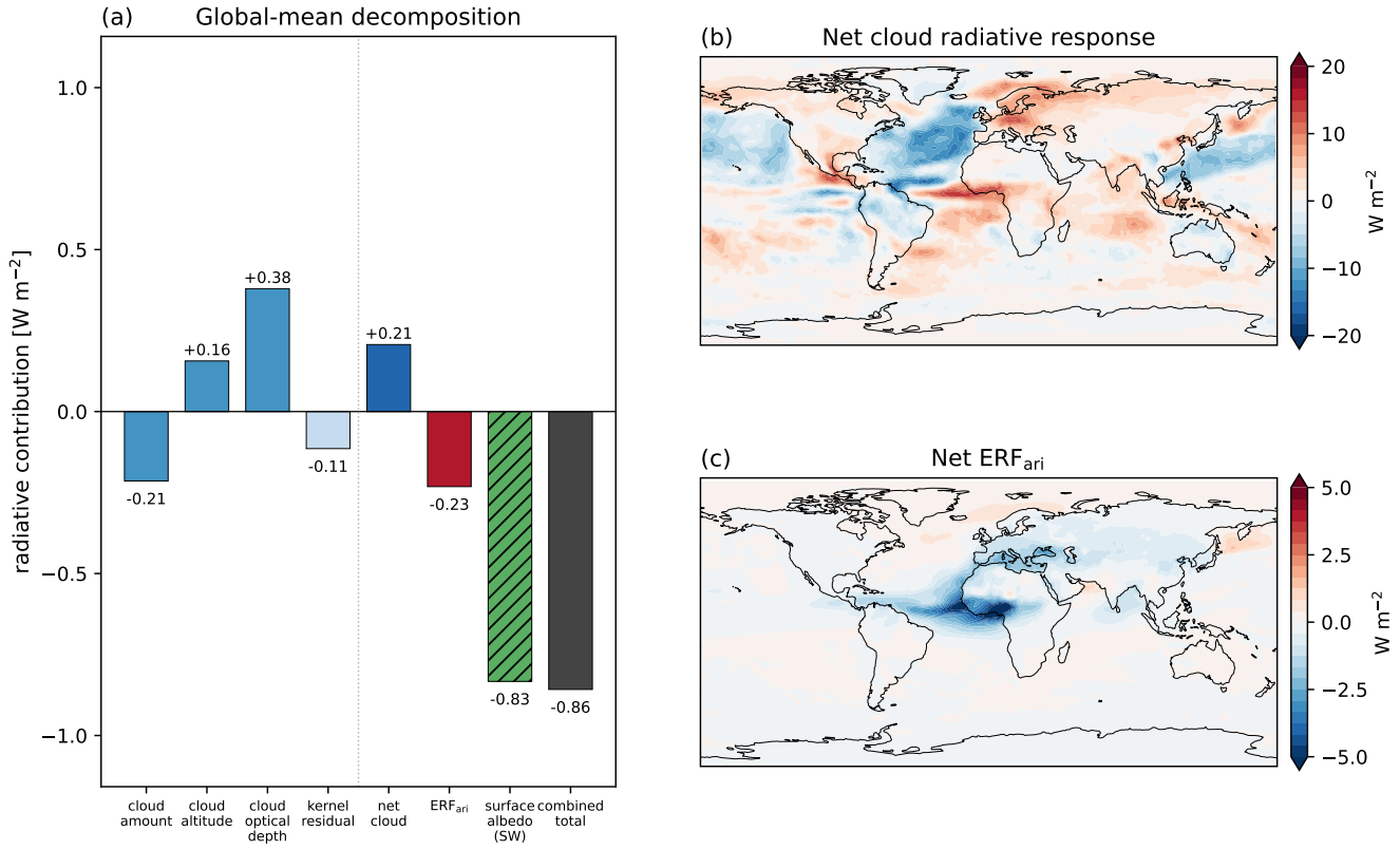
Figure 9. Kernel-corrected decomposition of the top-of-atmosphere radiative response to AMOC weakening (Hosing – Control). (a) Global mean cloud radiative response decomposed into cloud amount, cloud altitude and cloud optical depth components and the kernel decomposition residual, shown alongside the net effective radiative forcing due to aerosol–radiation interactions ( \text{ERF}_{\text{ari}} ), the surface albedo term (shortwave only), and their combined total. (b) Map of the net cloud radiative response. (c) Map of the net \text{ERF}_{\text{ari}} .
