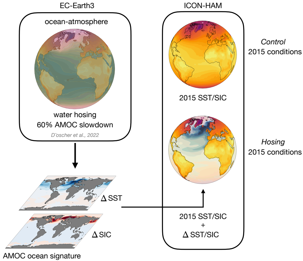
Figure 1. Schematic overview of the experimental design. Anomalies in sea surface temperature ( \Delta SST ) and sea ice concentration ( \Delta SIC ) are derived from a fully coupled EC-Earth3 freshwater-hosing simulation that produces an approximately 60 % reduction in AMOC strength. These ocean surface anomalies are superimposed on the present-day (2015) SST and SIC climatology to force the Hosing experiment, while the Control simulation uses the unperturbed climatology. In both ICON-HAM simulations, only the ocean surface conditions are prescribed, whereas the atmosphere and the land surface temperature evolve freely in response to the imposed ocean state, together with the interactive dust and sea salt emissions. The land runs in the jsbach_lite configuration, with vegetation phenology and albedo held at climatology. Adapted from Vella et al. (2026).
