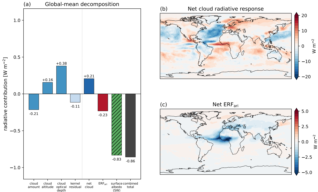
Figure 9. Kernel-corrected decomposition of the top-of-atmosphere radiative response to AMOC weakening (Hosing – Control). (a) Global mean cloud radiative adjustment response decomposed into cloud amount, cloud altitude and cloud optical depth components and the kernel decomposition residual, shown alongside the net aerosol-direct-effective radiative effect-forcing due to aerosol-radiation interactions ( \text{DREERF}_{\text{ari}} ), the surface albedo term (shortwave only), and their combined total. (b) Map of the net cloud radiative adjustment response . (c) Map of the net aerosol-DRE anomaly \text{ERF}_{\text{ari}} .
