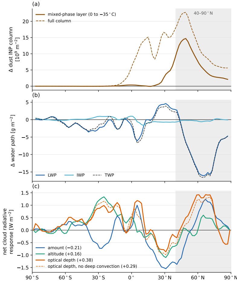
Figure 10. Zonal means (Hosing – Control) of (a) the dust INP column in the mixed-phase layer, where the control annual mean temperature lies between 0 and -35^\circ\text{C} (solid), and over the full column (dashed), (b) liquid, ice and total water path, and (c) the net cloud amount, altitude and optical depth components of the cloud radiative response, with the optical depth component also shown without deep convective clouds (dashed). Global means in \text{W m}^{-2} are given in the legend of (c). Grey shading marks 40–90°N, the region of Fig. 7.
