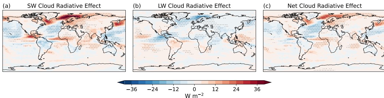
Figure 8. Global maps of the difference (Hosing – Control) in (a) shortwave (SW), (b) longwave (LW), and (c) net cloud radiative effect. Stippling indicates regions where the difference is statistically significant at the 95 % confidence level ( p < 0.05 ).
