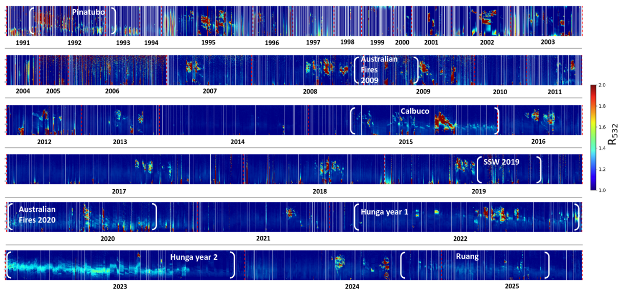
Figure 3. Time series of 532 nm backscatter ratio acquired at DDU between February 1991 and October 2025. The time scale is not linear and depends on the number of available measurements. Each individual profile is integrated over 15 minutes. Dashed red vertical lines delimit the different years. White vertical bands indicate periods where at least one day separates two consecutive measurements. White brackets and labels highlight significant stratospheric perturbations.
