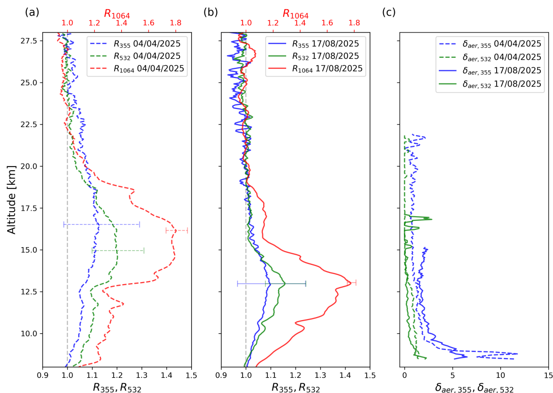
Figure 5. Backscatter ratios R_{355} , R_{532} , R_{1064} (a and b; blue, green, and red, respectively) and depolarization ratios \delta_{aer,355} and \delta_{aer,532} (c; blue and green, respectively) profiles acquired at DDU on 4 April 2025 (dashed lines) and 17 August 2025 (solid lines).
