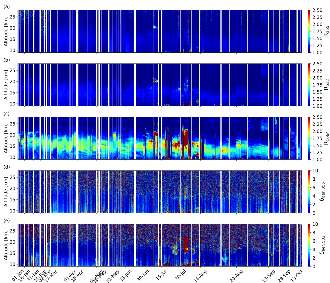
Figure 4. 2025 DDU lidar time series, from top to bottom: backscatter ratios at 355 nm ( R_{355} ), 532 nm ( R_{532} ), 1064 nm ( R_{1064} ), depolarization ratios at 355 nm ( \delta_{aer,355} ) and 532 nm ( \delta_{aer,532} ). The time axis is not linear and depends on the number of available measurements. Each individual profile is integrated over 15 min.
