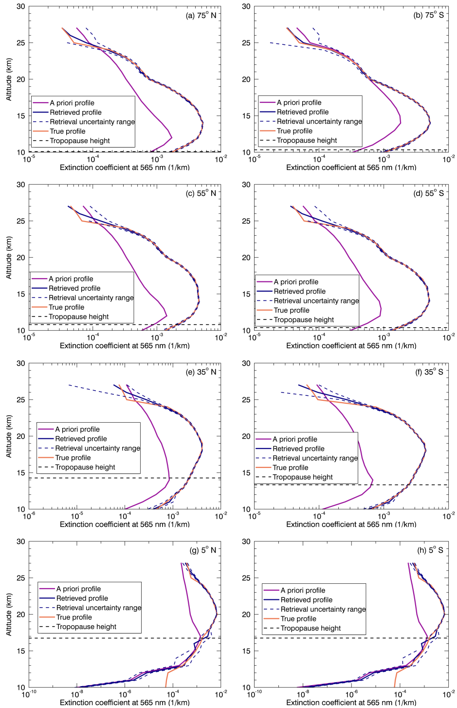
Figure 2. Retrieved extinction coefficient profiles at 565 nm for the injection of 5 \text{ Tg yr}^{-1} alumina including total errors retrieval uncertainties, background profiles ( a priori a priori profiles), and true profiles ( SOCOL-AERv2-model simulation ), and tropopause heights for (a) 75^\circ \text{ N} , (b) 75^\circ \text{ S} , (c) 55^\circ \text{ N} , (d) 55^\circ \text{ S} , (e) 35^\circ \text{ N} , (f) 35^\circ \text{ S} , (g) 5^\circ \text{ N} , and (h) 5^\circ \text{ S} .
