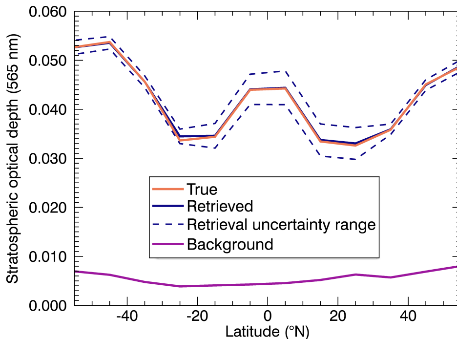
Figure 6. Stratospheric optical depth (565 nm) over as a function of latitude for the injection of 5 Tg yr -1 calcite, including the corresponding total errors: retrieved (blue line), background cases, (purple line) and true profiles (SOCOL-AERv2 model simulations orange line). The retrieval uncertainties are shown by the blue dashed lines.
