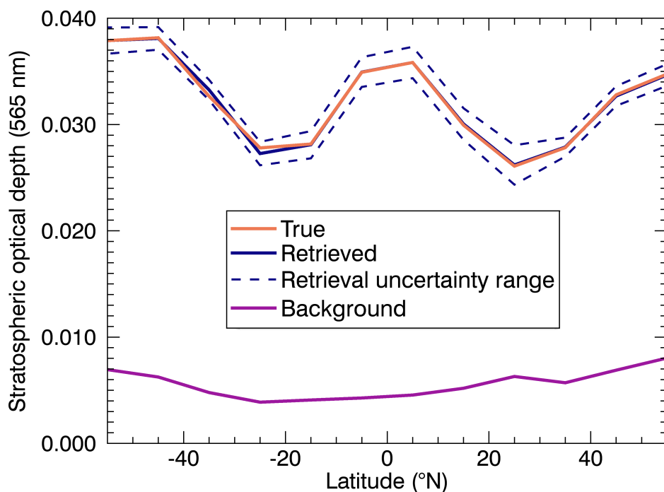
Figure 3. Stratospheric optical depth (565 nm) over as a function of latitude for the injection of 5 Tg yr -1 alumina, including the corresponding total errors: retrieved (blue line), background cases, (purple line) and true profiles (SOCOL-AERv2 model simulations orange line). The retrieval uncertainties are shown by the blue dashed lines.
