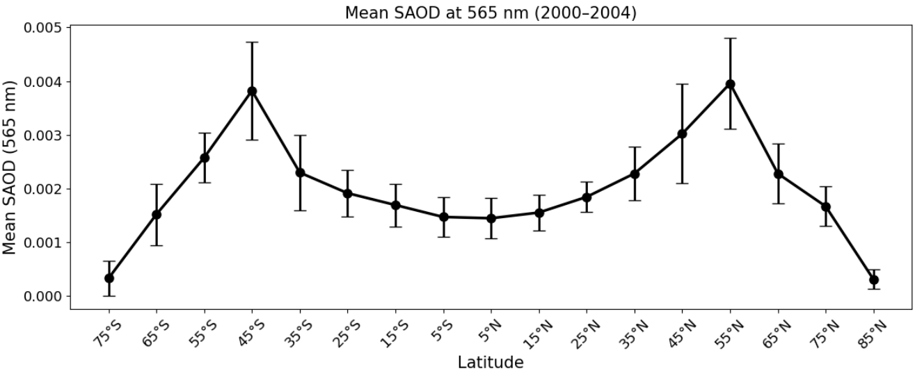
Figure 8. Mean SAOD (565 nm) over as a function of latitude for the SAGE II data from 2000 — 2004. The vertical bars indicate the standard deviation of the SAOD values for each latitude.
