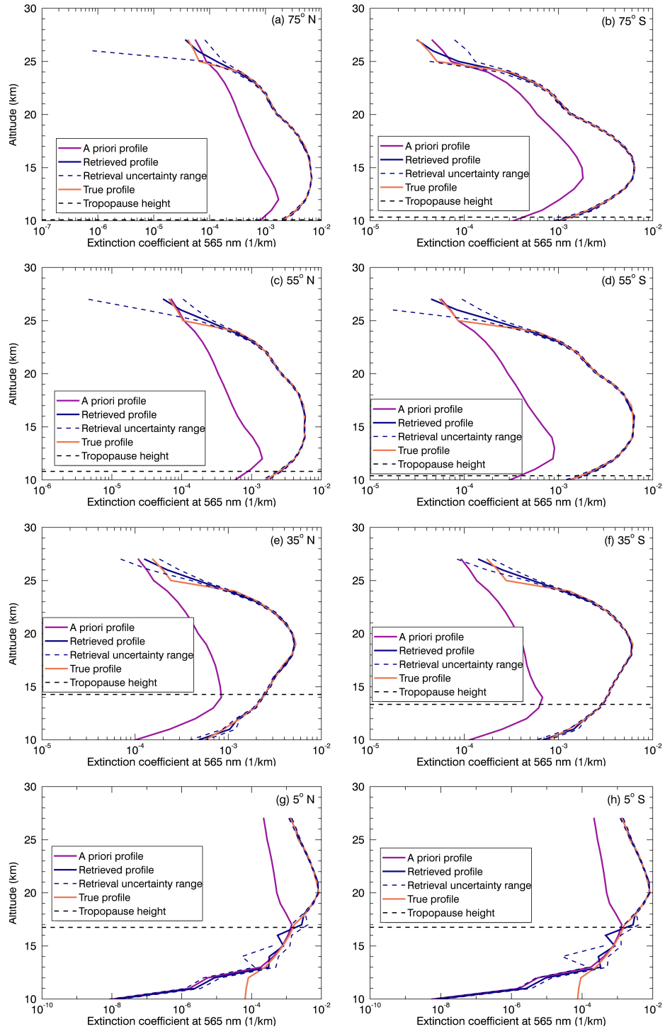
Figure 5. Retrieved extinction coefficient profiles at 565 nm for the injection of 5 \text{ Tg yr}^{-1} calcite including total errors retrieval uncertainties , background profiles ( a priori a priori profiles), and true profiles ( SOCOL-AERv2-model simulation ), and tropopause heights for (a) 75^\circ \text{ N} , (b) 75^\circ \text{ S} , (c) 55^\circ \text{ N} , (d) 55^\circ \text{ S} , (e) 35^\circ \text{ N} , (f) 35^\circ \text{ S} , (g) 5^\circ \text{ N} , and (h) 5^\circ \text{ S} .
