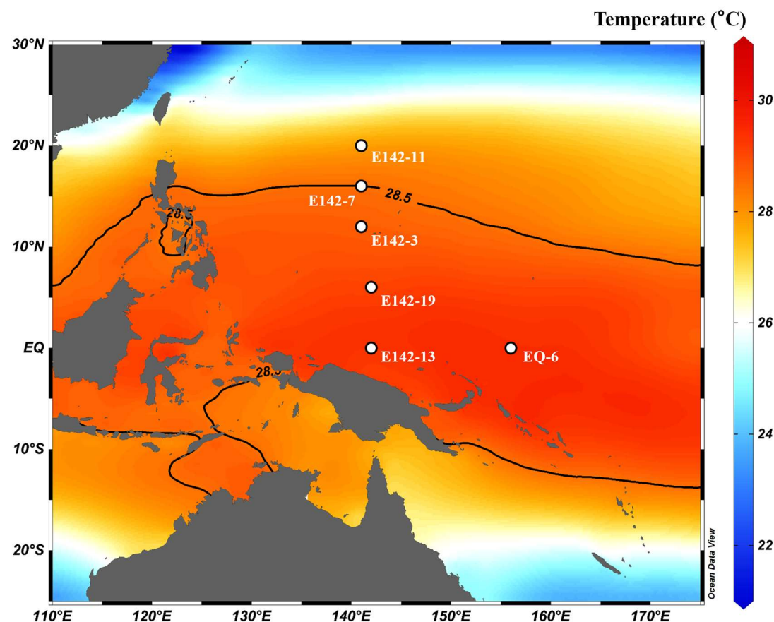
Figure 1. Study area and sampling stations in the Tropical Northwest Pacific. The sampling area is located in the Western Pacific Warm Pool, and the 28.5 °C isotherms are shown as black lines.
