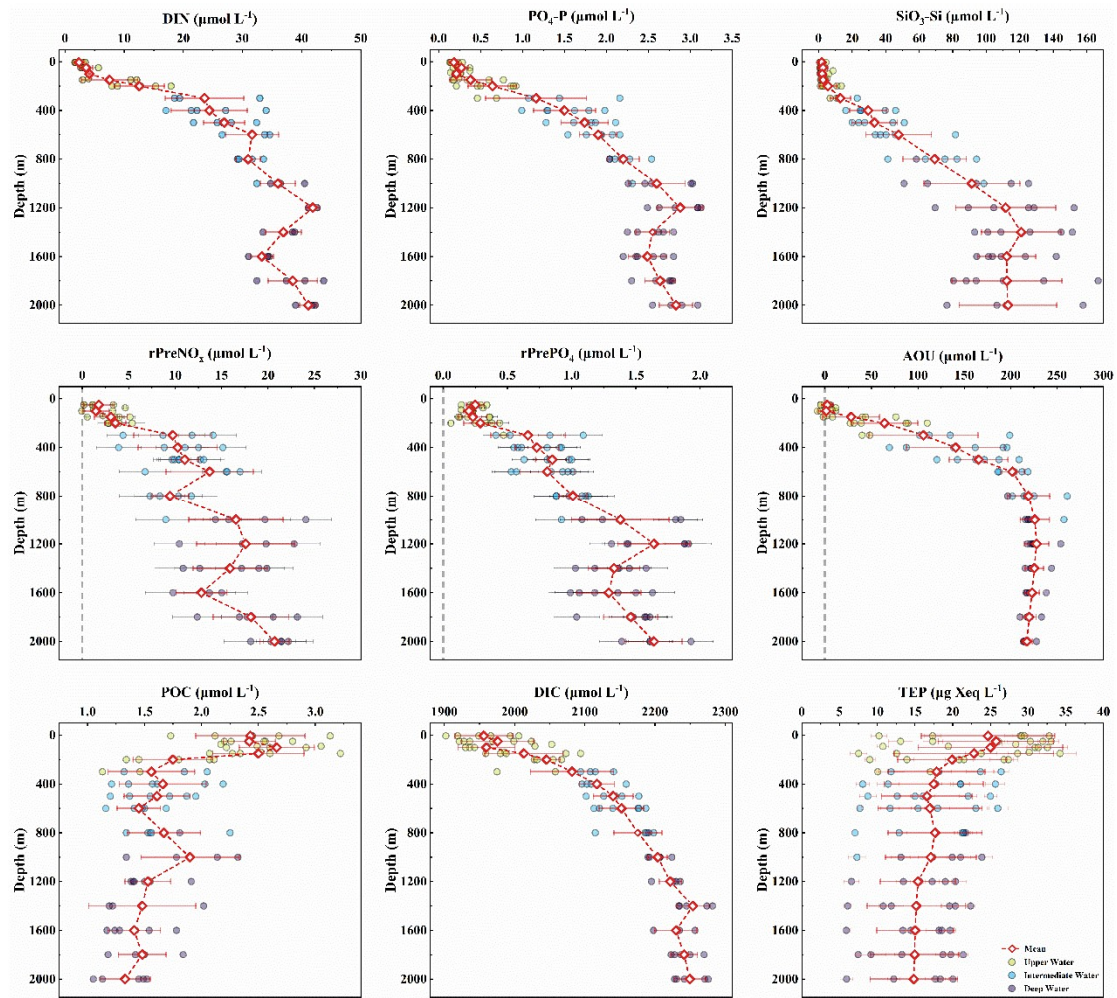
Figure 3. Vertical distributions of chemical and particulate parameters in the water column. Profiles show (a) dissolved inorganic nitrogen (DIN), (b) phosphate (PO 4 -P, as dissolved inorganic phosphorus, DIP), (c) silicate (SiO 3 -Si, as dissolved inorganic silicon, DSi), (d) residual preformed NO x (rPreNO x ), (e) residual preformed phosphate (rPrePO 4 ), (f) apparent oxygen utilization (AOU), (g) particulate organic carbon (POC), (h) dissolved inorganic carbon (DIC), (i) transparent exopolymer particle (TEP). For rPreNO x and rPrePO 4 , each point and its horizontal error bar represent the mean ± standard deviation derived from the 9 parameter combinations for an individual sample. For TEP, each point and its horizontal error bar represent the mean ± standard deviation of triplicate measurements. Red diamonds connected by dashed lines and their horizontal error bars denote the mean ± standard deviation of all samples collected at each nominal sampling depth.
