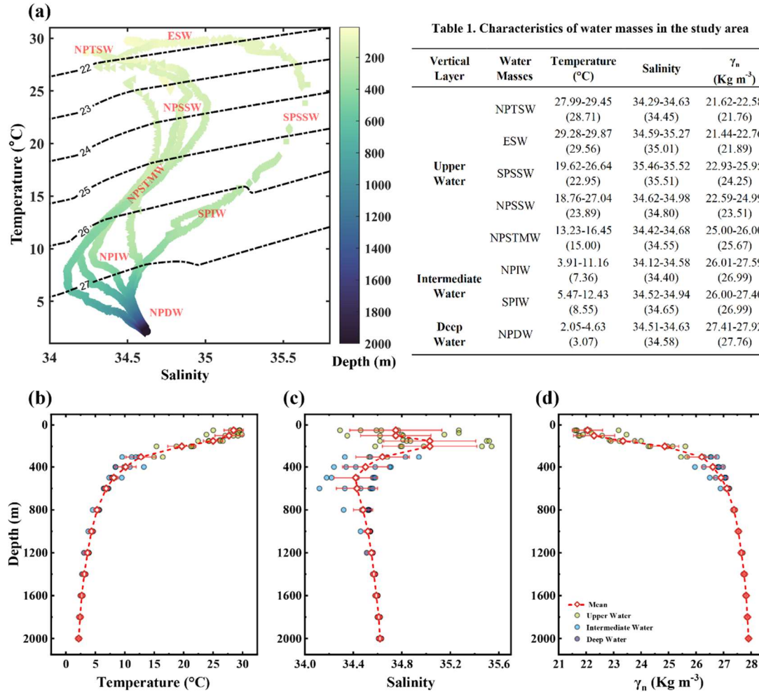
Figure 2. Hydrographic characteristics of the water column. (a) Temperature-salinity diagram of six stations, and the vertical profiles of (b) temperature, (c) salinity, (d) neutral density ( \gamma_n ). Red diamonds connected by dashed lines and their horizontal error bars denote the mean \pm standard deviation of all samples collected at each nominal sampling depth.
