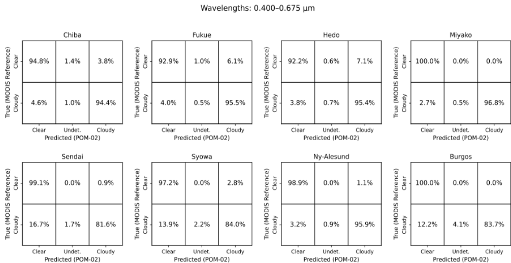
Figure 6. Confusion matrices for clear, undetermined, and cloudy sky discrimination using atmospheric slope ( m_{\text{atm}} ) values determined using 0.400 and 0.675 \mu\text{m} wavelength pair. MODIS cloud-mask classifications are used as the reference, while POM-02 slope-based classifications are treated as predictions. Each matrix is normalized by the MODIS reference class, so that each row sums to 100%.
