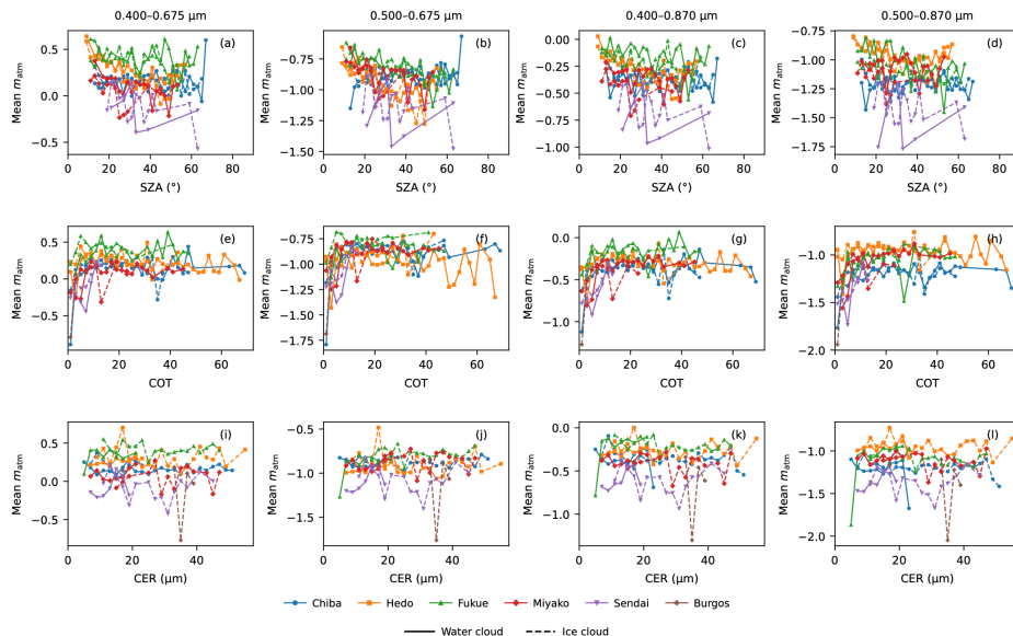
Figure 5. Dependence of mean spectral atmospheric slope ( m_{\text{atm}} ) values on solar zenith angle (SA), cloud optical thickness (COT), and cloud-particle effective radius (CER) under cloudy-sky conditions identified using the reference MODIS cloud mask data. Mean values were calculated at each site using bin intervals of 2^\circ for SA, 2 for COT, and 2 \mu\text{m} for CER.
