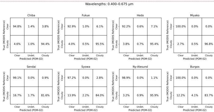
Figure 6. Confusion matrices for clear, undetermined, and cloudy sky discrimination using atmospheric slope ( m_{\text{lim}} ) values determined using 0.400 and 0.675 \mu\text{m} wavelength pair. MODIS cloud-mask classifications are used as the reference, while POM-02 slope-based classifications are treated as predictions. Each matrix is normalized by the MODIS reference class, so that each row sums to 100%.
