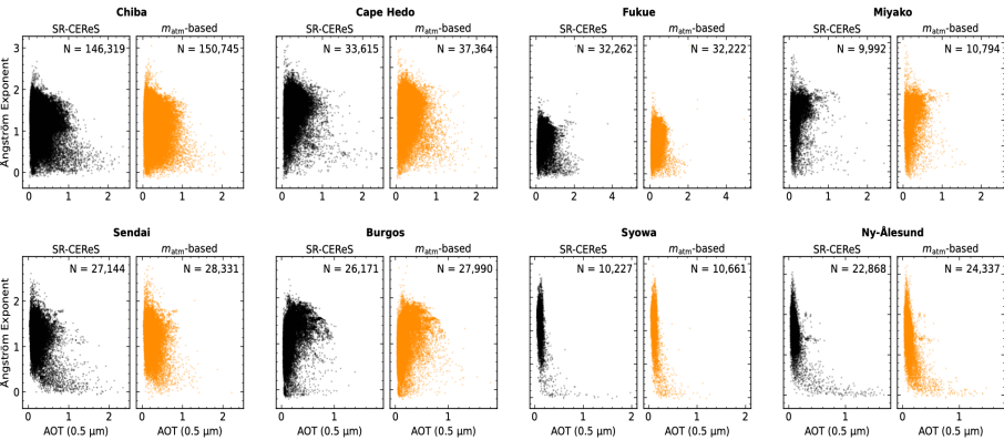
Figure 11. Scatter plots of Ångström exponent (AE) versus aerosol optical thickness (AOT) at 0.5 μm for eight SKYNET sites after cloud screening using two systems: the SR-CEReS package (left panels) and the slope-based method derived from the atmospheric slope of zenith radiance between 0.500 and 0.675 μm with ε value of 0.05 (right panels). Numbers indicate the total observations retained by each method.
