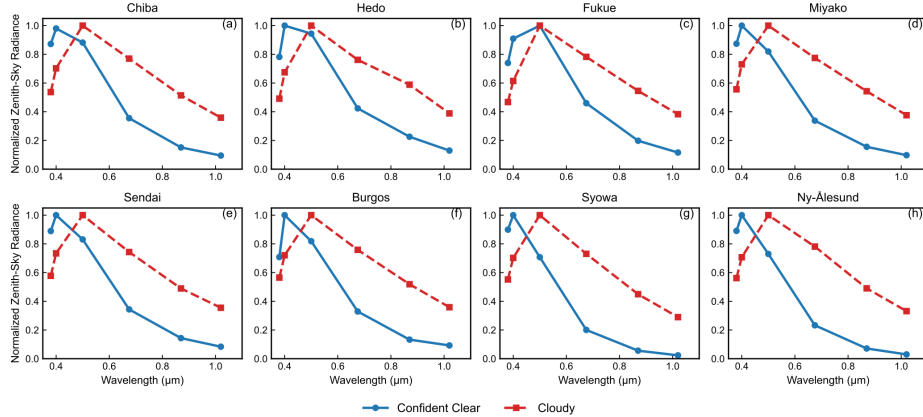
Figure 2. Median normalized spectral zenith sky radiance under cloudy and confidently clear sky conditions at (a) Chiba, (b) Hedo, (c) Fukue, (d) Miyako, (e) Sendai, (f) Burgos, (g) Syowa, and (h) Ny-Ålesund. Zenith sky radiances were normalized
