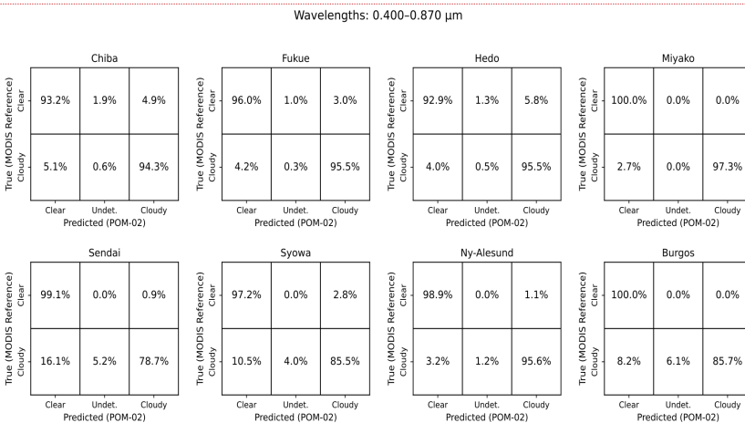
Figure 8. Same as Fig. 6, but for the spectral slope between 0.400 and 0.870 \mu\text{m} .
