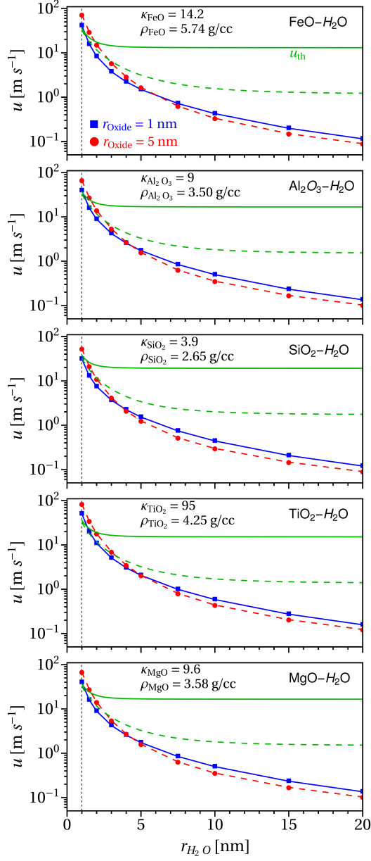
Figure 3. Left Panels: Variation of u_{max} and u_{th} (green) as a function of r_{H_2O} needed for collision between charged ice and various neutral metal oxides. The solid and dashed lines are for r_{Oxide} = 1 nm (blue) and 5 nm (red), respectively. The colors are explained in the uppermost panel. Right Panels: Variation of u_{max} normalized with the same for SiO 2 as a function of r_{H_2O} . Other parameter used: q_{H_2O} = -1e , q_{Oxide} = 0 , \kappa_{H_2O} = 100 and \rho_{H_2O} = 0.92 g/cc.
