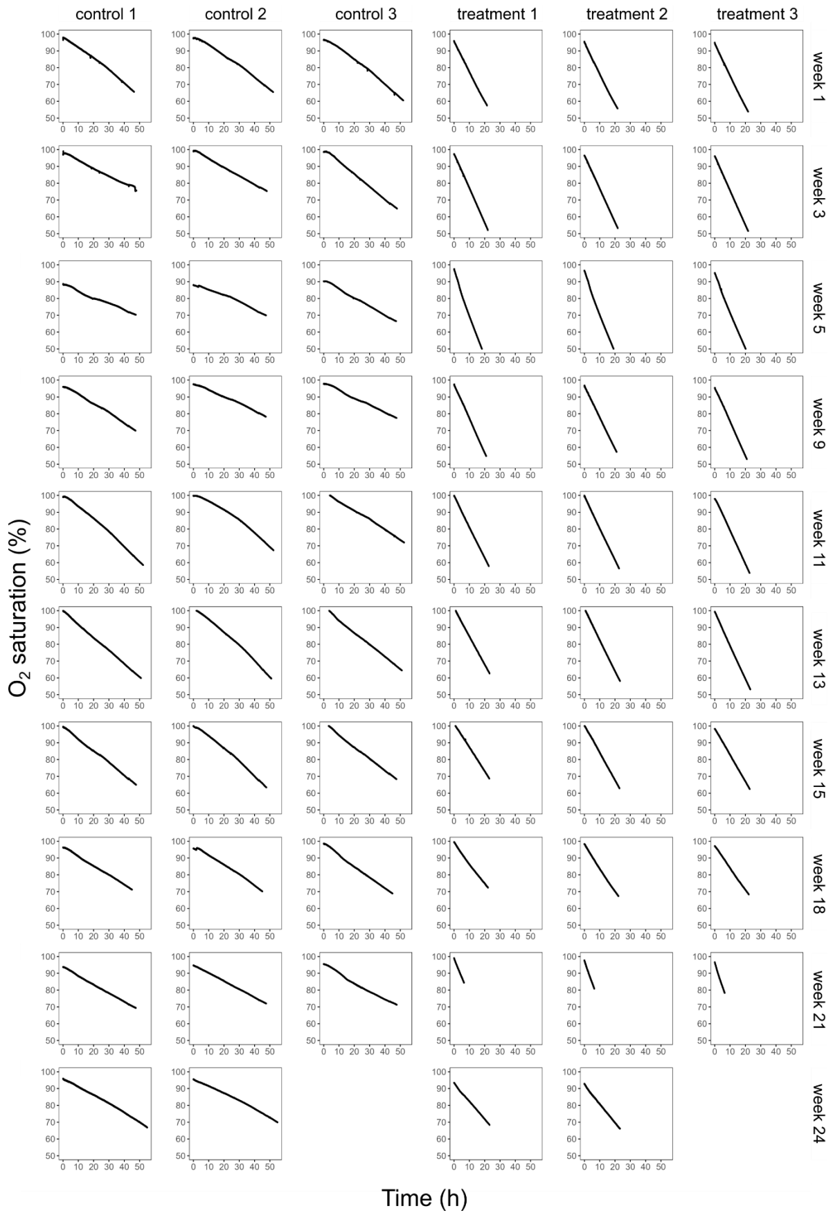
Figure S1: Oxygen (O 2 ) saturation changes versus incubation time, shown for each control and treatment chamber per week.
