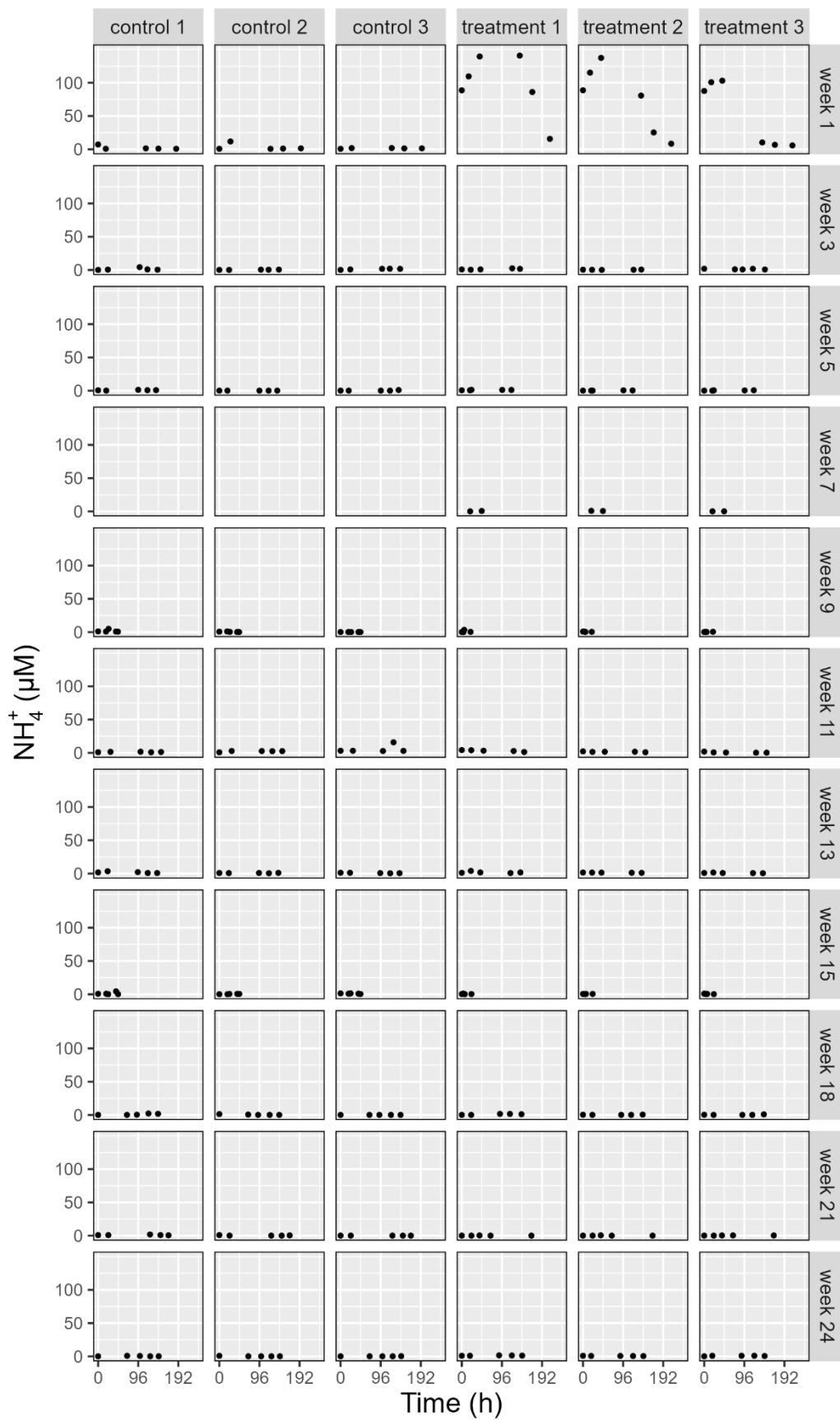
Figure S5: Ammonium (NH 4 + ) concentration changes versus incubation time, shown for each control and treatment chamber per week.
