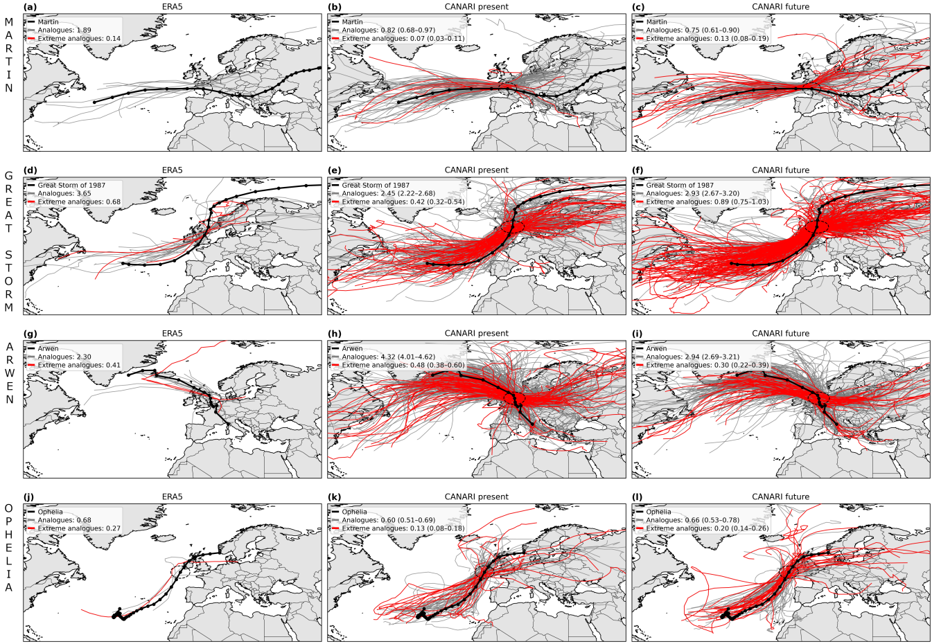
Figure 5. The full track of the case study cyclones (top to bottom) Martin, the Great Storm of 1987, Arwen and Ophelia (black lines) and their analogues (grey lines) from (a,d,g,j) ERA5, (b,e,h,k) the present-day CANARI LE, and (c,f,i,l) the future CANARI LE. Extreme analogues are marked red. The dashed circles indicate the 300 km radius used to identify the position of cyclones at peak intensity. The legends show analogue and extreme analogue rates per decade, with confidence intervals (95%) constructed from a bootstrap resampling of the CANARI LE members.
