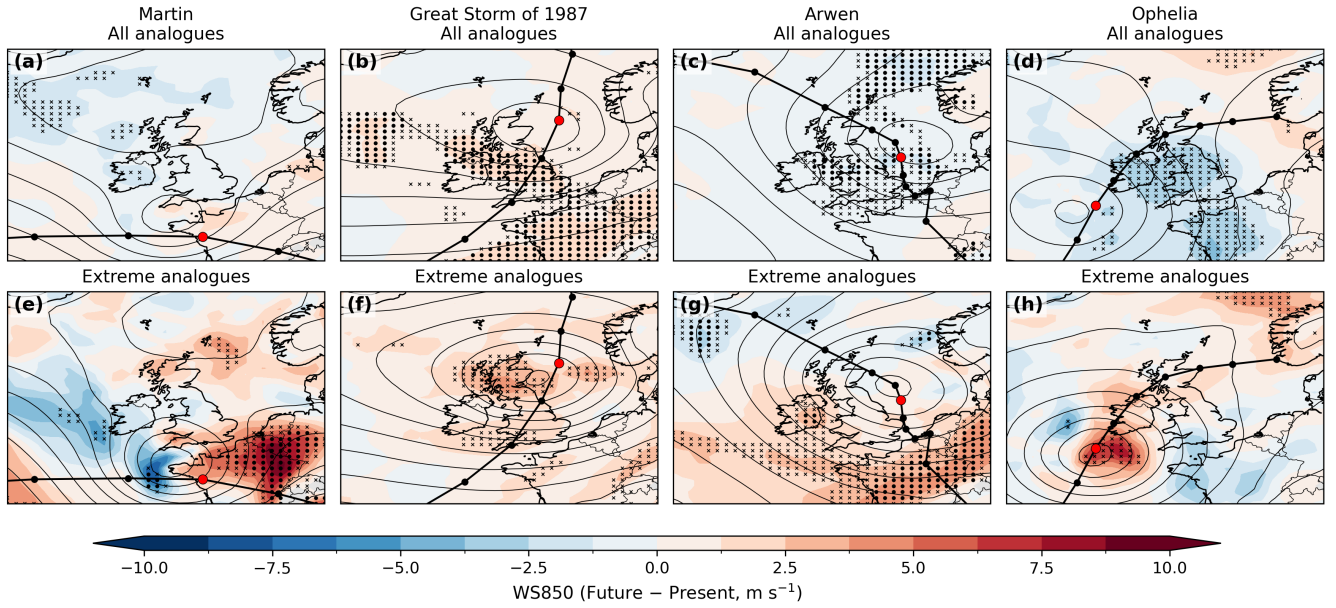
Figure 6. Composite difference plots (CANARI future–present) of wind speed at 850 hPa (shading, \text{m s}^{-1} ) for (a,e) Martin, (b,f) Great Storm of 1987, (c,g) Arwen and (d,h) Ophelia analogues and extreme analogues at their time of maximum intensity. Black contours show the CANARI present composite SLP (intervals of 4 hPa). Stippling denotes significant regions according to the Benjamini-Hochberg false discovery rate procedure (Benjamini and Hochberg, 1995) with \alpha_{\text{FDR}} = 0.10 (Wilks, 2016) while the grid-points marked with crosses indicate local significance at the \alpha = 0.05 level, both based on a Welch’s two-sample t -test. Historical tracks are shown as black lines with the positions of maximum intensity marked by red circles.
