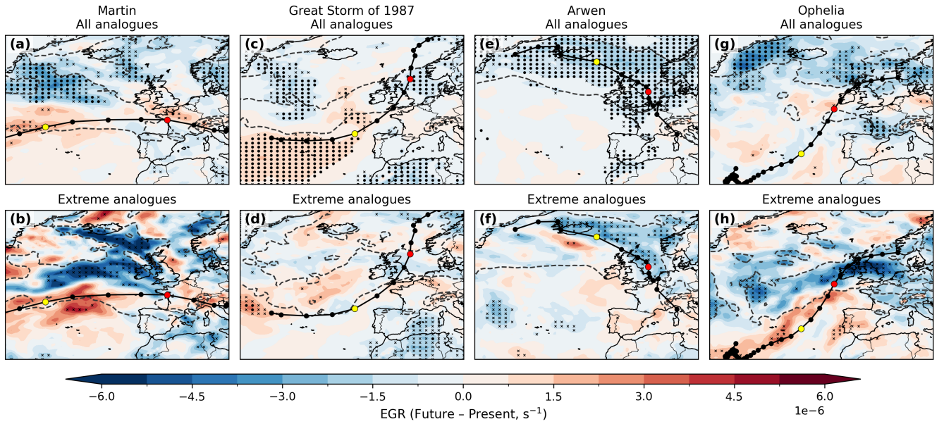
Figure 8. As Fig. 6 but for Eady growth rate (EGR, s -1 ) 24 hours prior to the time of maximum intensity. Dashed contours show the CANARI present composite EGR and yellow circles indicate the track position 24 hours prior to the time of maximum intensity.
