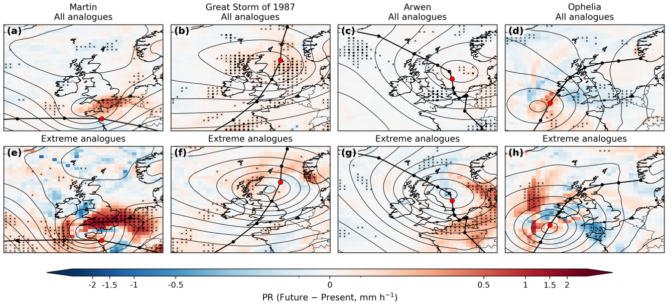
Figure 7. As Fig. 6 but for 6-hour mean precipitation rate (mm hr -1 ) at the time of maximum intensity.
