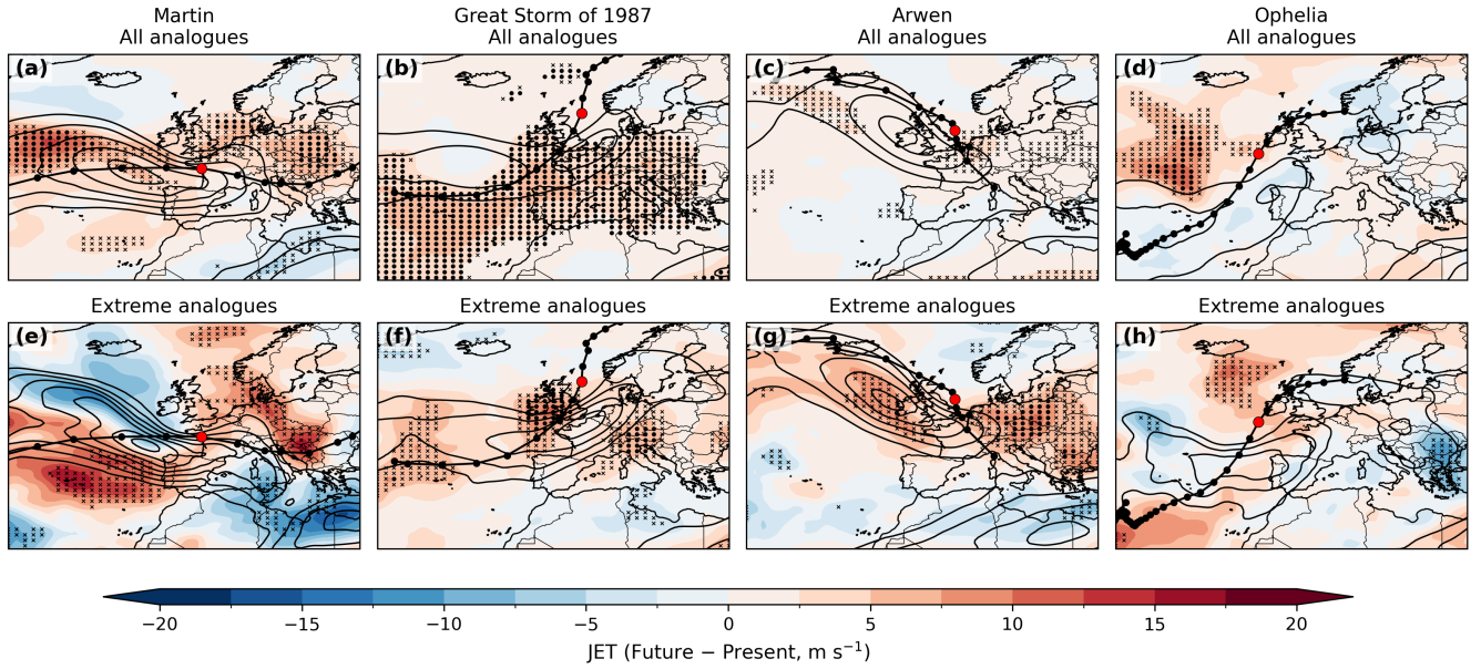
Figure 9. As Fig. 6 but for average wind speed between 400–250 hPa ( \text{m s}^{-1} ) with the CANARI present composite shown by black contours.
