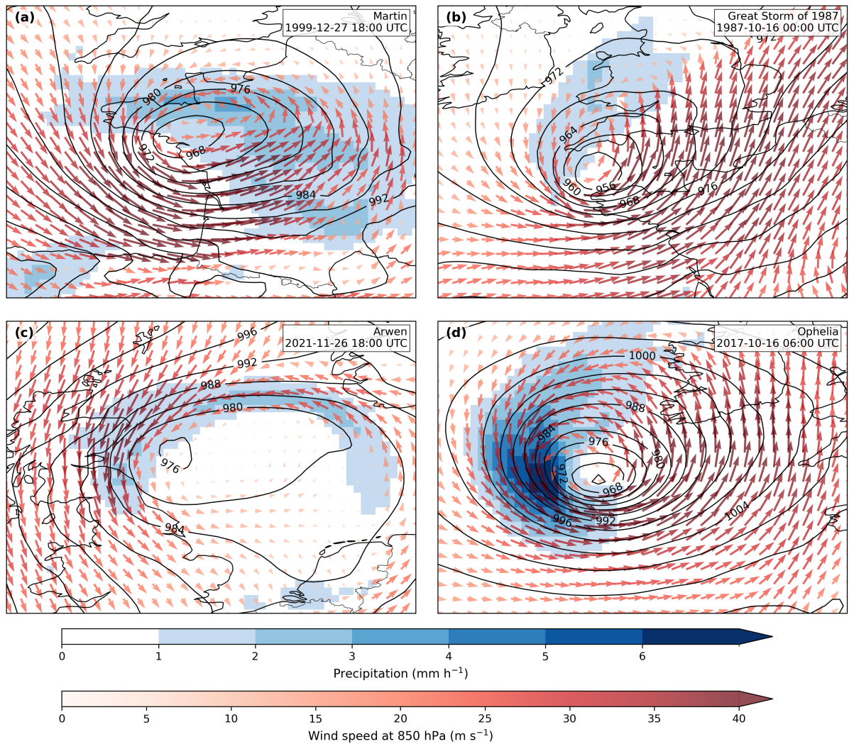
Figure 1. Sea-level pressure (hPa; black contours), 6-hour mean precipitation rate ( \text{mm h}^{-1} ; shading for values \geq 1 \text{ mm h}^{-1} ), and 850-hPa wind ( \text{m s}^{-1} ); coloured wind vectors for (a) Storm Martin, (b) the Great Storm of 1987, (c) Storm Arwen, and (d) cyclone Ophelia from ERA5 reanalysis. The times shown correspond approximately to the hour of peak intensity for each cyclone, as measured by T42 850 hPa relative vorticity.
