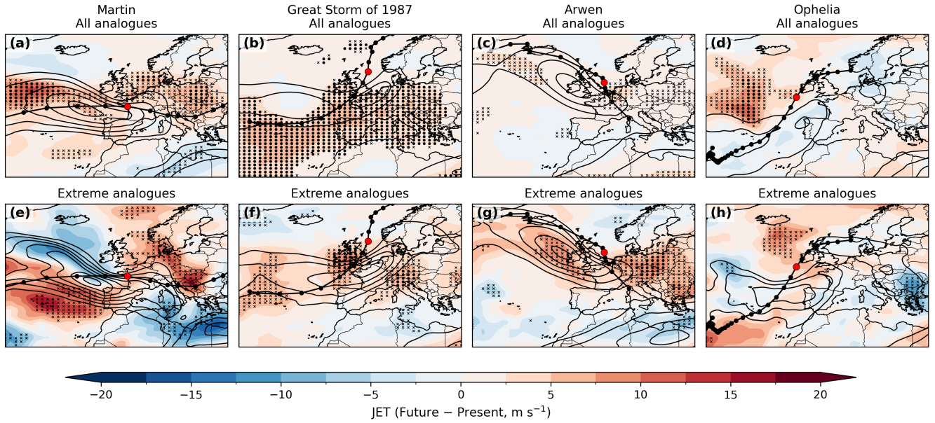
Figure 9. Composite difference plots (CANARI future–present) of As Fig. 6 but for average wind speed between 400–250 hPa ( \text{m s}^{-1} ) for (a,e) Martin, (b,f) Great Storm of 1987, (c,g) Arwen and (d,h) Ophelia analogues and extreme analogues at their time of maximum RV. Black contours show with the present-day CANARI LE present composite field. Shading denotes grid points where differences are non-zero at the 5% significance level based on a Welch’s two-sample t -test and coloured contours show non-significant changes. Historical tracks are shown with by black lines, the position of maximum intensity marked red contours .
