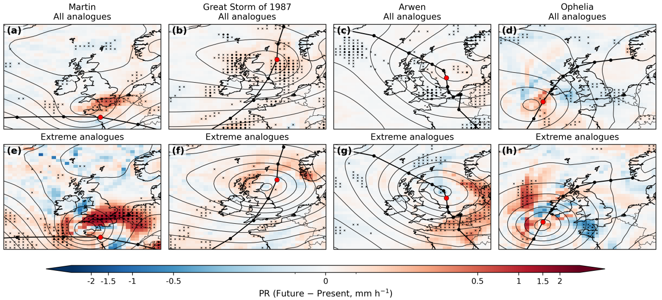
Figure 7. Composite-difference plots (CANARI future–present) of As Fig. 6 but for 6-hour mean precipitation rate ( PR , \text{mm h}^{-1} ) for (a,e) Martin, (b,f) Great Storm of 1987, (c,g) Arwen and (d,h) Ophelia analogues and extreme analogues at their the time of maximum RV intensity . Black contours are taken from the CANARI-LE present SLP composite fields, with intervals of 4 hPa. Shading shows PR differences using a diverging colour scale with a symmetric logarithmic normalisation. Hatching denotes grid points where differences are non-zero at the 5% significance level based on a Welch’s two-sample t -test. Historical tracks shown with black lines, the position of maximum RV (0 h) is marked by a red circle.
