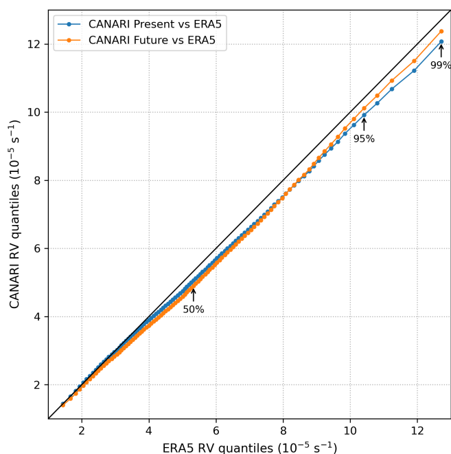
Figure 4. CANARI present and ERA5 Comparison of the distribution of track-maximum relative vorticity quantiles in ERA5 (x-axis; 1980-2010) and the CANARI present (blue; 1980-2010) and future (orange; 2070-2100) for all cyclones that reach peak intensity within the North-Atlantic-European region between the months of September and April displayed in Fig. 3 (60° W–20° E, 30° N–70° N) between the months of September and April.
