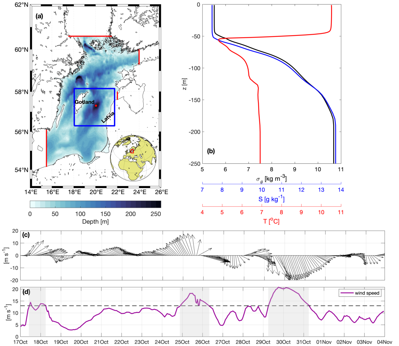
Figure 1. (a) Model domain (central Baltic Sea, known as Baltic Proper) and bathymetry. Red lines indicate the open boundaries of the model, the blue box shows the study area (Eastern Gotland Basin), and the red dot marks the position of the profiles shown in panel (b). (b) Vertical profiles of density, salinity, and temperature at the deepest point of the Eastern Gotland Basin (Gotland Deep) on 29 October 21:00 UTC. (c) Basin-averaged wind speed and direction throughout the study period (October/November 2017). (d) Basin-averaged wind speed magnitude, with the dashed horizontal line indicating the 13 \text{ m s}^{-1} threshold used to define storm events. The light gray shaded areas indicate the approximate duration of the three successive storm events.
