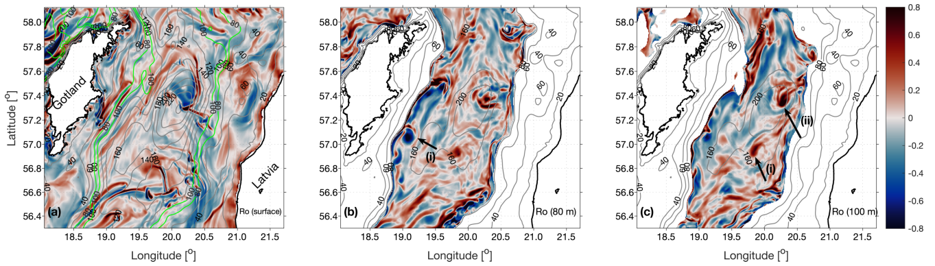
Figure 2. Surface-layer and deep-water submesoscale features. Rossby number (Ro) snapshots (a) in the surface layer (2 m depth), (b) below the main pycnocline (80 m), and (c) in the interior (100 m) of the Eastern Gotland Basin for 31 October 2017 09:00 UTC (storm conditions). The gray contours in all panels show the topography, whereas the green lines in (a) delineate the 80 m and 100 m bathymetry contours. Black arrows indicate eddy-like features.
