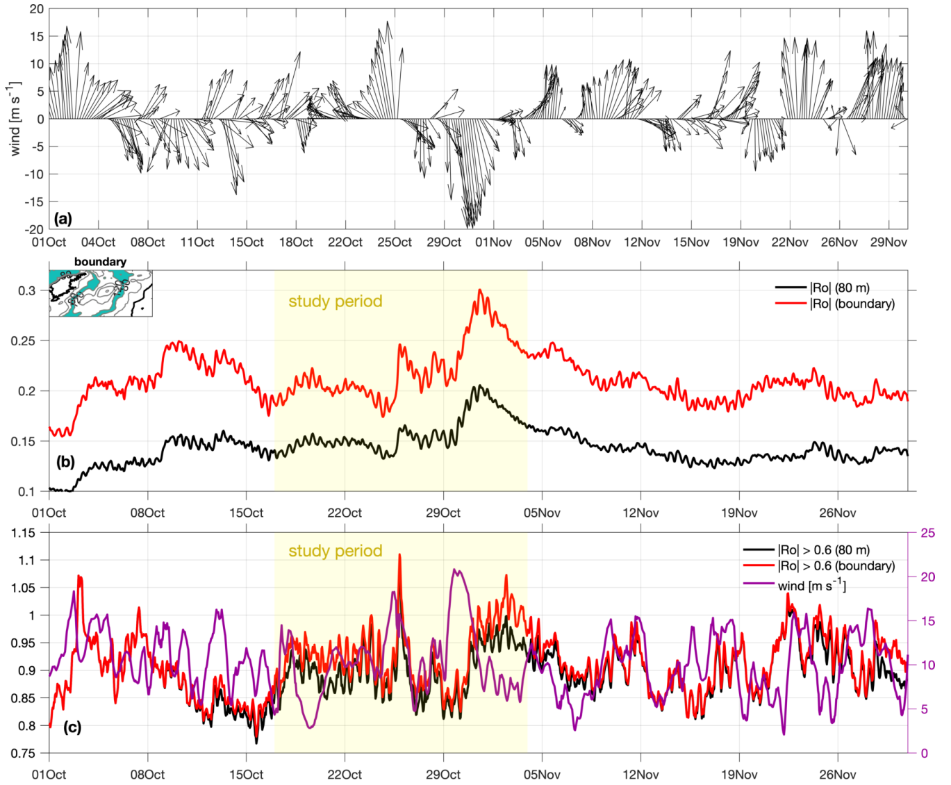
Figure A1. (a) Basin-averaged wind speed and direction, (b) absolute value of \text{Ro} at 80 m depth (black line) and near the lateral boundaries of the basin (red line), defined as the area between 80 m and 120 m depth (green region in the inset panel). (c) Same as before, but for the strong \text{Ro} features (defined as |\text{Ro}| > 0.6 ). The purple line indicates the spatially averaged wind speed. The study period is indicated by the light yellow shaded area.
