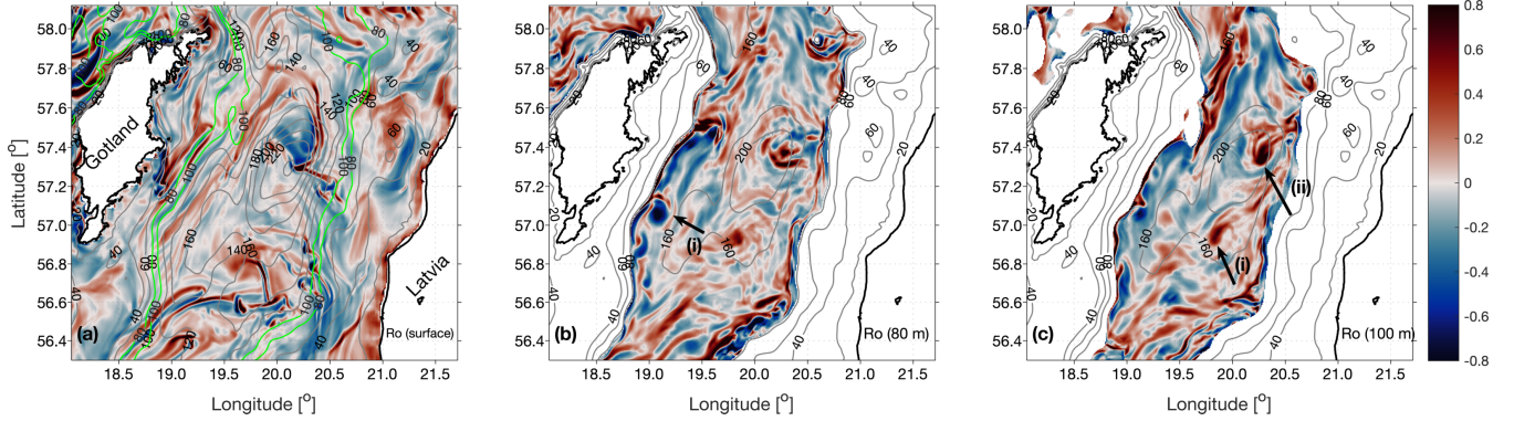
Figure 2. Surface-layer and deep-water submesoscale features. Rossby number ( Ro ) snapshots (a) in the surface layer (2 m depth), (b) below the main pycnocline (80 m), and (c) in the interior (100 m) of the Eastern Gotland Basin for 31 October 2017 09:00 UTC (storm conditions). The gray contours in all panels show the topography, whereas the green lines in (a) delineate the 80 m and 100 m bathymetry contours. Black arrows indicate eddy-like features.
