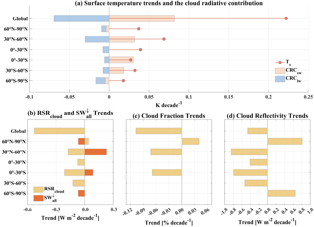
Figure 1. (a) ERA5 T_s trends from July 2002 to February 2023 and the T_s trends caused by changes in surface shortwave and longwave cloud radiative forcing ( CRC_{sw} and CRC_{lw} ) (methodology detailed in Section 2.3). (b) Global and latitude-zone averaged trends in the all-sky surface downward shortwave radiation fluxes ( SW_{all}^{\downarrow} ) and the cloud component of TOA RSR ( RSR_{cloud} ), (c) CF, and (d) CR. Note that the latitudinal-mean trends in (a)-(c) are weighted by their area to account for their contributions to the global mean; the sum of the zonal trends approximately equals the global trend. Only trends significant at the 95% confidence level are shown.
