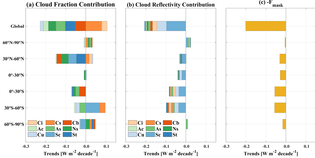
Figure 4. The trends in domain-averaged RSR_{cloud} caused by the changes in (a) CF and (b) CR across nine cloud types, and (c) the cloud masking effect ( -\Delta F_{mask} ), at global and latitudinal scales, sorted in descending order of magnitude. Note that the latitudinal-mean trends are weighted by their area to account for their contributions to the global mean; the sum of the zonal trends approximately equals the global trend. Only trends significant at the 95% confidence level are shown.
