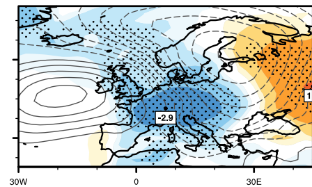
ModE-RAClim
