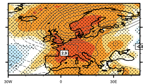
ModE-RAClim
