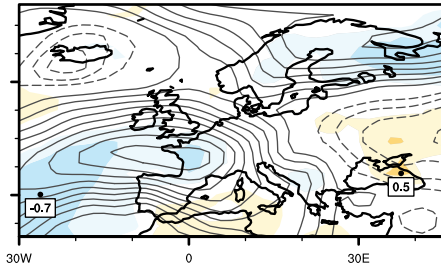
ModE-Sim
