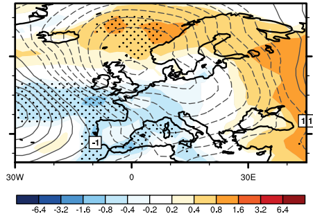
ModE-Sim
