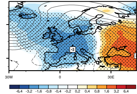
ModE-RAClim
