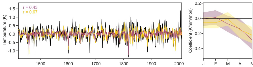
Figure 6. Time series of JJA 2 m temperatures in the land area between 8° W and 38° E, 36-48° N in ModE-RA (black) and predicted from the regression models based on spring-only predictors (purple) and spring-summer predictors (orange). Right: Coefficients (95% confidence intervals shaded) for precipitation in January to May in the two models.
