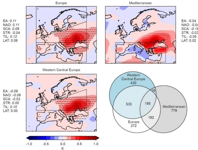
Figure 4. Composites of ModE-RA JJA 2m temperature anomalies for all years and ensemble members with JFMAM precipitation <10 th percentile in Europe, MED, and WCE. Stippling indicates 2m temperature anomalies exceeding two standard deviations. The averages of the six circulation indices, here standardised for better intercomparison are also indicated ( p < 0.05 in italics). The lower right shows an Euler diagram of the number of the cases.
