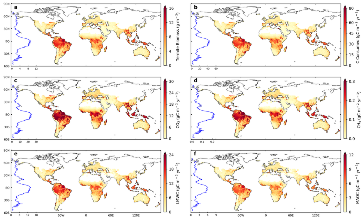
Figure 2. Spatial distribution of termite-driven carbon pools. a , Termite biomass. b , Carbon consumed. c , CO_2 emissions. d , Net CH_4 emissions. e , LMWC flux. f , MAOC flux. The inset in each plot (blue line) shows the latitudinal mean of the corresponding variable, using the same units as the associated colorbar.
