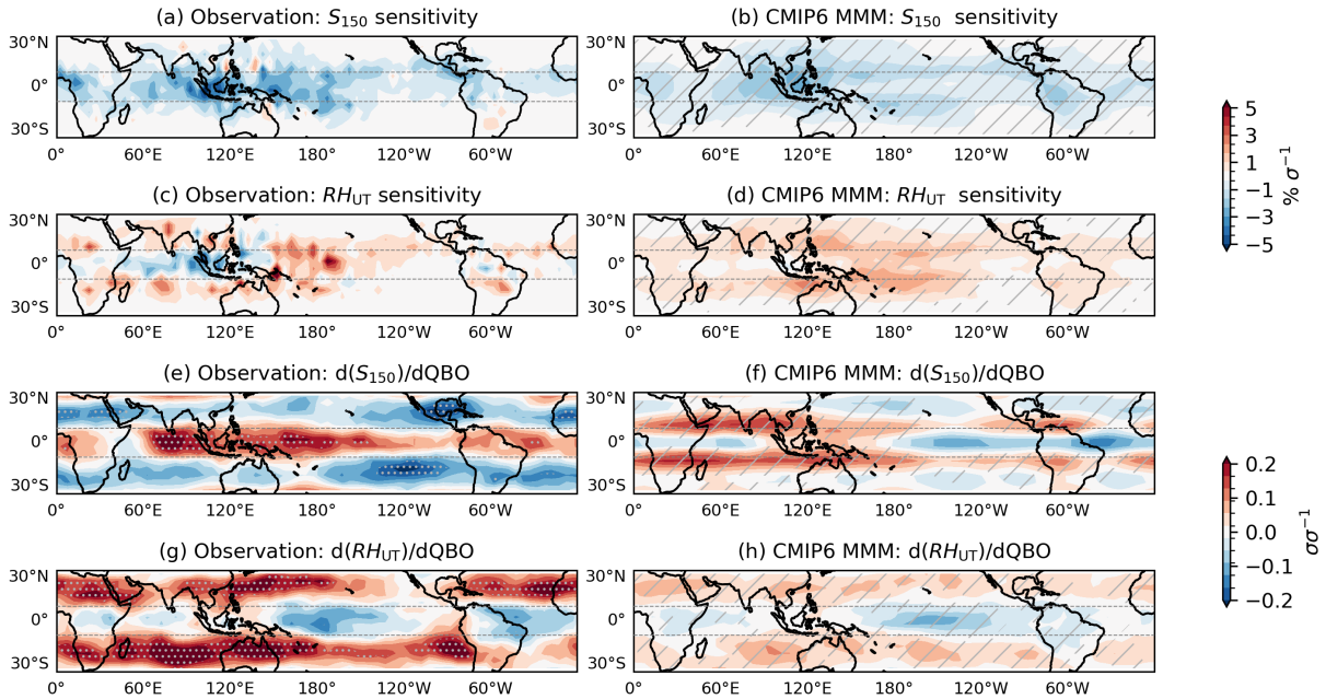
Figure 4: Historically derived sensitivities of the TTL cloud fraction to static stability at 150 hPa ( S_{150} ) and upper tropospheric 425 relative humidity ( RH_{UT} ) in observations (a, c) and the CMIP6 MMM (b, d). QBO-regressed S_{150} and RH_{UT} respectively, in units of standard deviation of CCF per standard deviation of QBO, in observations (e, g) and the CMIP6 MMM (f, h). Stippling in (e, g) marks statistically significant results (99% confidence). Hatching in the right column denotes regions where six out of seven models agree on the sign.
