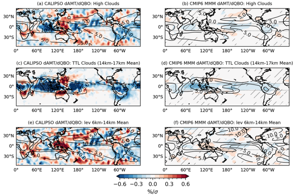
Figure 2: QBO regressed high-cloud fraction (<440 hPa), TTL cloud fraction (<180 hPa), and 440–180 hPa cloud fraction in CALIPSO (a, c, e) and CMIP6 MMM (b, d, f), represented in units of standard deviation of the QBO index. Overlaid line contours indicate the climatology of respective cloud fraction. Stippling in (a, c, e) denotes 90% confidence, and hatching in (b, d, f) denotes six out of 7 models having the same sign.
