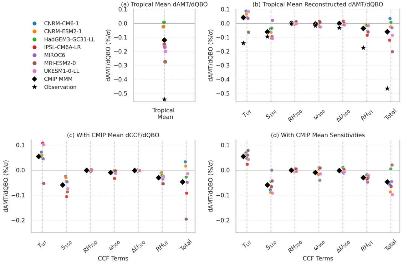
Figure 5: (a) Tropical mean (10S–10N) of QBO-regressed TTL cloud fraction in observations, CMIP6 models and the MMM. (b) Individual CCF contributions to the tropical-mean QBO-induced TTL cloud response and the total. (c) Same as (b) but replacing model-specific QBO-regressed CCF anomalies with the MMM CCF responses. (d) Same as (b) but replacing model-specific cloud sensitivities with the CMIP6 MMM sensitivities. Changes are per unit standard deviation of QBO.
