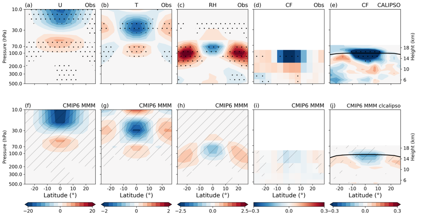
Figure 1: Latitude–height sections of QBO-regressed (a) zonal-mean zonal wind, (b) temperature, (c) relative humidity from ERA-5, (d) cloud fraction from MODIS and (e) CALIPSO between \pm 30^\circ latitude. (f–j) Similarly for the CMIP6 multi-model mean, with (i) ISCCP-simulated cloud fraction and (j) CALIPSO-simulated cloud fraction. Panels are shown on pressure levels, except for panels (d) and (i), which use a bin-based representation defined by cloud top pressure, and for visualisation, the uppermost bin is limited to 90 hPa. Stippling marks statistically significant results in the top row (95% confidence; 90% for cloud fraction). Hatching denotes regions where six out of seven models agree on the sign. In panels (e) and (j), the black line denotes the mean tropopause pressure level.
