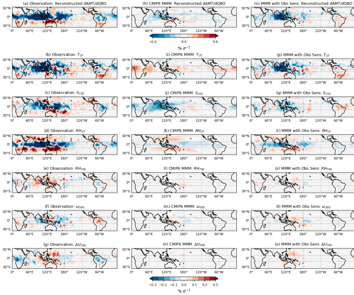
375 Figure 3: Reconstruction of QBO-regressed TTL cloud fraction anomalies using CCF analysis for (a) observations and (h) the 380 CMIP6 MMM. (b-g) Contribution of each CCF to the observed QBO–TTL cloud relationship and (i-n) to the CMIP6 MMM QBO– TTL cloud relationship. (p-u) QBO-regressed CCFs from the CMIP6 MMM convolved with observed cloud sensitivities and (o) their sum.
