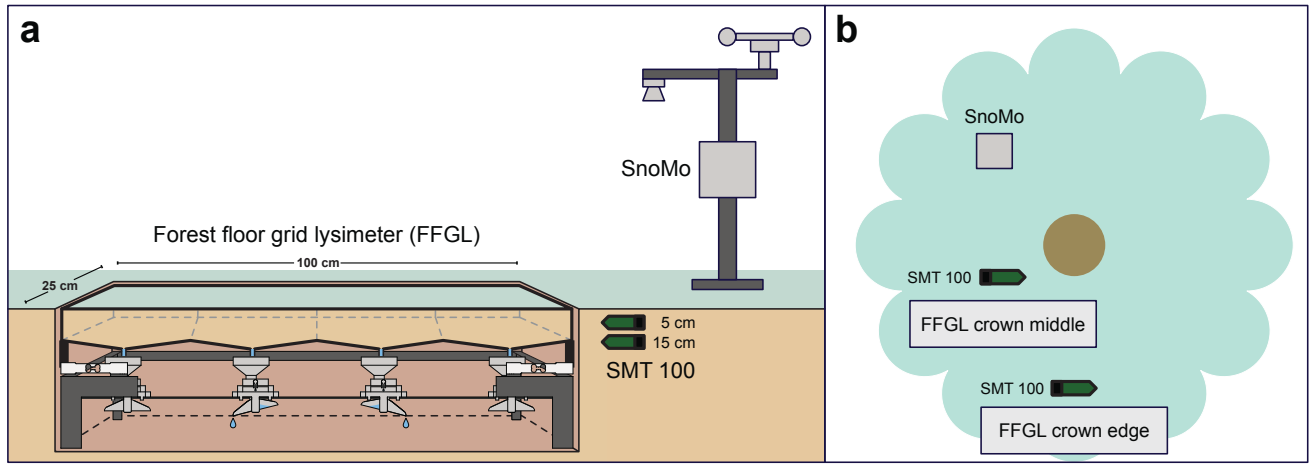
110 Figure 1: Installed setup (a) containing a microclimate station (SnoMo), soil moisture probes (SMT100) and forest floor grid 115 lysimeters (FFGL), and (b) the corresponding positioning to the tree.
