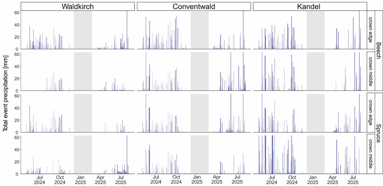
205 Figure 4: Identified rainfall events and their total Throughfall ( P_{TF} ) for all twelve lysimeters, the snow-affected period which was excluded from the statistical analysis is rendered in grey.
