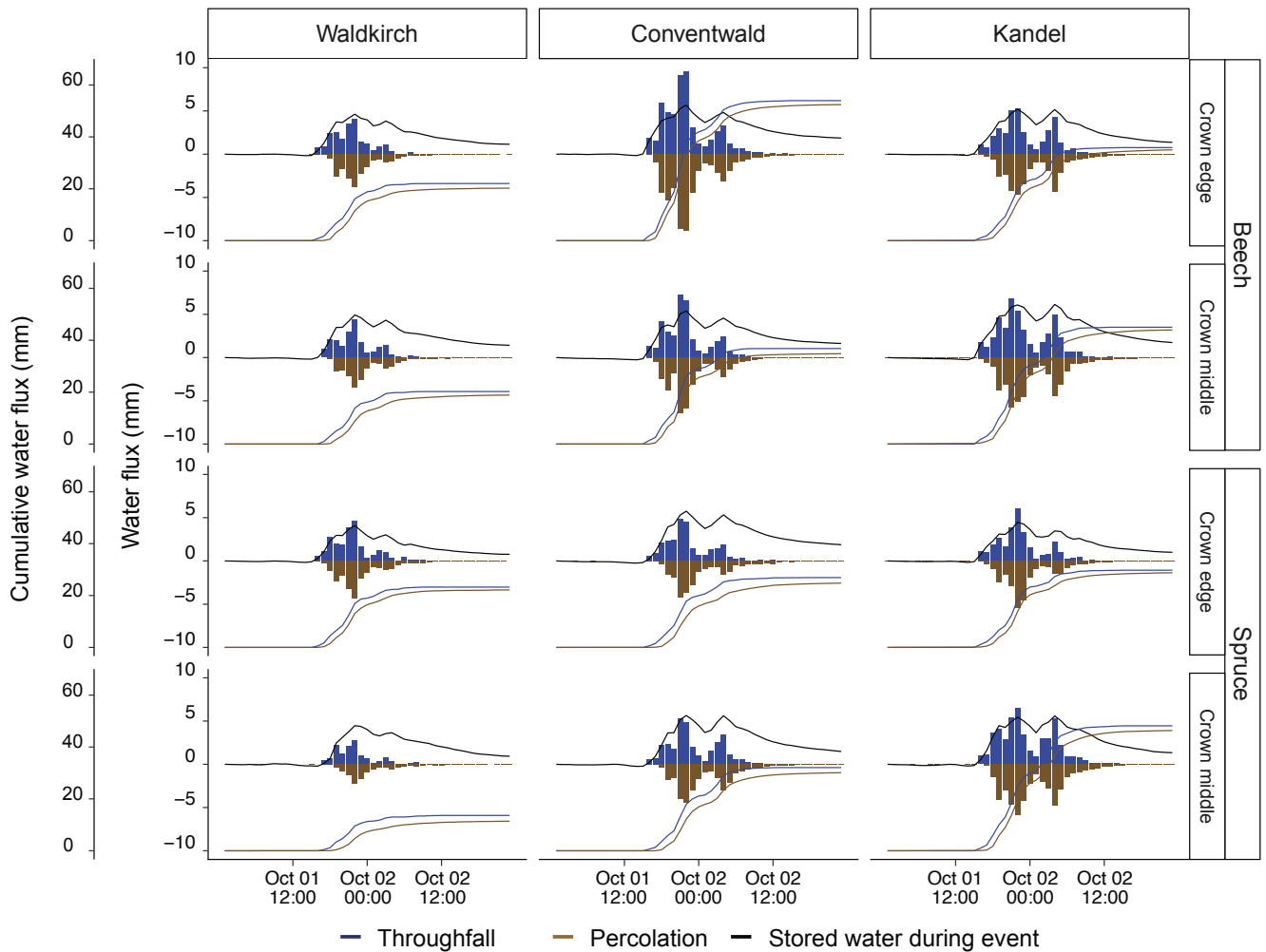
Figure 3: Total and cumulative hourly water fluxes of precipitation and percolation, as well as amount of additionally stored water during the event for a selected rainfall event in fall 2024 (1.10.2024).
