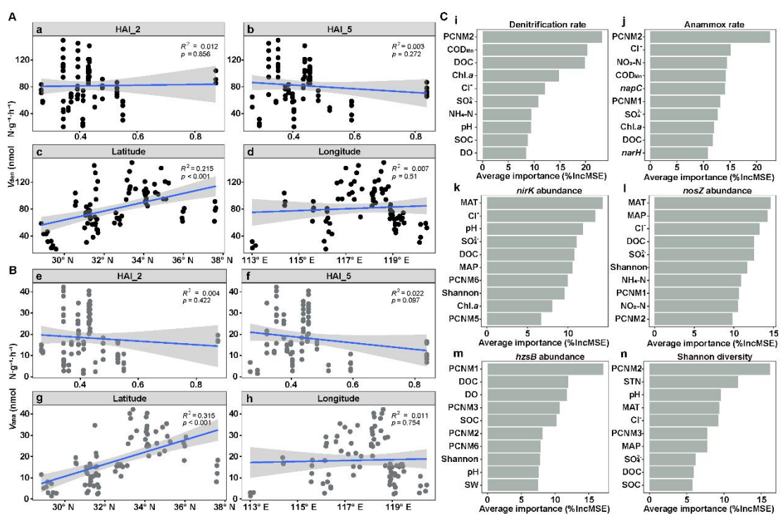
Figure 5 Drivers of nitrogen removal processes in the Eastern China Plain lakes. Linear regressions of denitrification (A) and anammox (B) rates against Human Activity Intensity (HAI)
