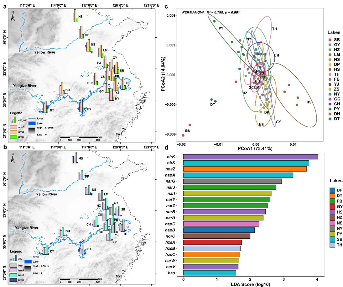
Figure 3 Spatial distribution of functional genes associated with sediment denitrification (a) and anammox (b) in the Eastern China Plain lakes. (c) Beta-diversity of functional gene profiles visualized via Principal Coordinates Analysis (PCoA). (d) Linear Discriminant Analysis Effect Size (LEfSe) identifying discriminative functional genes between groups. Beta-diversity elucidated the spatial patterns of the nitrogen removal functional gene (Fig. 3c). Sampling sites overlapped extensively in the two-dimensional ordination space, with the first principal coordinate axis (PCoA1) explaining the majority of the variance (73.41%). However,
