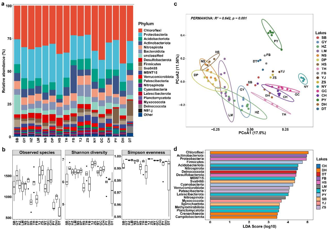
Figure 4 Sediment microbial community characteristics in the Eastern China Plain lakes. (a) Taxonomic composition of the top 20 phyla. (b) Alpha-diversity indices, where "Observed species" denotes the number of observed amplicon sequence variants (ASVs). (c) Microbial beta-diversity based on PCoA. (d) LEfSe analysis identifying discriminative taxa at the phylum level between groups.
