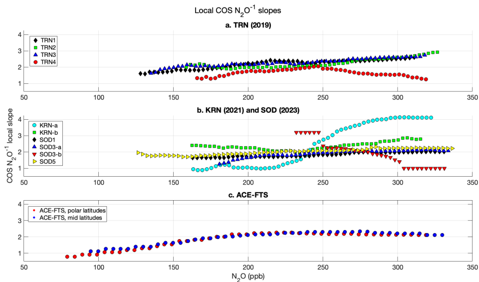
305 Figure 4: Local COS N 2 O -1 slopes (ppt ppb -1 ) obtained from AirCore and ACE-FTS profiles.
