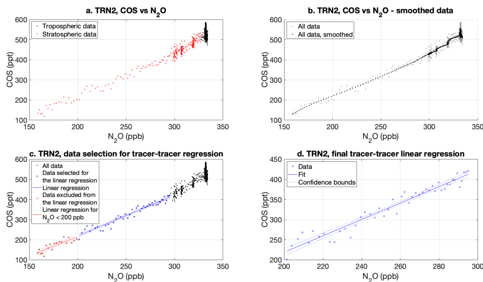
Figure 2: Data selection steps for the linear regression between COS and N 2 O, exemplified with the TRN2 AirCore data.
