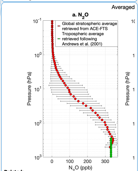
Deleted: Figure 4: the average global profiles used to calculate the global average burdens for 2019. The red dots represent globally averaged ACE-FTS data, while the green dots are the tropospheric averages retrieved following Andrews et al. (2001). Where both data are present, only the averages retrieved with Andrews et al. (2001) method were considered.
