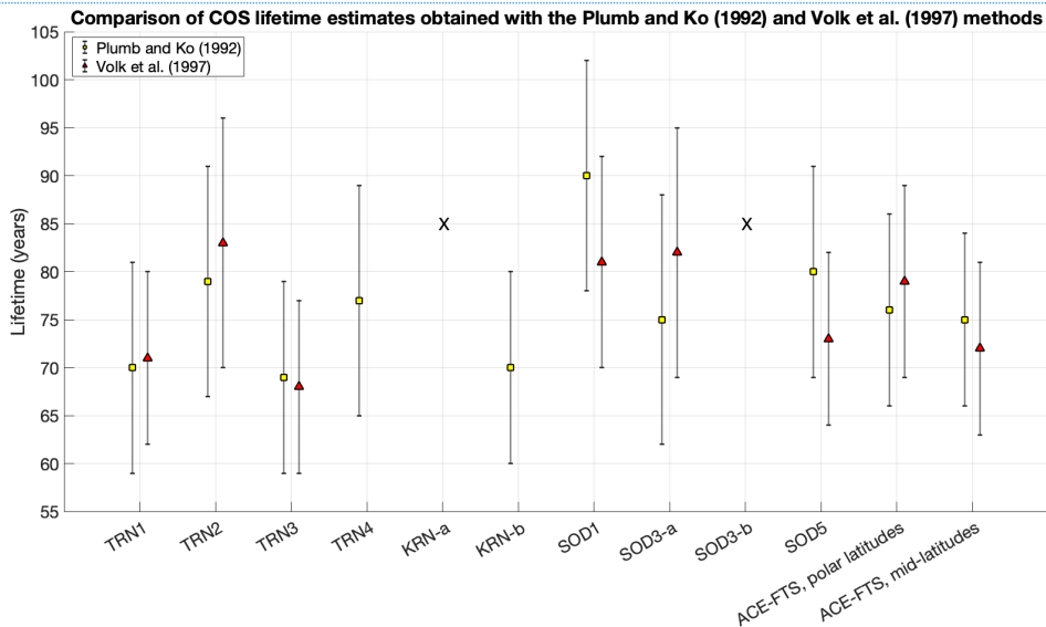
395 Figure 6: calculated COS lifetime for AirCore samples and ACE-FTS observations obtained following the two methodologies. Datasets for which it was not possible to apply any of the two methods reliably are signaled by an “X”.
