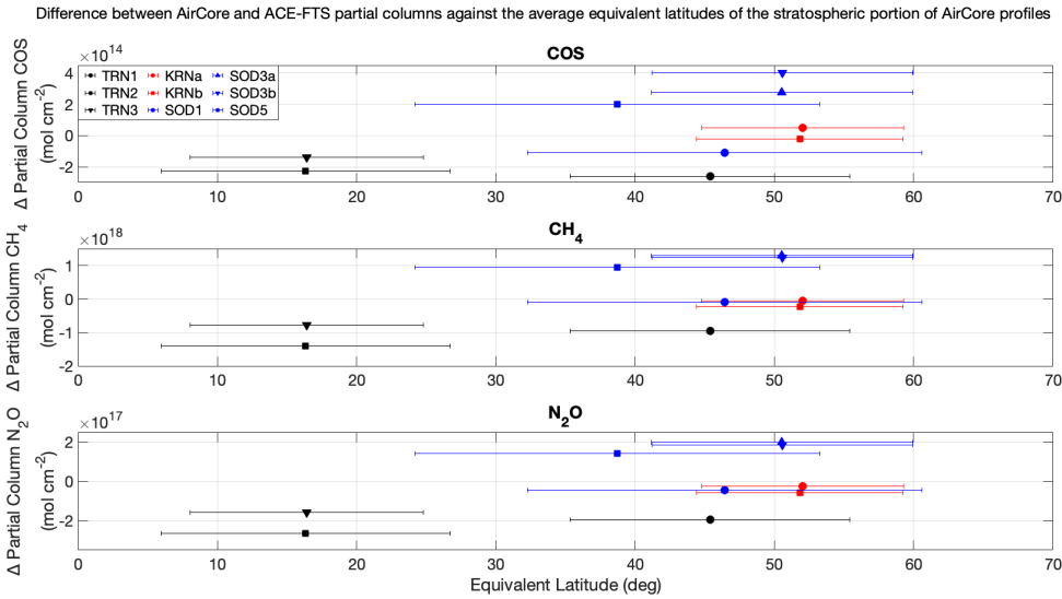
Figure 9: retrieved differences between stratospheric partial columns of AirCore and ACE-FTS profiles, against the average stratospheric equivalent latitude of AirCore profiles. The partial columns are reported in molecules cm -2 .
