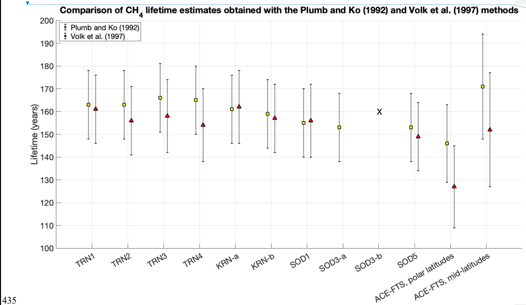
Figure 7: calculated CH 4 lifetime for AirCore samples and ACE-FTS observations obtained following the methods of Plumb and Ko (1992) and Volk et al. (1997). The missing estimates for SOD3-b are marked as an “X”.
