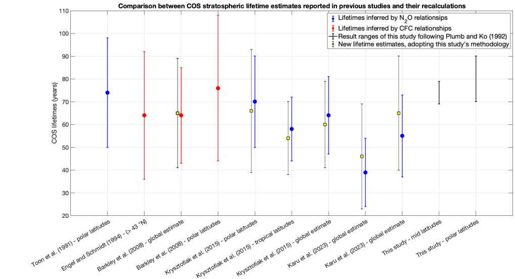
Figure 8: comparison between COS lifetime estimates of previous studies with their recalculations with new tropospheric burdens obtained following the methods of this study (based on Andrews et al., 2001), in chronological order. The ranges reported for this study correspond to the Plumb and Ko (1992) method, which was also adopted in the studies presented in this figure.
