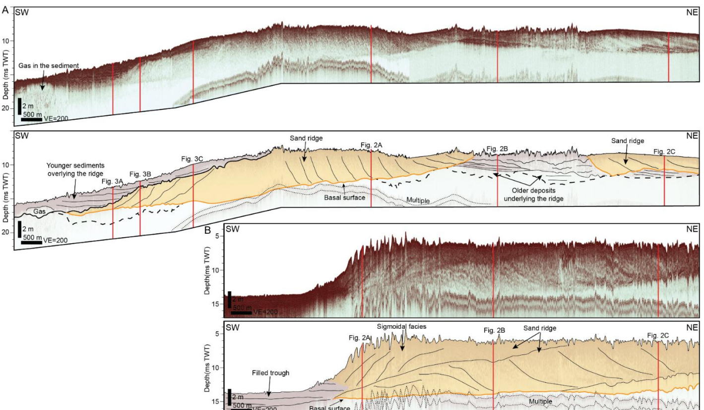
Figure 4. High-resolution acoustic profiles generated by merging multiple lines along the Stroombank sand ridge (SW to NE), displayed from offshore to onshore (A–B). Profile locations are shown in Fig. 1C, and corresponding sediment cores are presented in Fig. 6.
