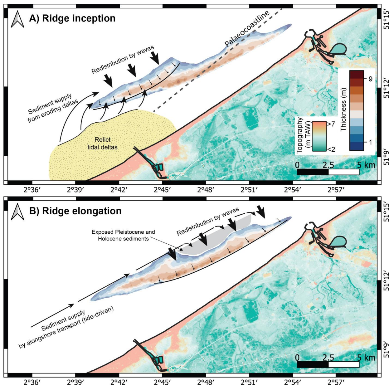
Figure 8. Conceptual model for the formation of the Stroombank sand ridge using the sediment thickness map of Fig. 5B. A) Ridge inception: the initial accumulation of sand was fuelled by sediment supplied from the erosion of relict tidal-delta deposits associated with a waning tidal-inlet system southwest of the Stroombank. This sediment was reworked and redistributed along the incipient ridge by wave-driven cross-shore transport. The palaeocoastline is based on the reconstructions of Cartelle et al. (2025, 2026) for the Late Holocene and represents a minimum seaward position. B) Ridge elongation: once the ebb-tidal-delta sediment source became buried, ridge development was maintained primarily by tide-driven alongshore sediment transport supplying sand from the southwest, and by wave-driven reworking that redistributed sediment across the ridge. Background topographic data were provided by Nationaal Geografisch Instituut and are available at www.geo.be .
