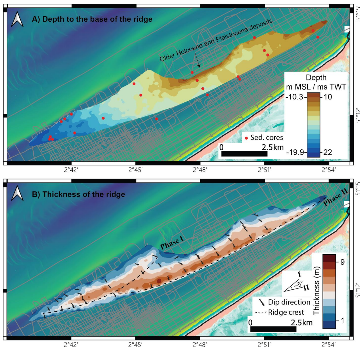
Figure 5. (A) Map of the depth to the basal disconformity underlying the Stroombank sand-ridge deposits. (B) Thickness map of the sedimentary body forming the Stroombank sand ridge. Phases I and II represent two stages of the ridge development, with phase I mostly buried and phase II corresponding to the present-day Stroombank ridge. Background bathymetric data were provided by Agentschap Maritieme Dienstverlening en Kust and are available at www.agentschapmdk.be . Topographic data were provided by Nationaal Geografisch Instituut and are available at www.geo.be .
