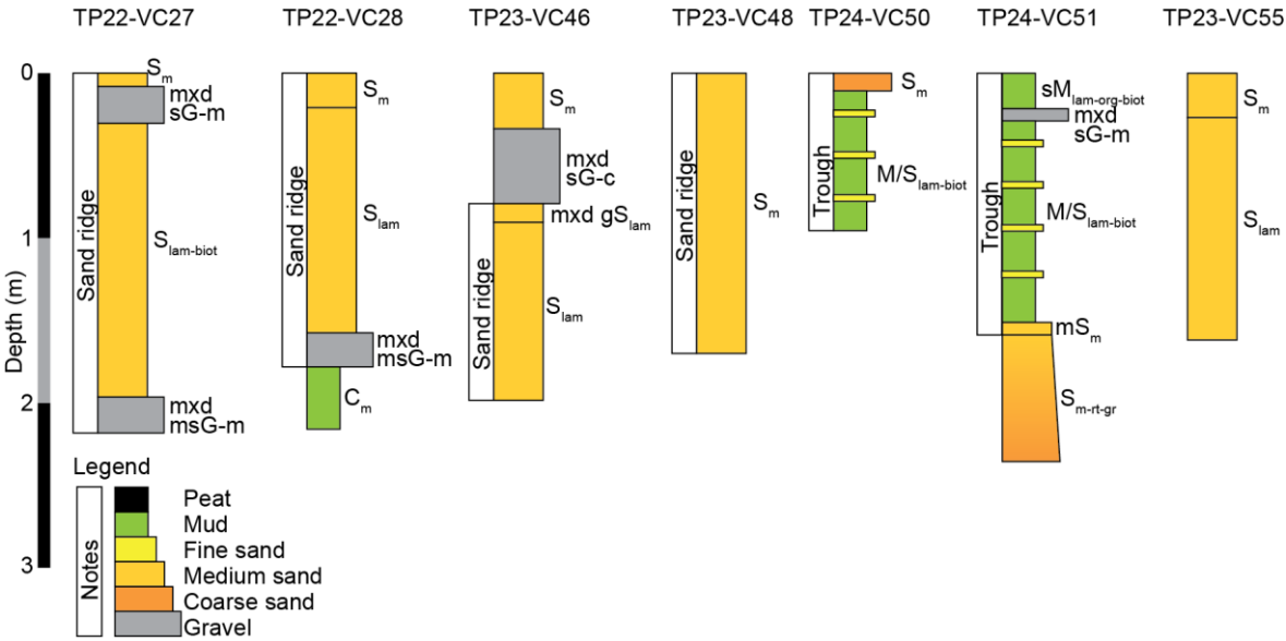
Figure A1. Core logs of sediment cores included in the study but not displayed in the main figures. Location is shown in Fig. 1C and sedimentary facies defined in Table A2.
