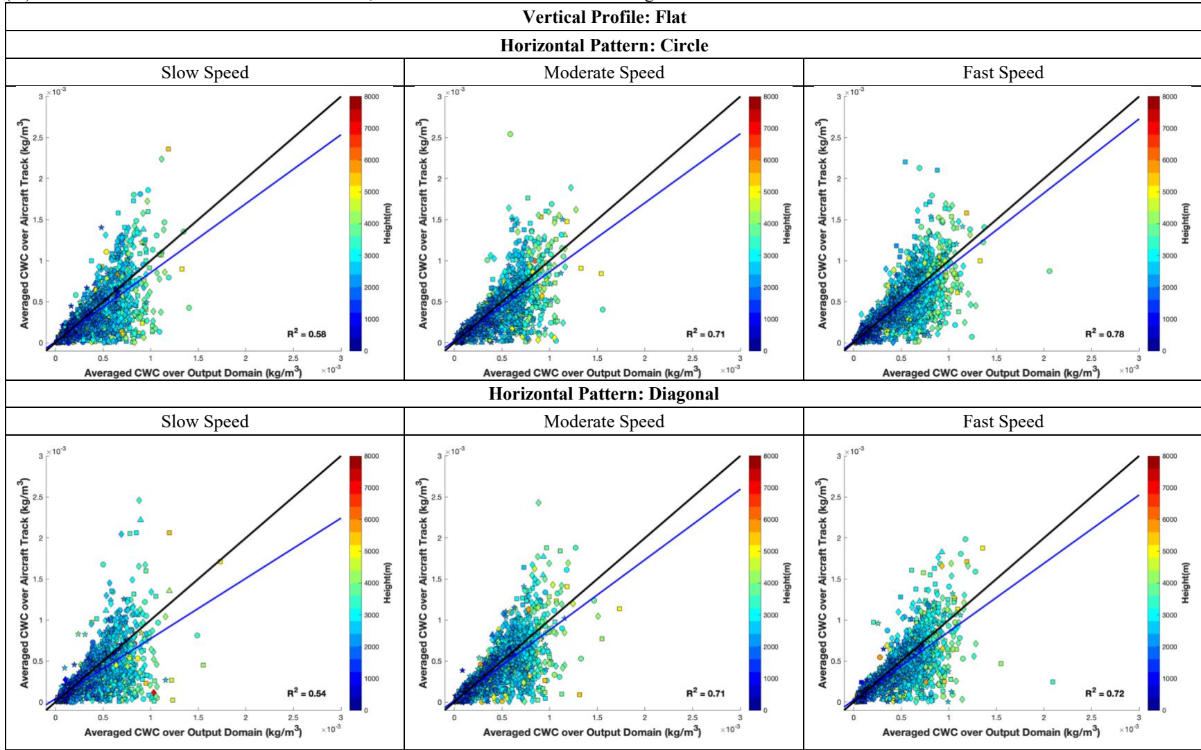
Figure S1. Scatter plots comparing aircraft-sampled and domain-averaged cloud water content (CWC) for all horizontal patterns, vertical profiles, and flight speed categories. The x-axis shows domain-mean CWC over sampled layers, and the y-axis shows trajectory-averaged CWC. Colors indicate sampling height (m). The black line denotes the 1:1 reference line, and the blue line shows the linear regression fit.
