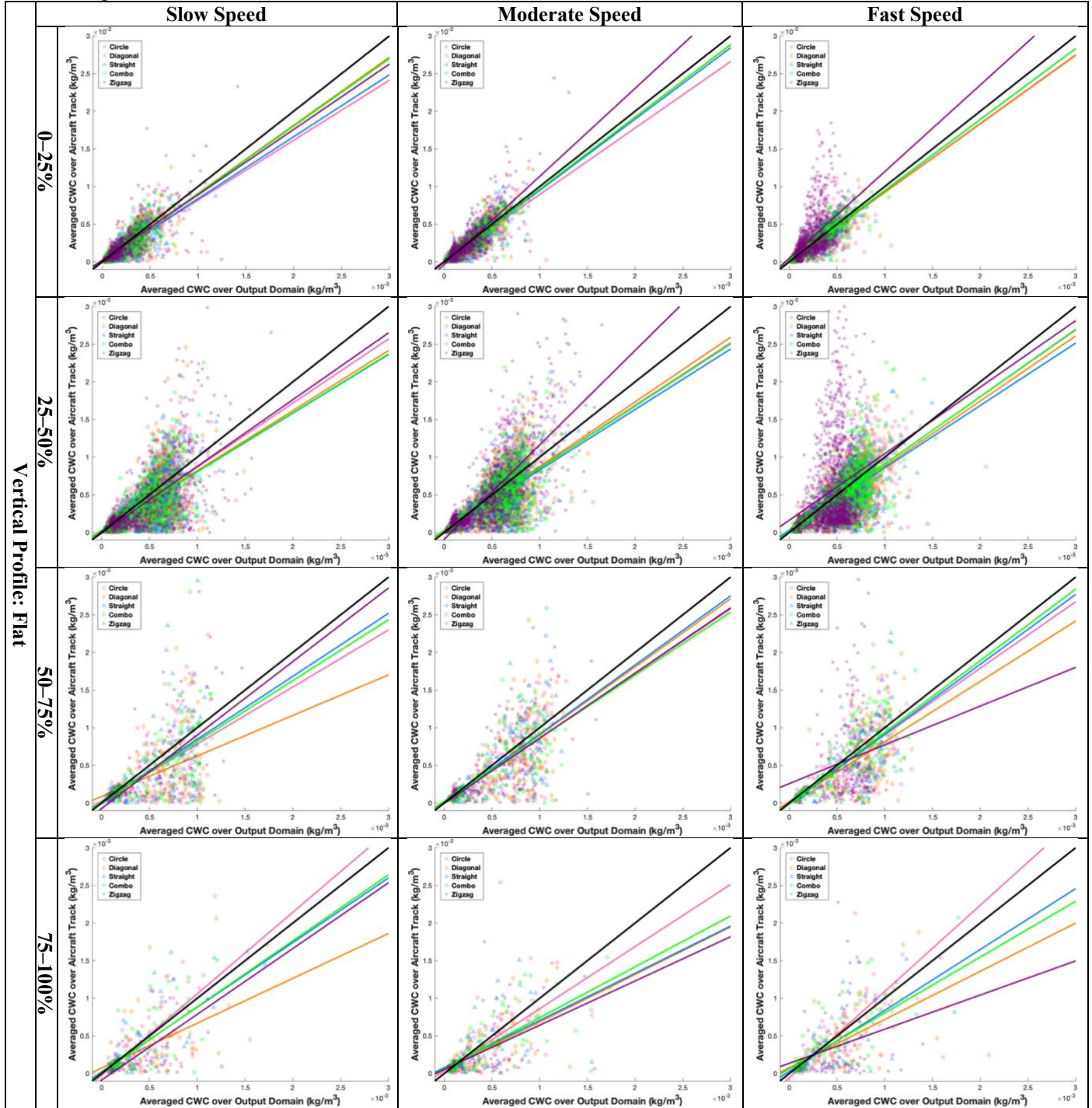
Figure S2. Scatter plots comparing aircraft-sampled and domain-averaged CWC for cases grouped by cloud fraction (CF) categories. The x-axis shows domain-mean CWC over the vertical layers intersected by the aircraft trajectory, and the y-axis shows trajectory-averaged CWC. Colors and symbols indicate different horizontal sampling patterns, and the black line denotes the 1:1 reference line. The zigzag pattern is plotted together for comparison but represents an independent trajectory type rather than the horizontal-vertical combination. The plotting method follows that used in Fig. S1.
