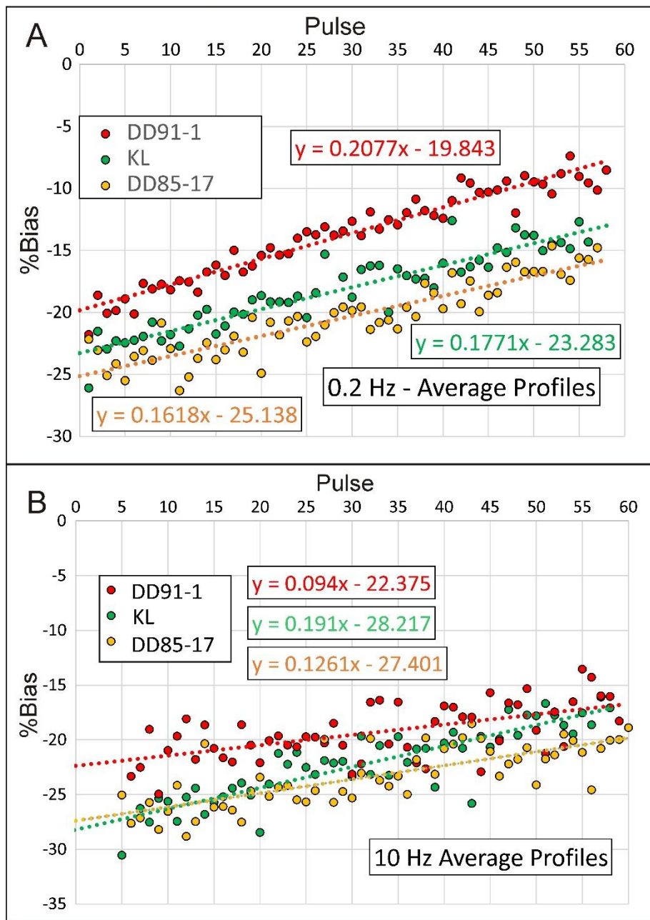
Fig. 10 Percent difference between the measured and true ^{206}\text{Pb}/^{238}\text{U} ratios of three zircon standards for data acquired at (A) 0.2 Hz and (B) 10 Hz. Each set of symbols represents an average of analyses on 4 spots. Analyses shown in A and B were carried out during different sessions with different instrument bias.
