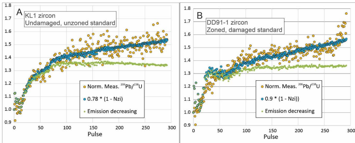
Fig 7: Signal profiles for 0.2 Hz analysis on standards KL (A) and DD91-1 (B). ^{206}\text{Pb}/^{238}\text{U} profiles (orange circles) normalized to estimates of instrument-biased true values compared to profiles of ablation deposits scaled by Pb depletion values chosen to maximize fit to ratio profiles (blue circles). Green dots are the same profiles assuming that ablated mass is proportional to area of the base of the pit with a final aspect ratio of 0.8
