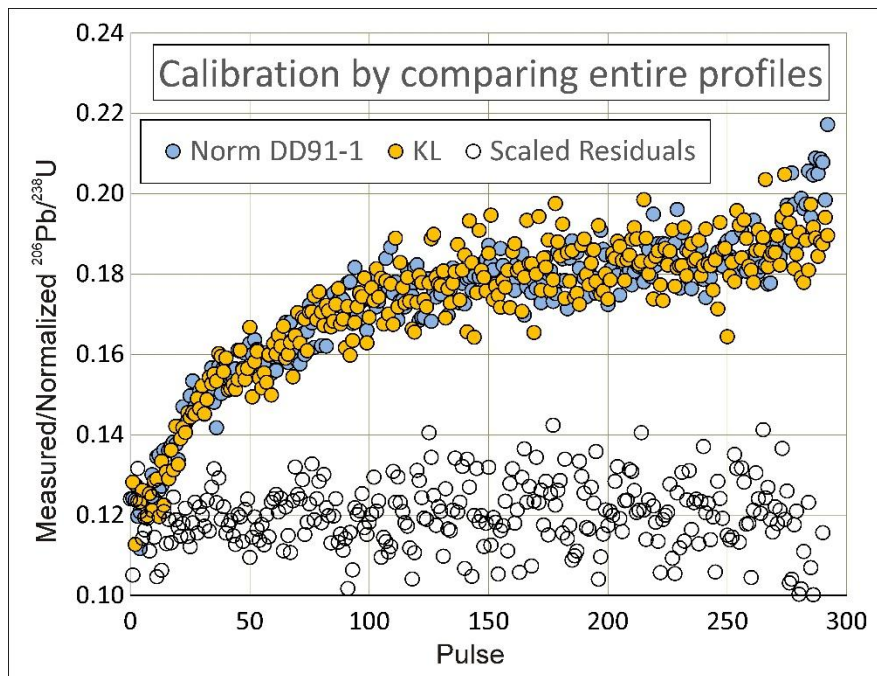
555 Fig 11: Comparison of measured KL ratio profile (taken as the standard) with measured DD91-1 profile (taken as the unknown) normalized to minimize the sum of squares of differences between corresponding data points (residuals). These are scaled so they are visible on the plot. The residual for two overlapping data would plot on the 0.12 line. Omitting the last 30 data, a normalization factor of 2.868 gives the minimum sum of residuals. The inferred ^{206}\text{Pb}/^{238}\text{U} value is 0.15% different from the accepted ratio.
