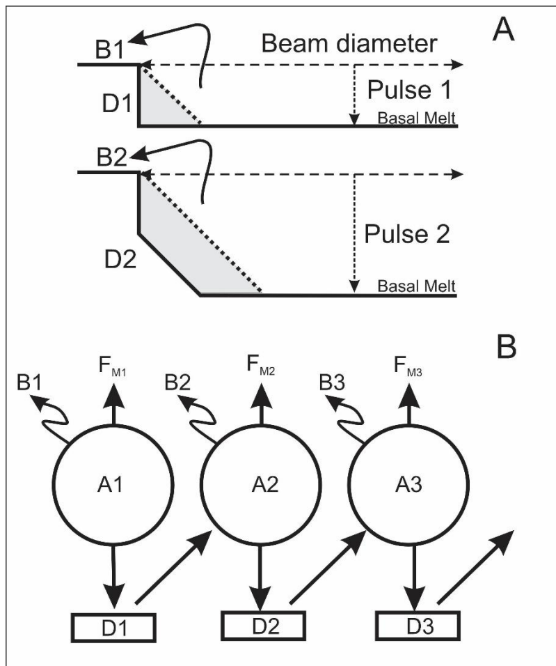
310 Fig. 4 (A) Schematic illustration of the model showing the effect of the first two laser pulses on a zircon sample as seen from the edge of a cross section of an ablation pit. D is the depth excavated per laser pulse. Pb-depleted ablated material (melt) deposited in the pit is shown in grey. The second pulse is assumed to re-ablate the residue left from the first but this consumes energy at the edge of the beam, causing the pit to taper with depth. (B) Effects of the first laser pulses on measured composition. The first ablation cloud (A1) 315 leaves a Pb-depleted deposit in the pit (D1) and fallback (B1), which increases its Pb/U ratio. The second pulse can re-evaporate D1 plus pristine material, leaving a second Pb-depleted deposit (D2) as well as
